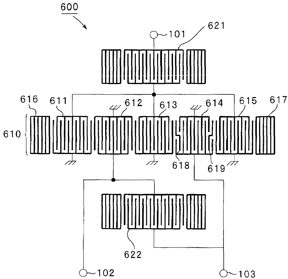
FIG. 19 Prior Art
