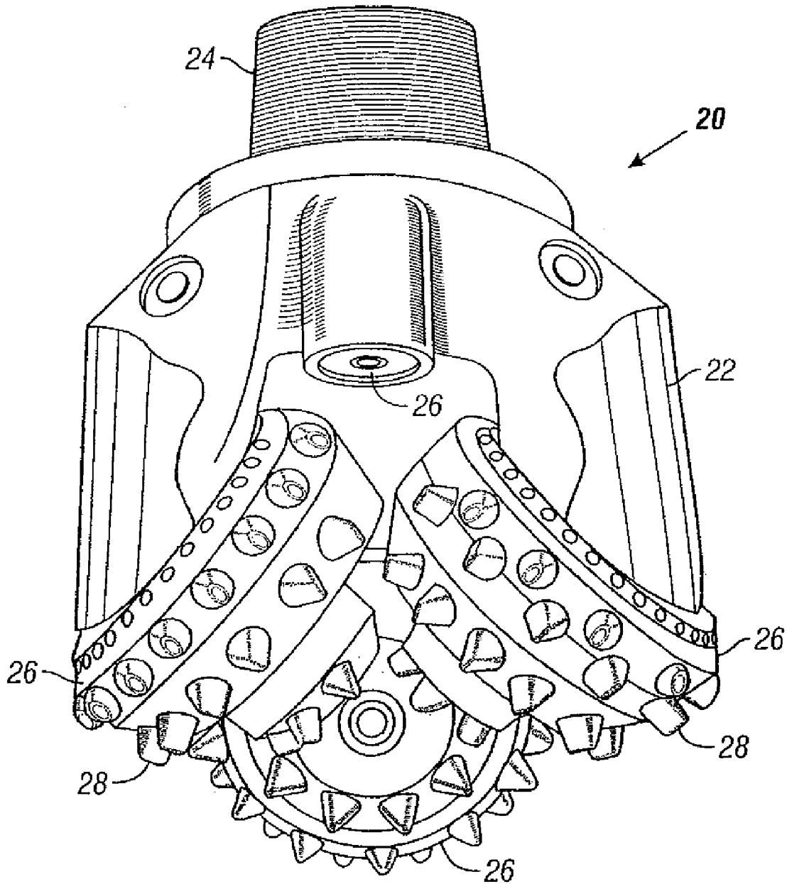
FIG. 1 (Prior Art)
