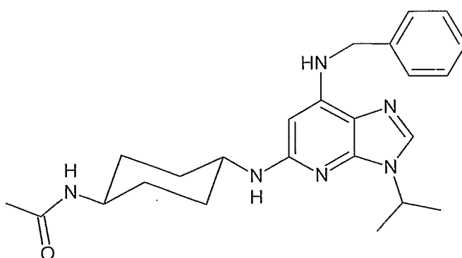
Formula 1h
