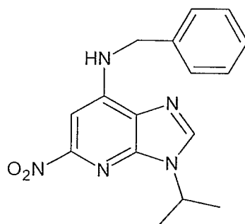
Formula Ie
