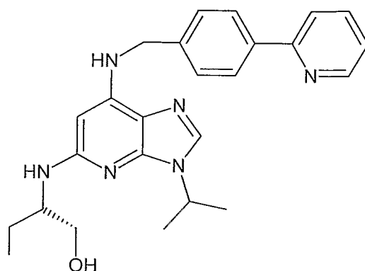
Formula Id
