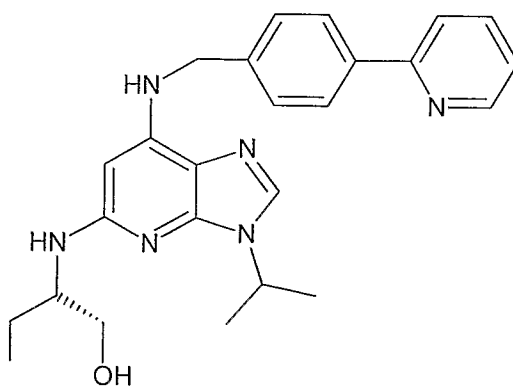
Formula Id
