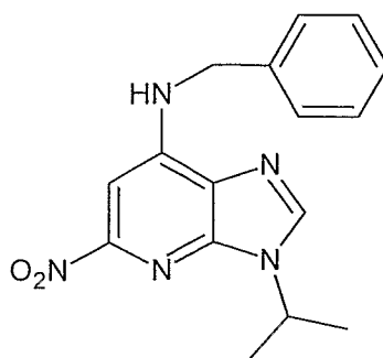
Formula Ie.
