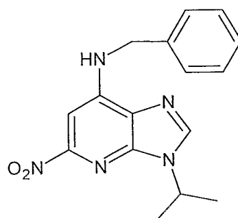
Formula Ie
