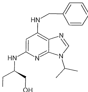
Formula Ia.
