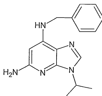
Formula If
