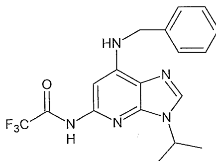
Formula Ig
