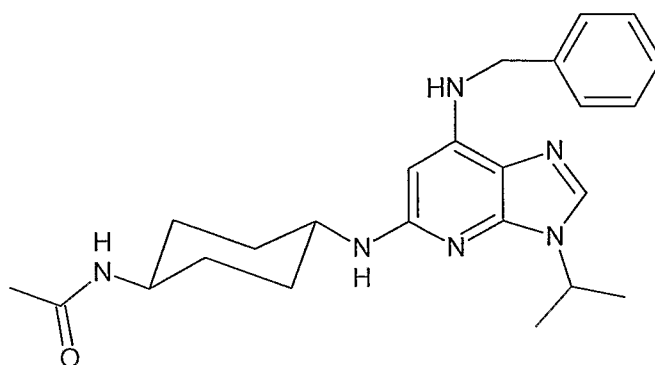
Formula Ih
