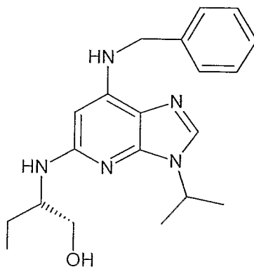
Formula Ib.
