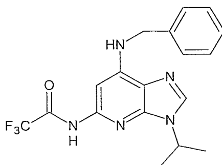
Formula 1g
