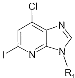
Formula V
