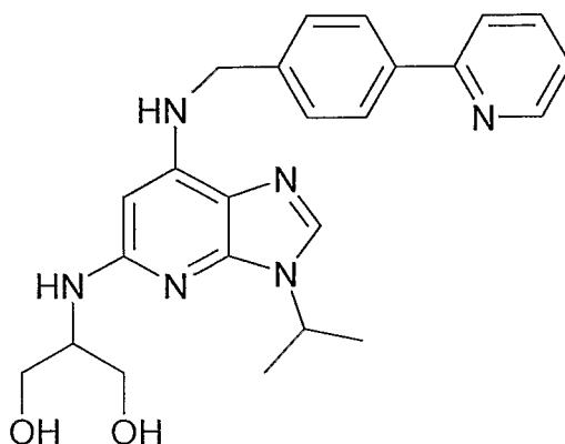
Formula Ii
