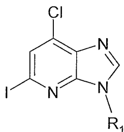
Compounds V
