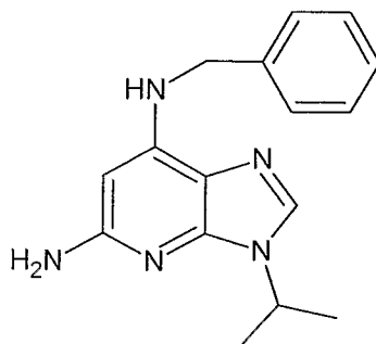
Formula If.
