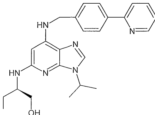
Formula Ic.
