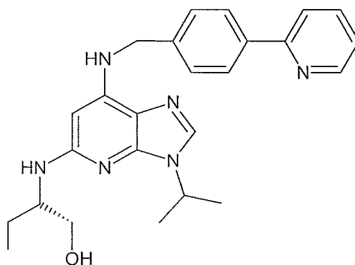
Formula Id.
