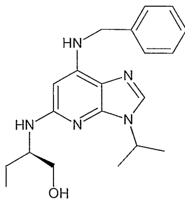
Formula Ia
