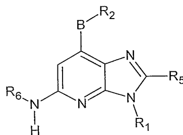
Formula V
