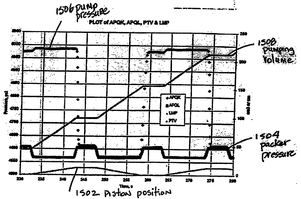
Fig. 15 History plot of pumping data used. Three strokes of BB pump.
