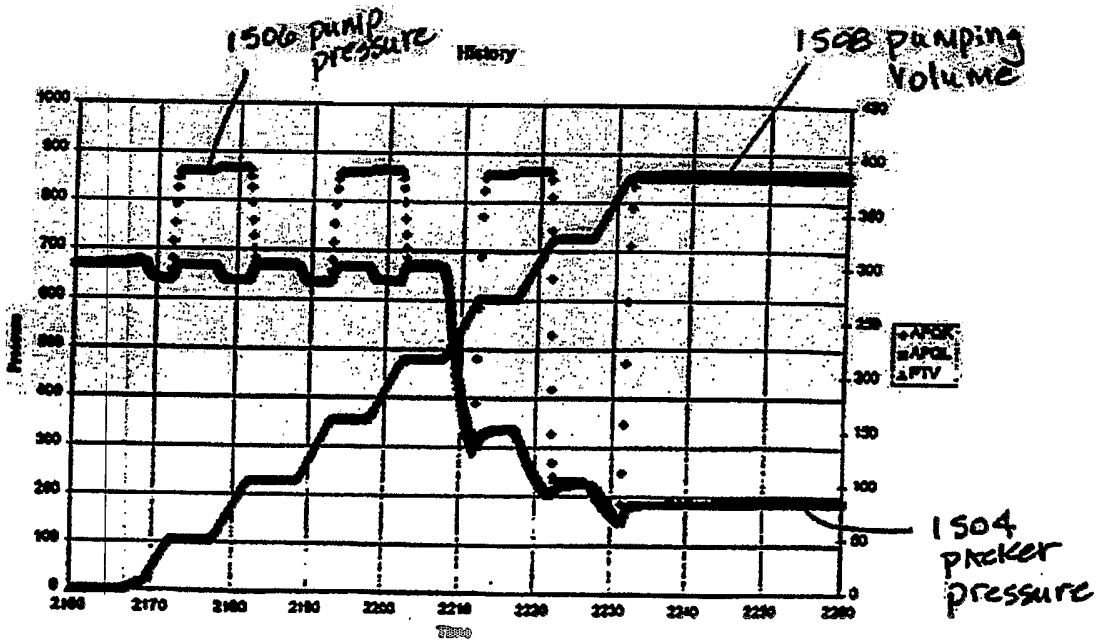
Fig. 17 Pumping history for example 2
