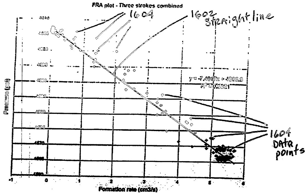
Fig. 16 FRA plot for the three strokes combined.
