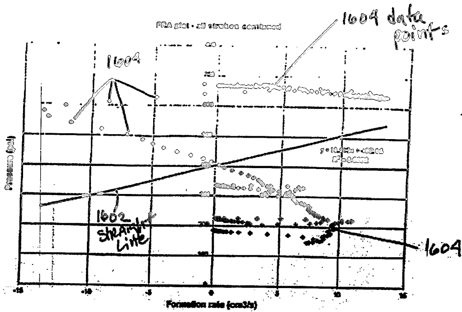
Fig. 18 FRA plot on all strokes, example 2
