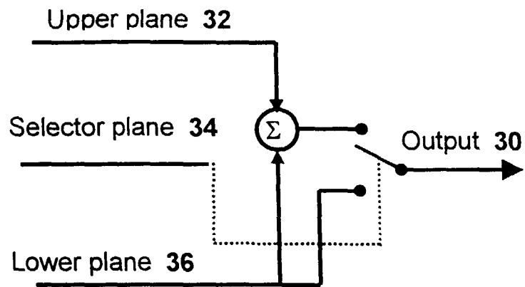
Figure 3A: Additive DIR Imaging Model Reconstruction
