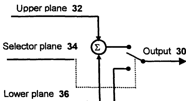
Figure 3A: Additive DIR Imaging Model Reconstruction
