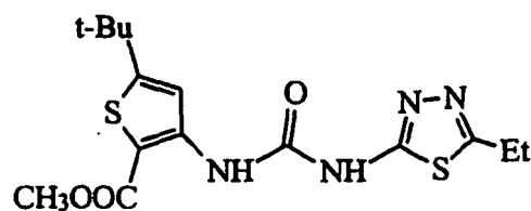
5-tert-Butyl-3-[3-(5-ethyl-[1,3,4]thiadiazol-2-yl)-ureido]-thiophene-2-carboxylic acid methyl ester
