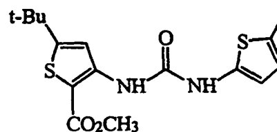
5-tert-Butyl-3-[3-(5-trifluoromethyl-[1,3,4]-thiadiazol-2-yl)-ureido]-thiophene-2-carboxylic acid methyl ester
