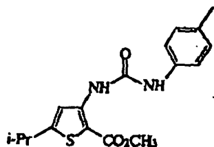
5-Isopropyl-3-(3-p-tolyl-ureido)-thiophene-2-carboxylic acid methyl ester
