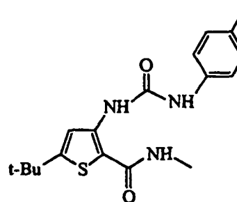
5-tert-Butyl-3-(3-p-tolyl-ureido)-thiophene-2-carboxylic acid methylamide
