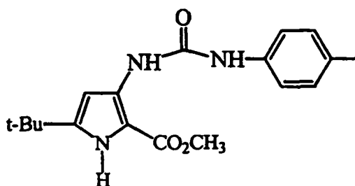
5-tert-Butyl-3-(3-p-tolyl-ureido)-1H-pyrrole-2-carboxylic acid methyl ester
