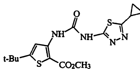
5-tert-Butyl-3-[3-(5-cyclopropyl-[1,3,4]thiadiazol-2-yl)-ureido]-thiophene-2-carboxylic acid methyl ester
