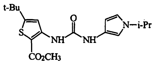
5-tert-Butyl-3-[3-(1-isopropyl-1H-pyrrol-3-yl)-ureido]-thiophene-2-carboxylic acid methyl ester
