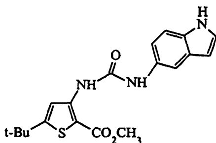
5-tert-Butyl-3-[3-(1H-indol-5-yl)-ureido]-thiophene-2-carboxylic acid methyl ester
