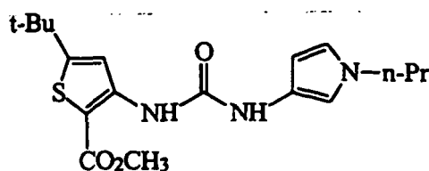
5-tert-Butyl-3-[3-(1-propyl-1H-pyrrol-3-yl)-ureido]-thiophene-2-carboxylic acid methyl ester
