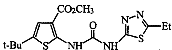
5-tert-Butyl-2-(3-(5-ethyl-[1,3,4]thiadiazol-2-yl)-ureido)-thiophene-3-carboxylic acid methyl ester
