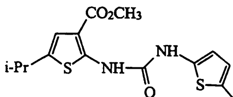
5-Isopropyl-2-[3-(5-methyl-thiophen-2-yl)-ureido]-thiophene-3-carboxylic acid methyl ester
