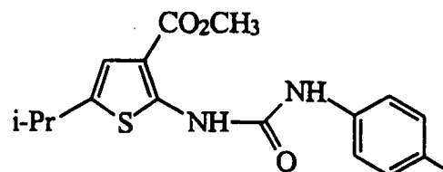
5-Isopropyl-2-(3-p-tolyl-ureido)-thiophene-3-carboxylic acid methyl ester
