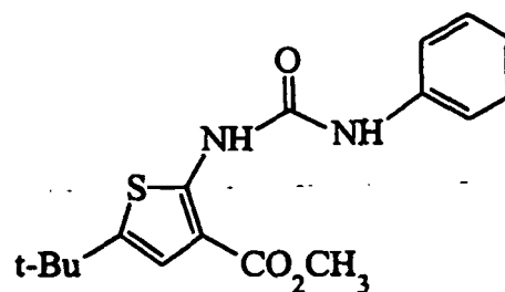
5-tert-Butyl-2-(3-phenyl-ureido)-thiophene-3-carboxylic acid methyl ester
