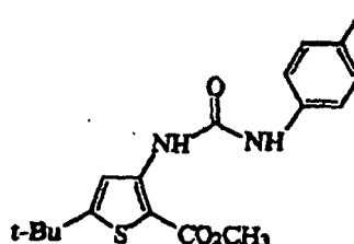
5-tert-Butyl-3-(3-p-tolyl-ureido)-thiophene 2-carboxylic acid methyl ester
