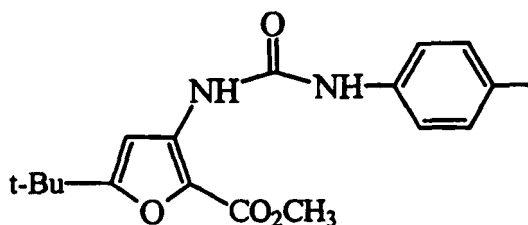
5-tert-Butyl-3-[3-(p-tolyl-ureido)-furan-2-carboxylic acid methyl ester
