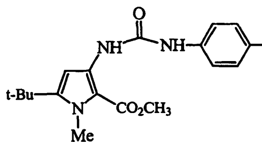
5-tert-Butyl-1-methyl-3-(3-p-tolyl-ureido)-1H-pyrrole-2-carboxylic acid methyl ester
