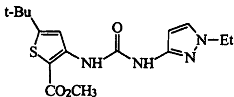
5-tert-Butyl-3-[3-(1-ethyl-1H-pyrazol-3-yl)-ureido]-thiophene-2-carboxylic acid methyl ester
