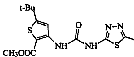
5-tert-Butyl-3-[3-(5-methyl-[1,3,4]thiadiazol-2-yl)-ureido]-thiophene-2-carboxylic acid methyl ester
