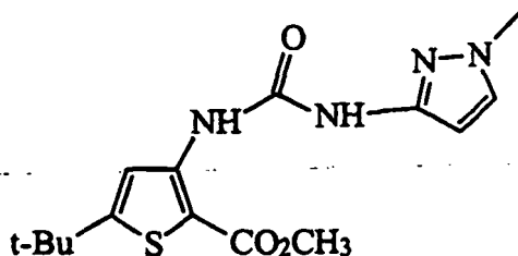
5-tert-Butyl-3-[3-(1-methyl-1H-pyrazol-3-yl)-ureido]-thiophene-2-carboxylic acid methyl ester
