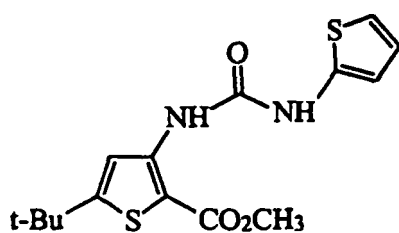
5-tert-Butyl-3-(3-thiophen-2-yl-ureido)-thiophene-2-carboxylic acid methyl ester
