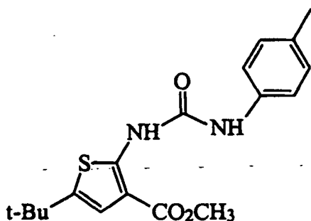
5-tert-Butyl-2-(3-p-tolyl-ureido)-thiophene-3-carboxylic acid methyl ester
