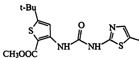
5-tert-Butyl-3-[3-(5-methyl-thiazol-2-yl)-ureido]-thiophene-2-carboxylic acid methyl ester
