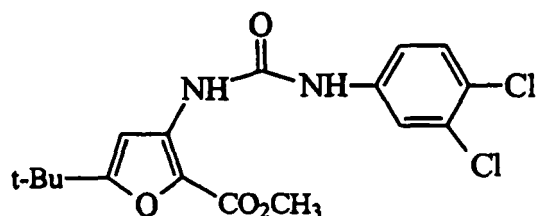
5-tert-Butyl-3-[3-(3,4-dichloro-phenyl)-ureido]-furan-2-carboxylic acid methyl ester
