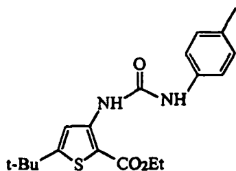
5-tert-Butyl-3-(3-p-tolyl-ureido)-thiophene-2-carboxylic acid ethyl ester
