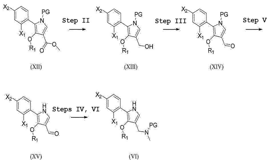
[Reaction Scheme 4]
