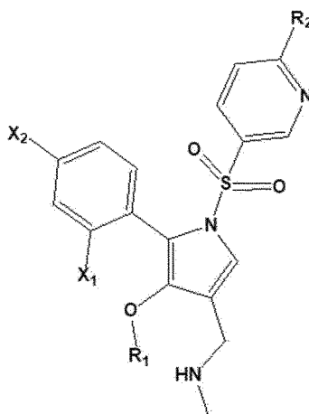
[Chemical Formula 2]
