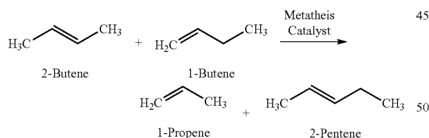
Formula 3: Cross-Metathesis
