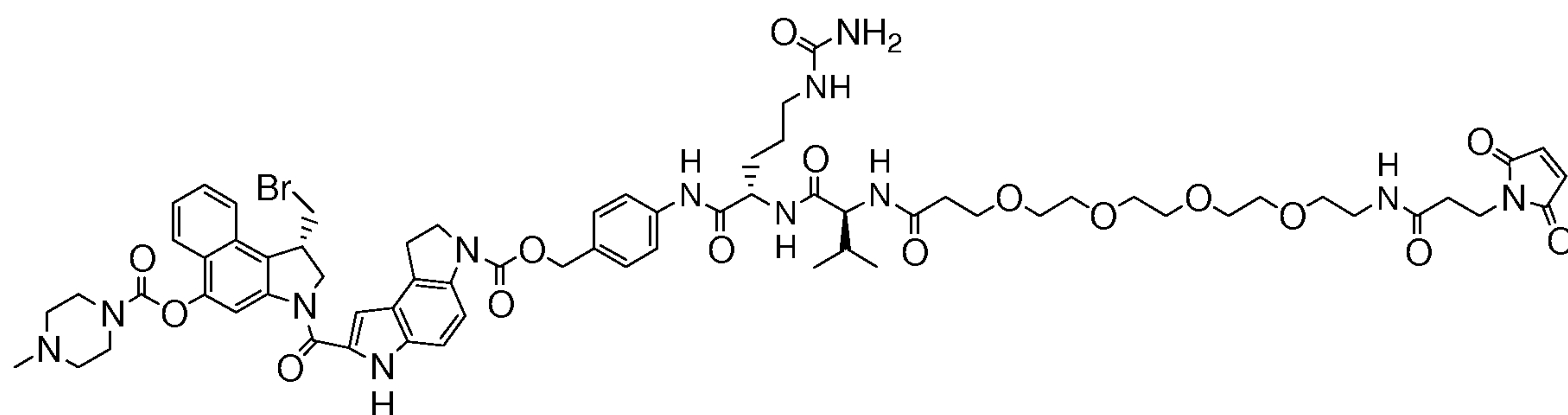
Compound H
