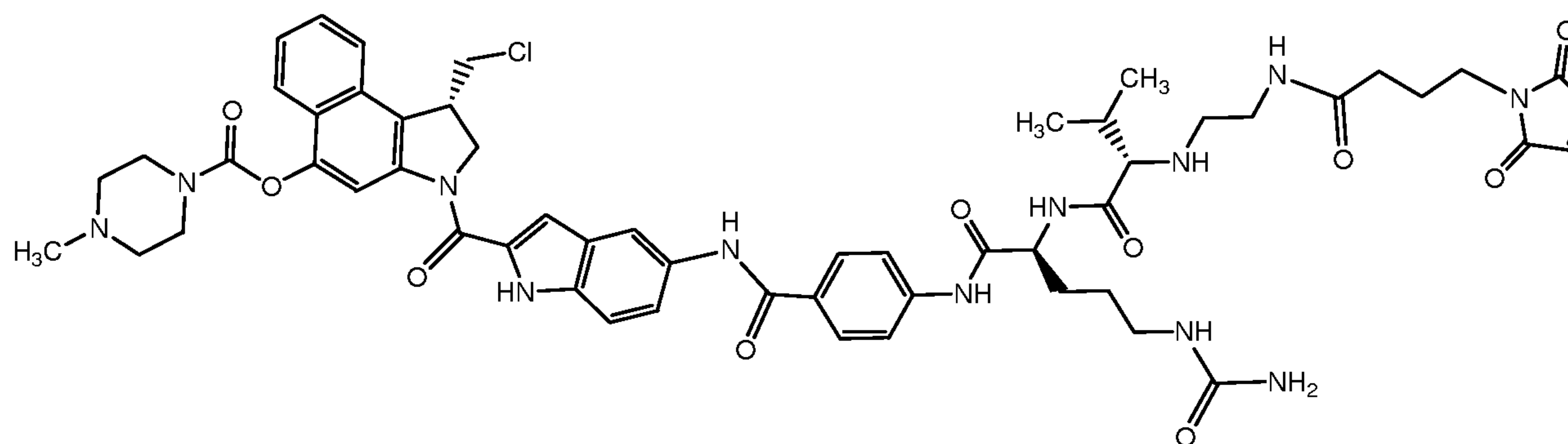
Compound I
