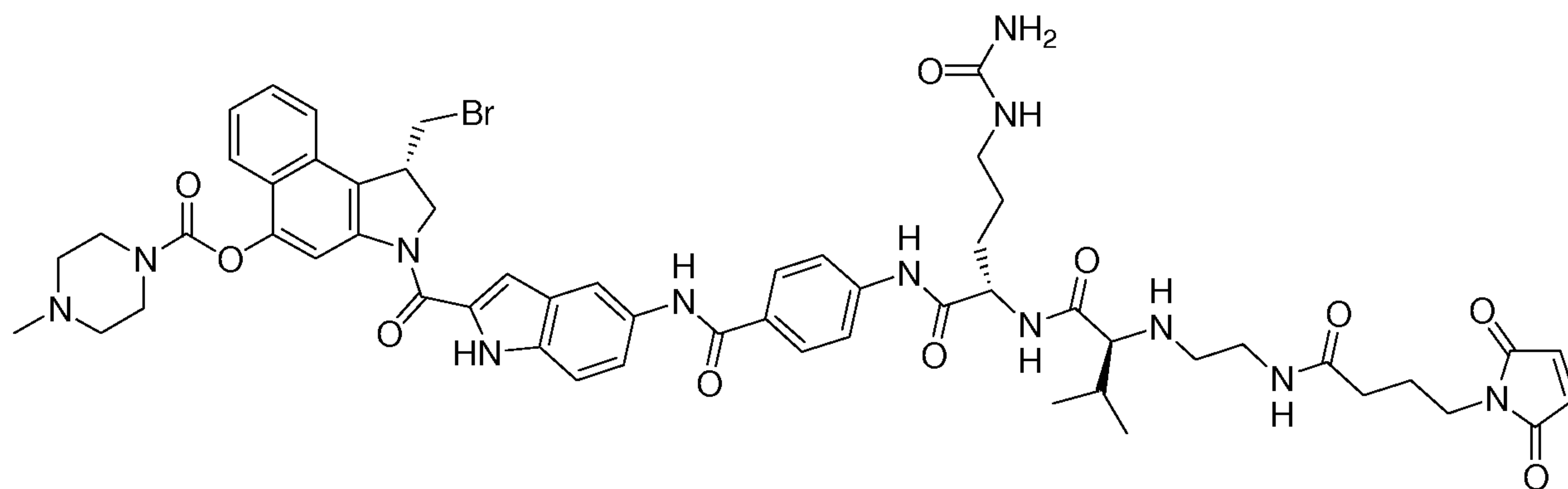
Compound H
