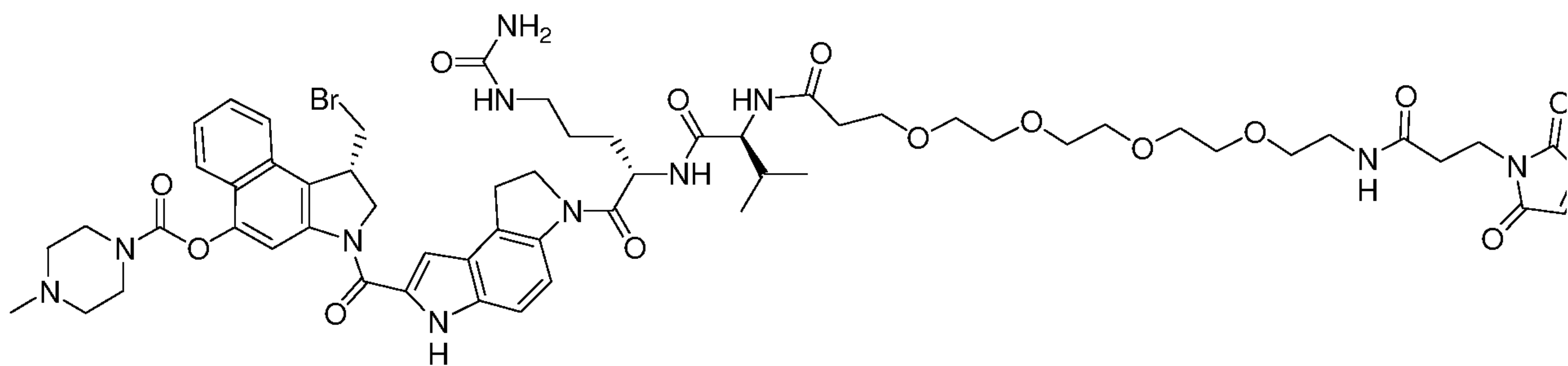
Compound G
