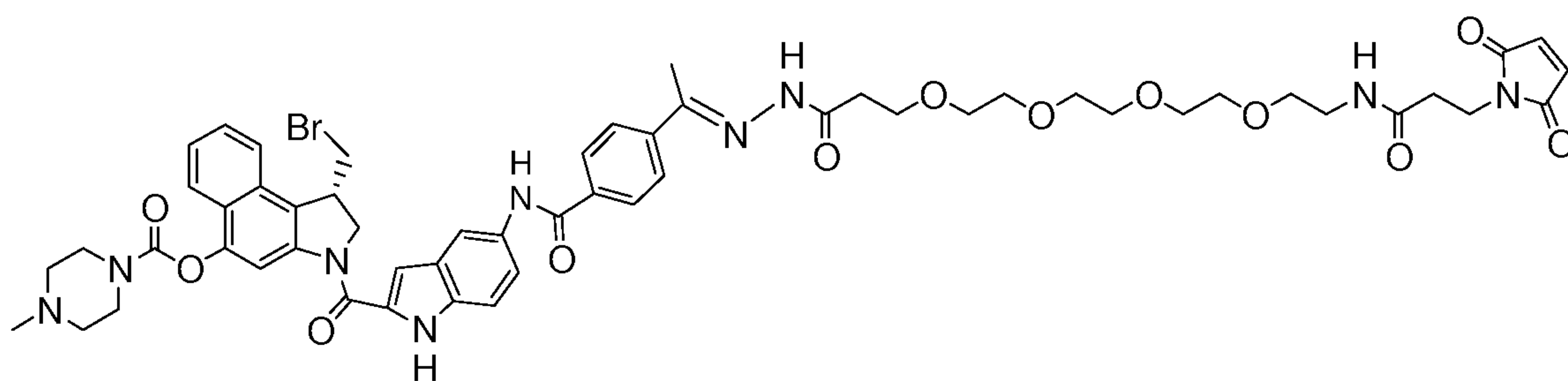
Compound C
