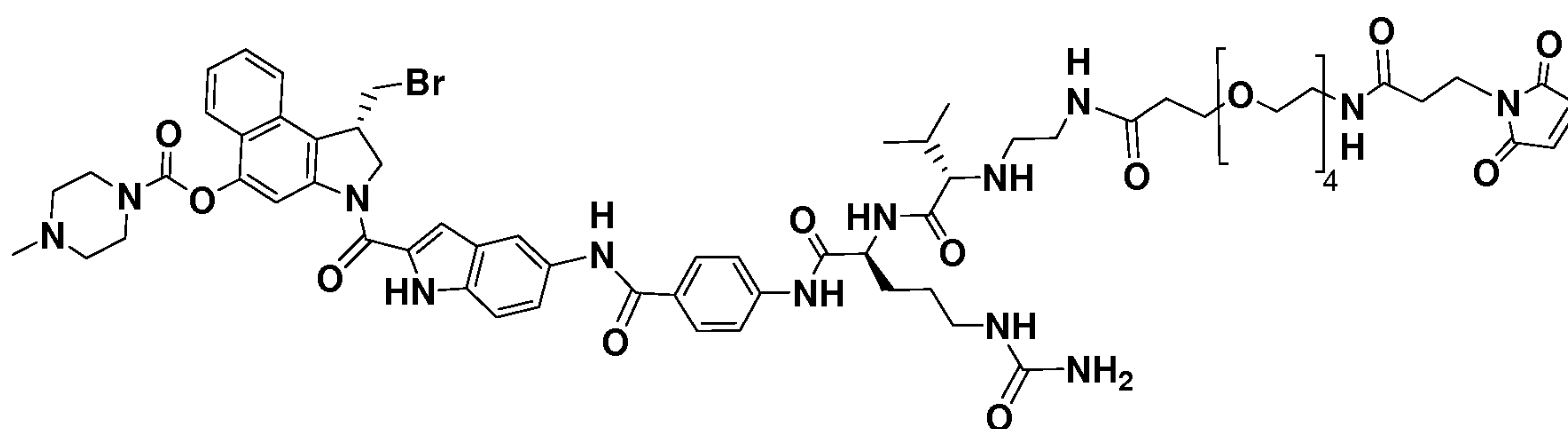
Compound A
