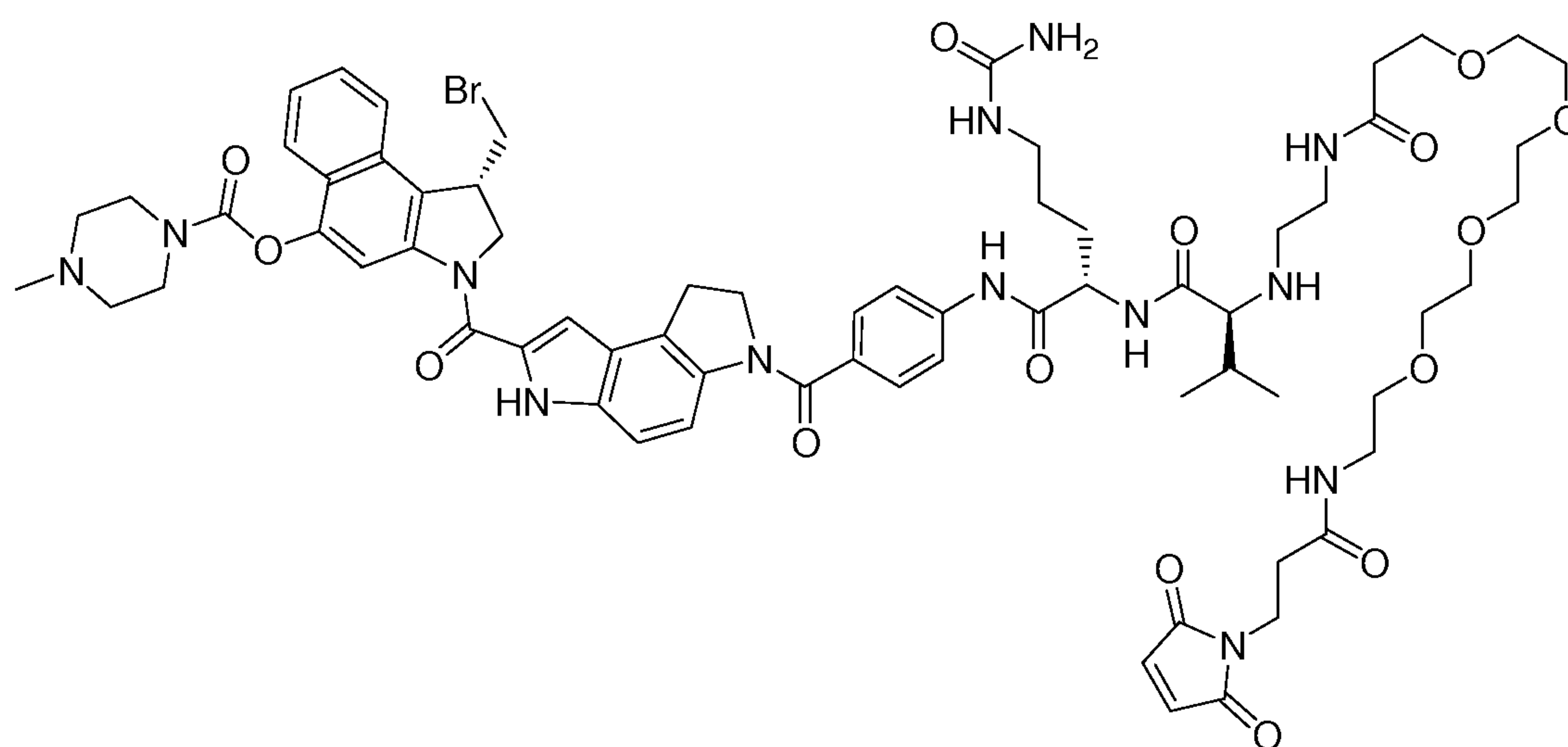
Compound F
