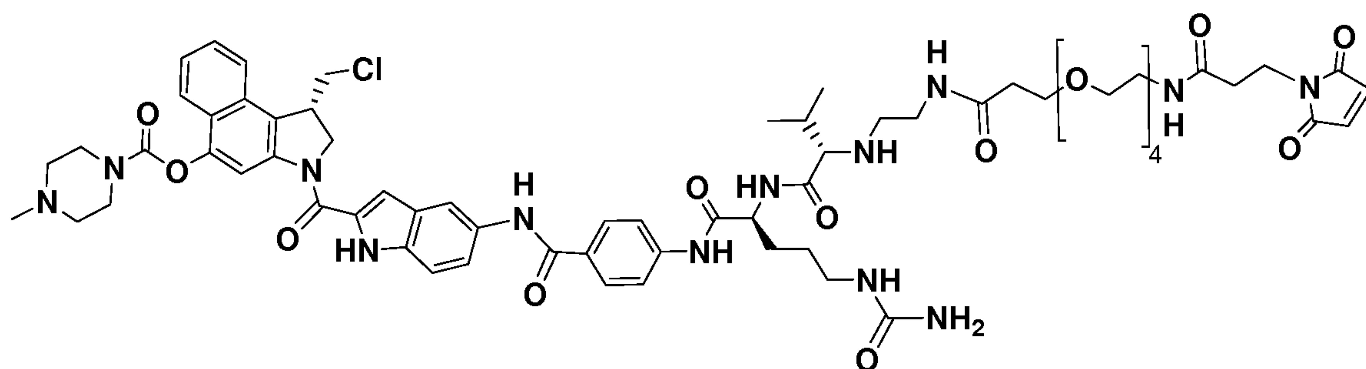
Compound D
