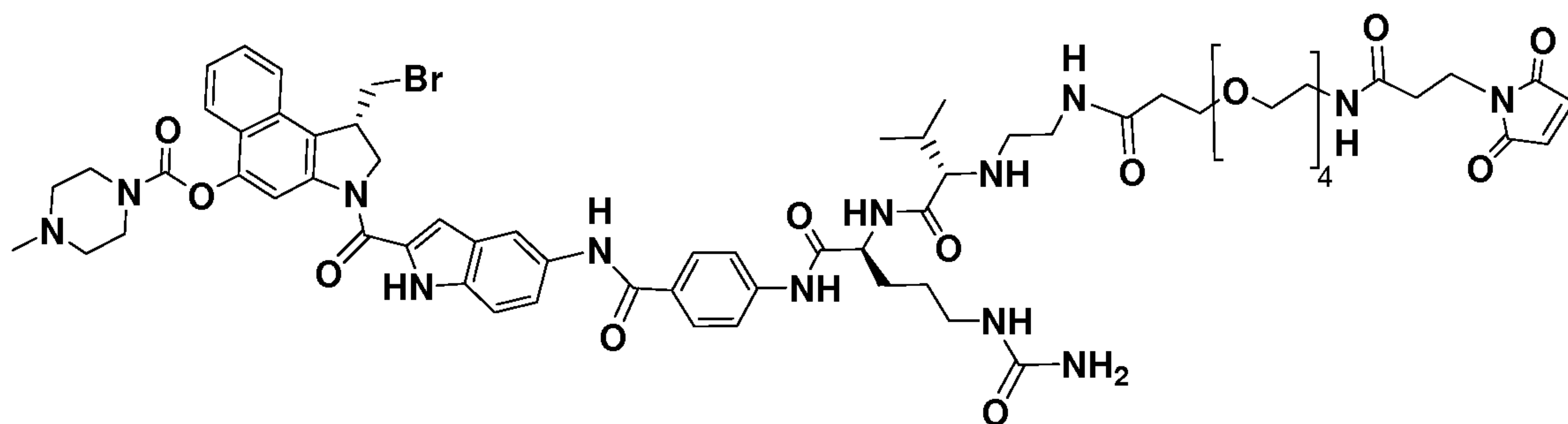
Compound A
