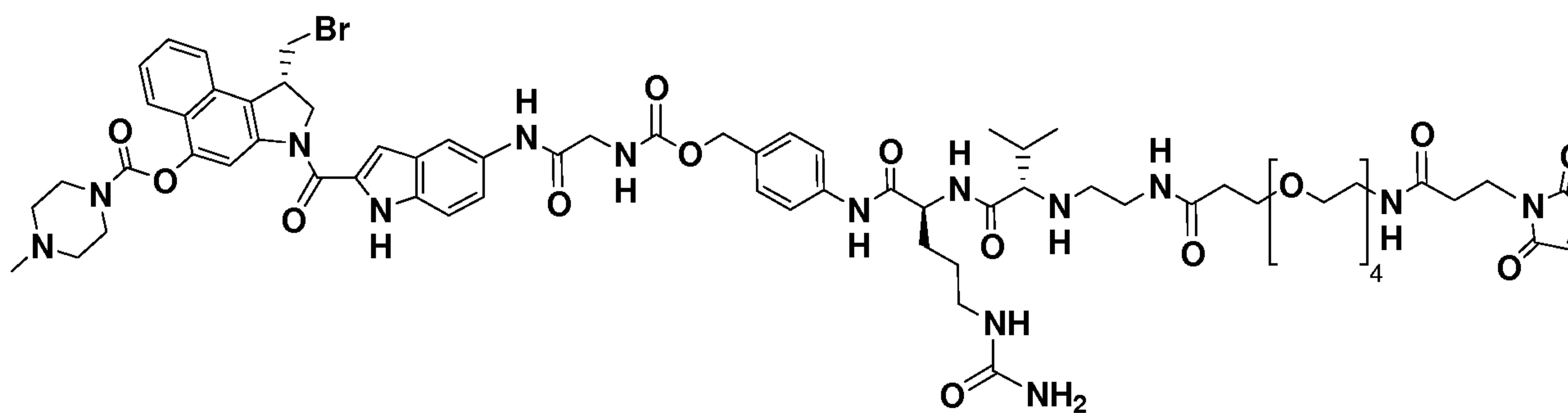
Compound D
