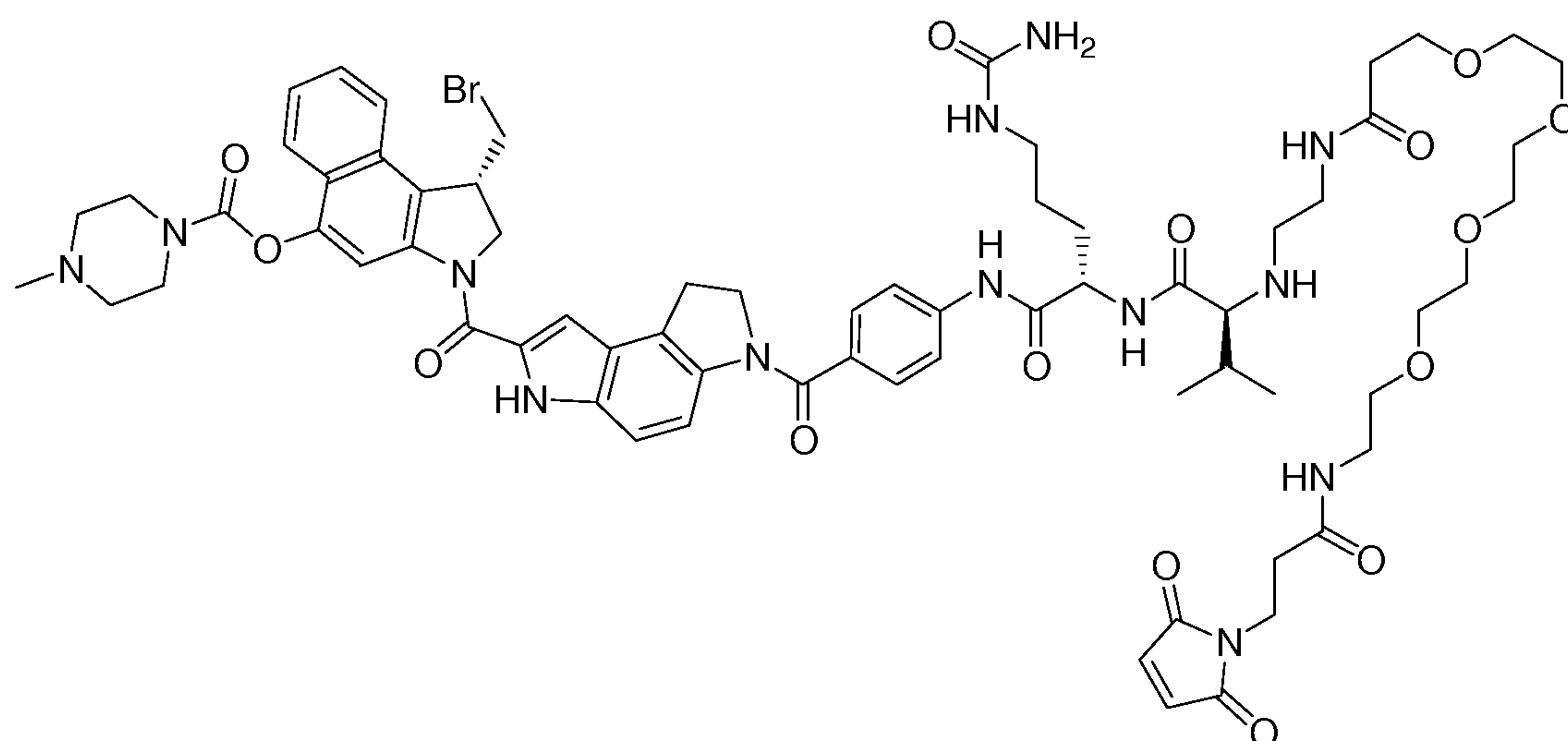
Compound F
