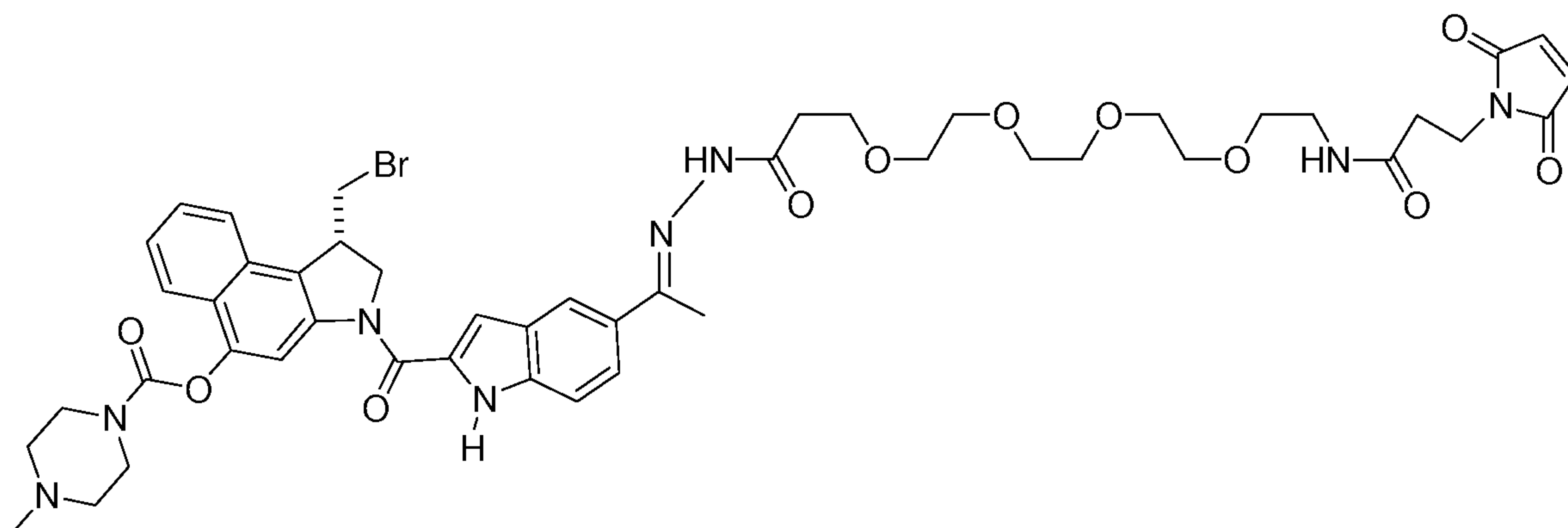
Compound A
