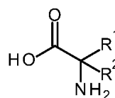
alpha-amino acid
