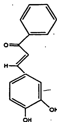
Chalcone (15)
