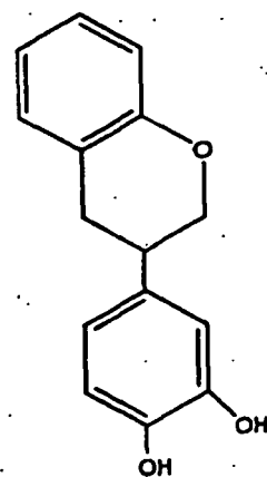
Isoflavan (13)
