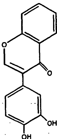
Isoflavone (9)
