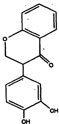
Isoflavanone (11)
