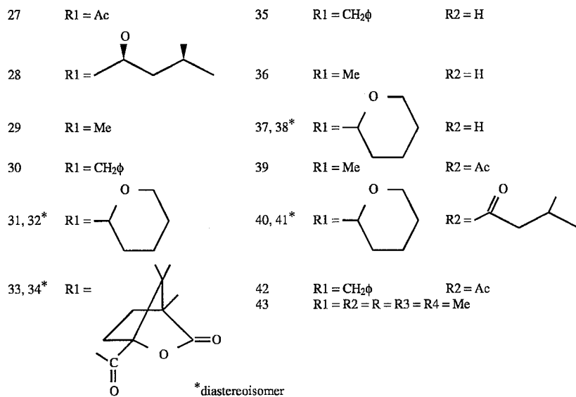
Scheme 4. Syntheses of 3',4'-trans-khellactone and benzodihydropyran derivatives
