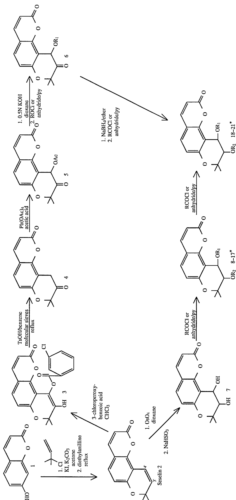
Scheme 1. Synthesis of 3,4'-cis-khellactone derivatives
