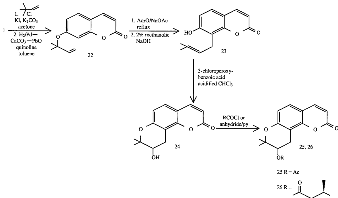
Scheme 3. Synthesis of 3' jatamansinol derivatives
