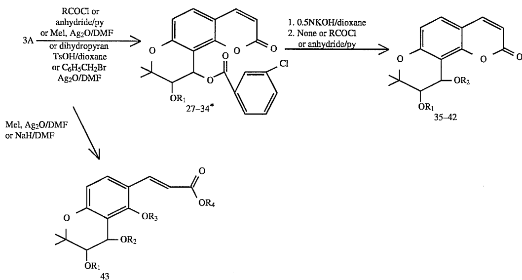
Scheme 4. Syntheses of 3',4'-trans-khellactone and benzodihydropyran derivatives
