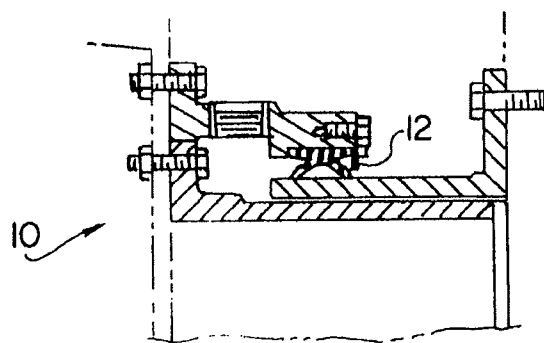
FIG. 2 (PRIOR ART)
