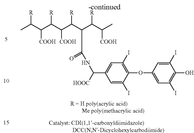
Sketch 2B: Schematic Route of T4/Polymer Conjugates Synthesis via Amine Group
