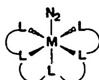
1 Pentadentate 1 N 2
