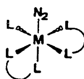
1 Pentadentate 1 N 2
