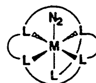
1 Pentadentate 1 N 2
