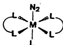
1 Pentadentate 1 N 2
