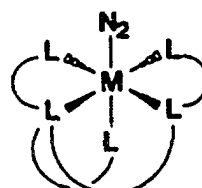
1 Pentadentate 1 N 2
