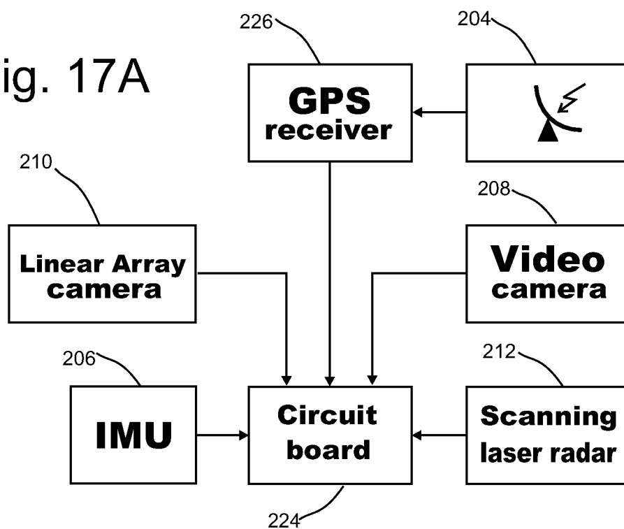
Data acquisition module
