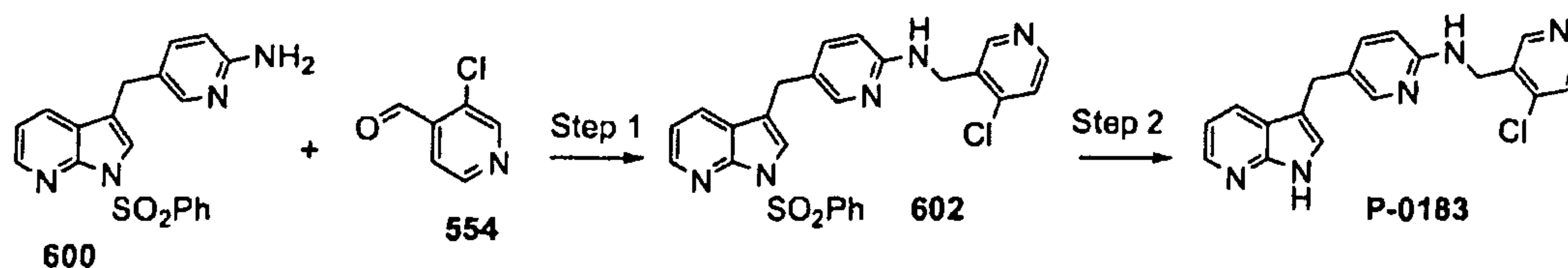
Scheme 187
