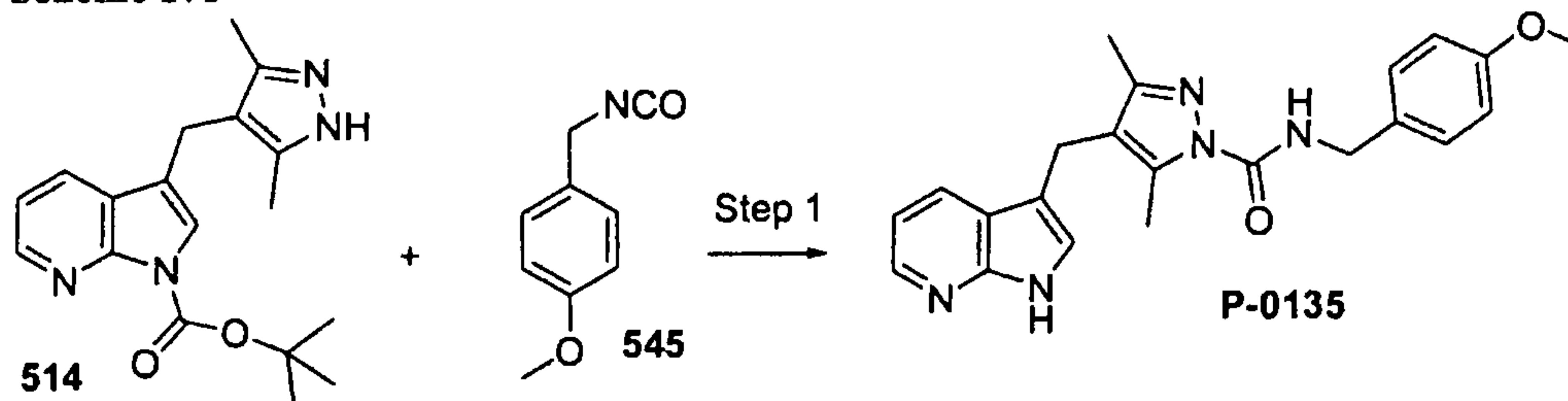
Scheme 171
