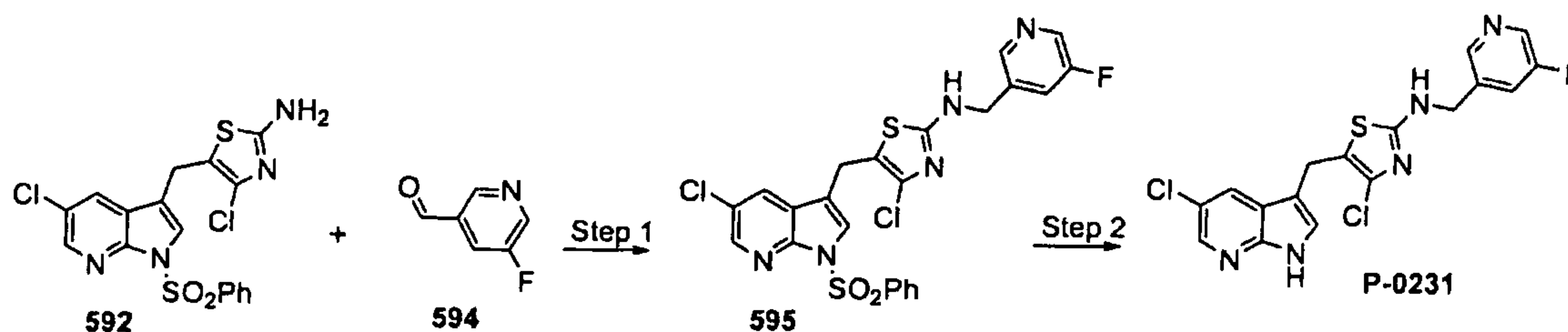
Scheme 184
