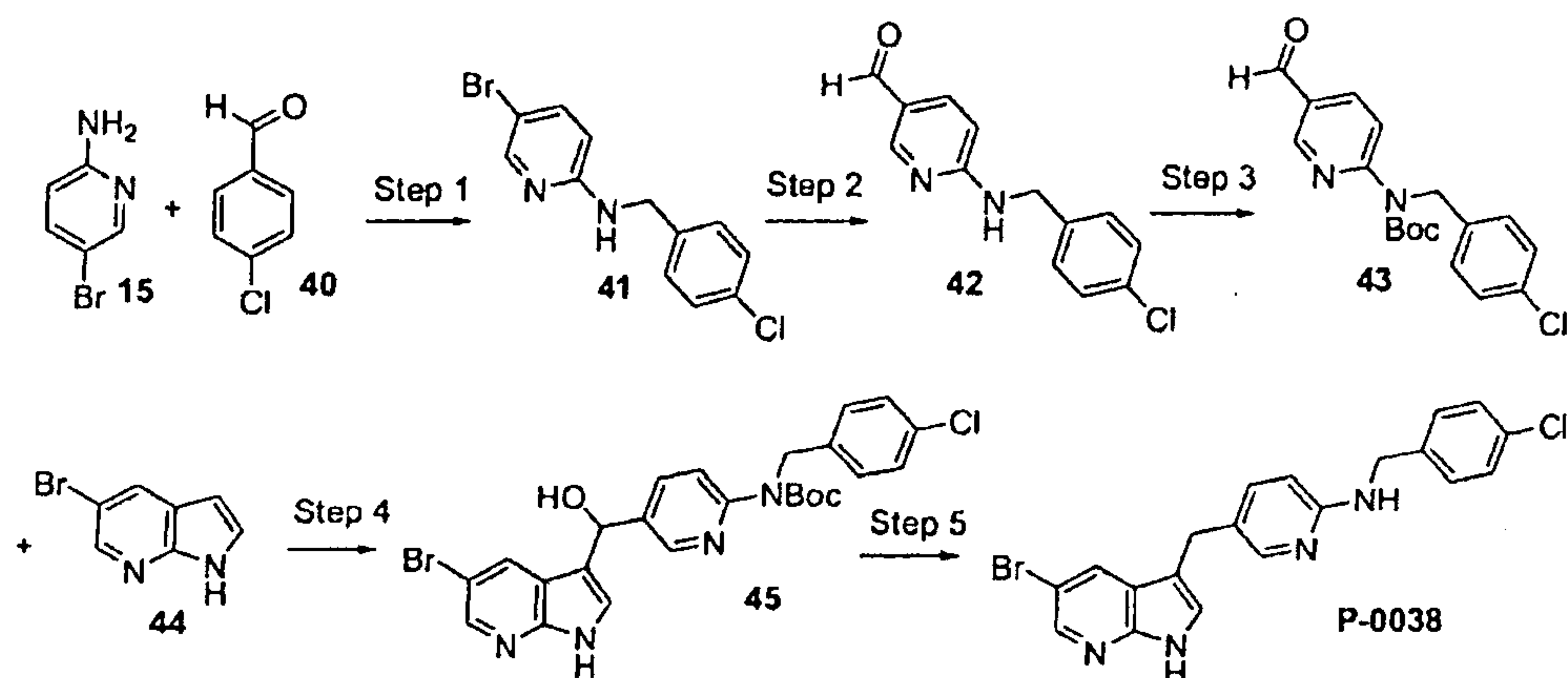
Scheme 19
