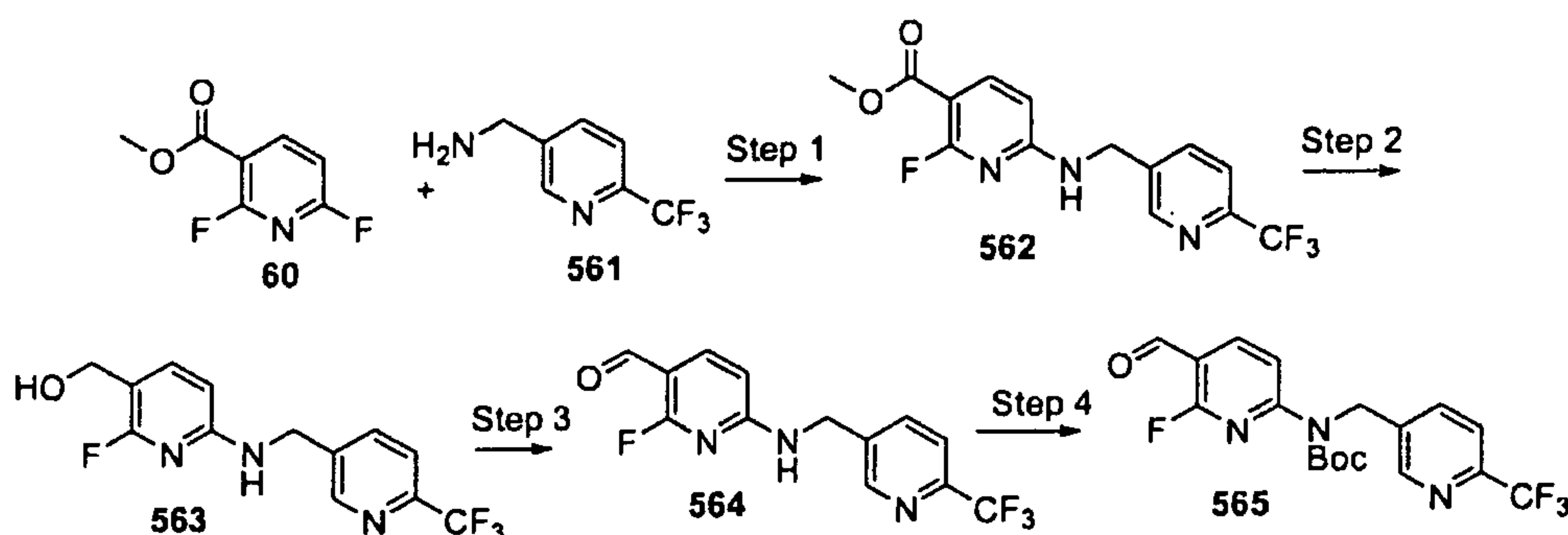
Scheme 176
