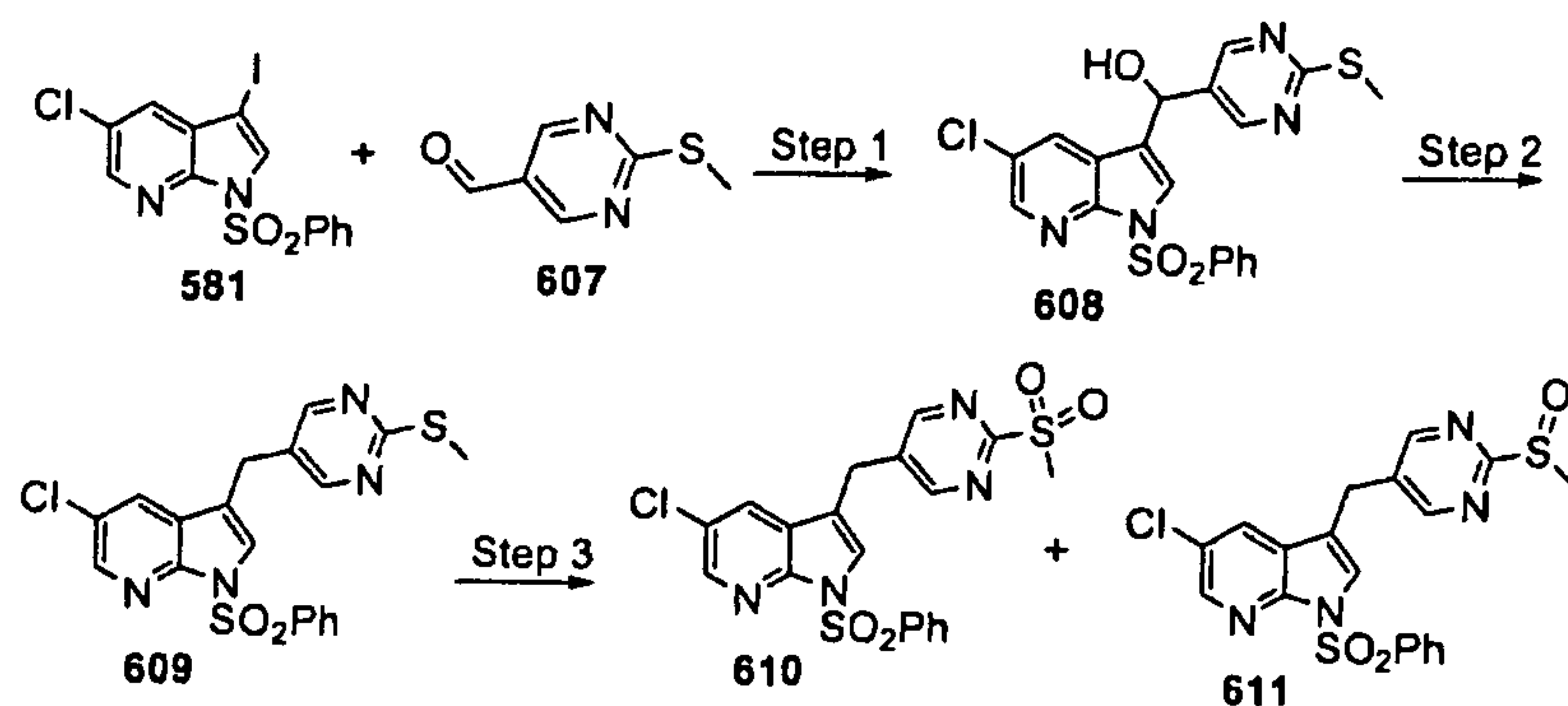
Scheme 191
