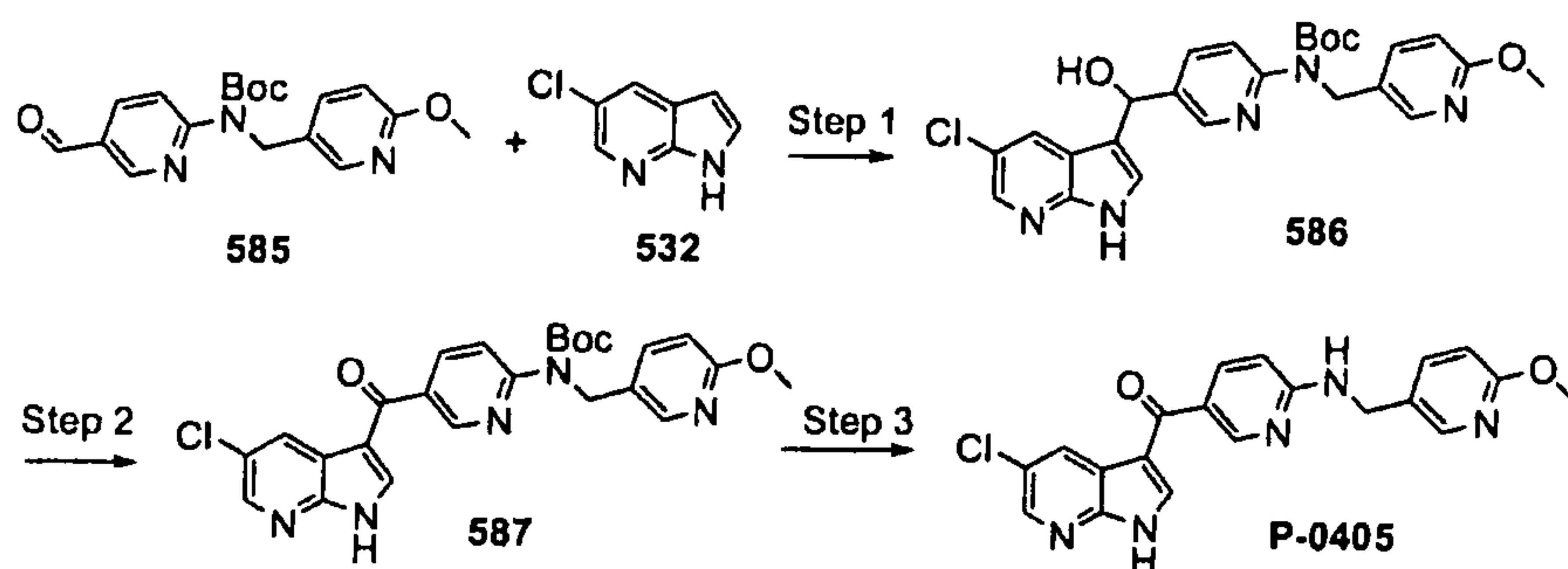
Scheme 182
