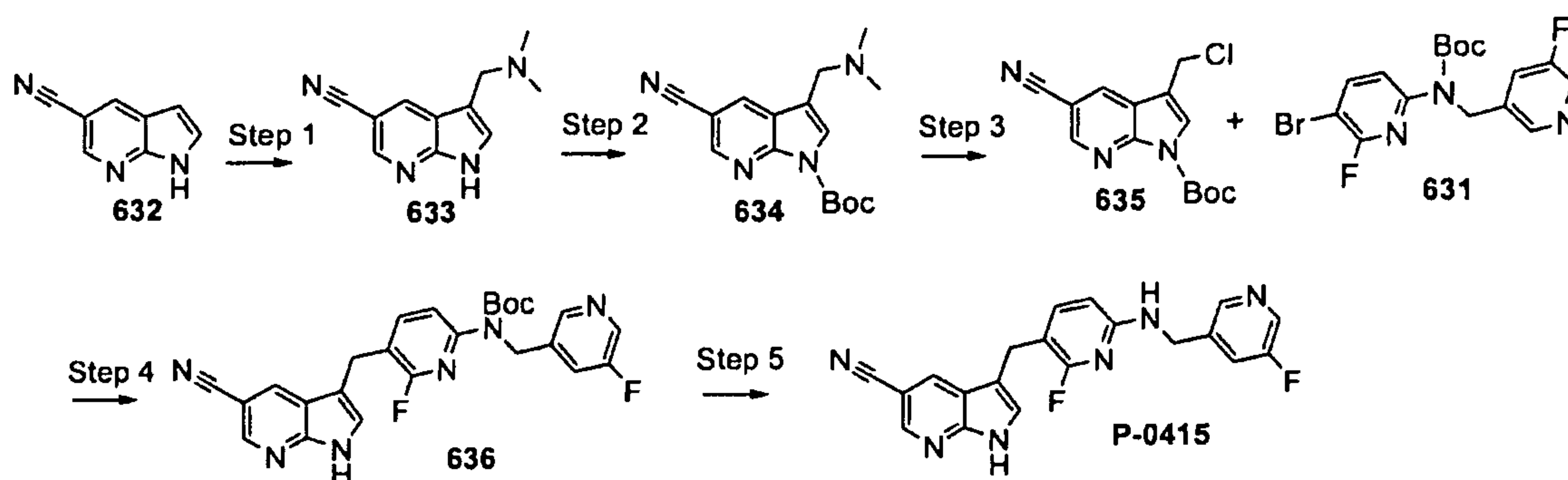
Scheme 201
