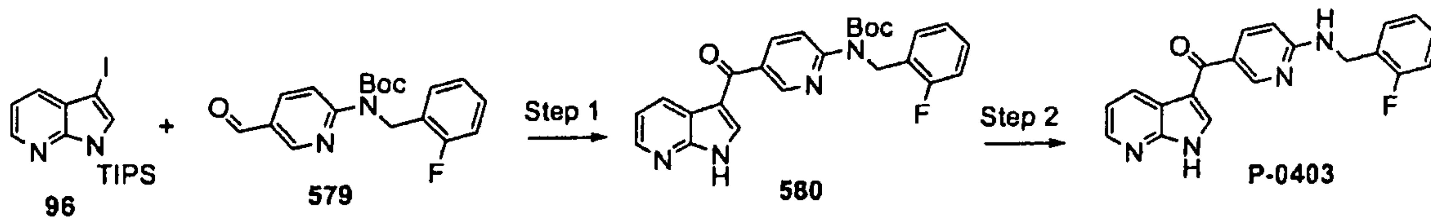
Scheme 180
