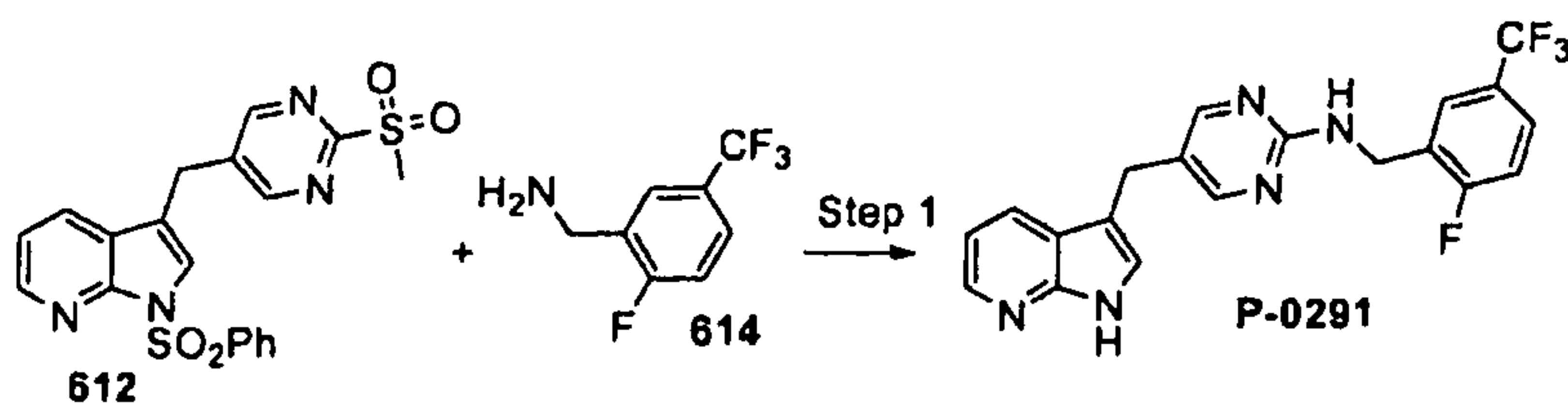
Scheme 193
