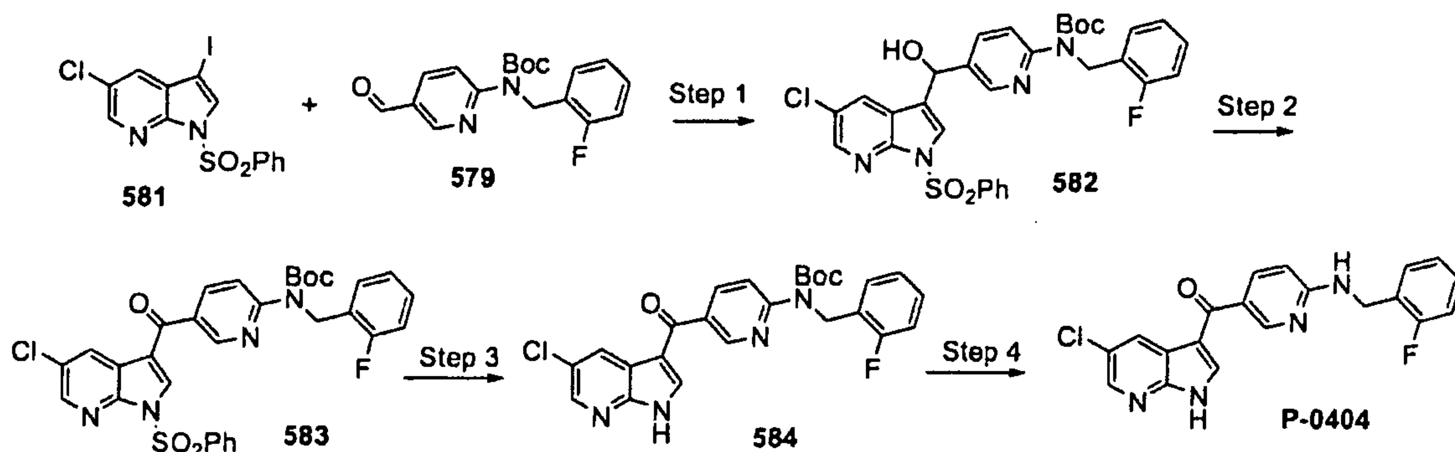
Scheme 181
