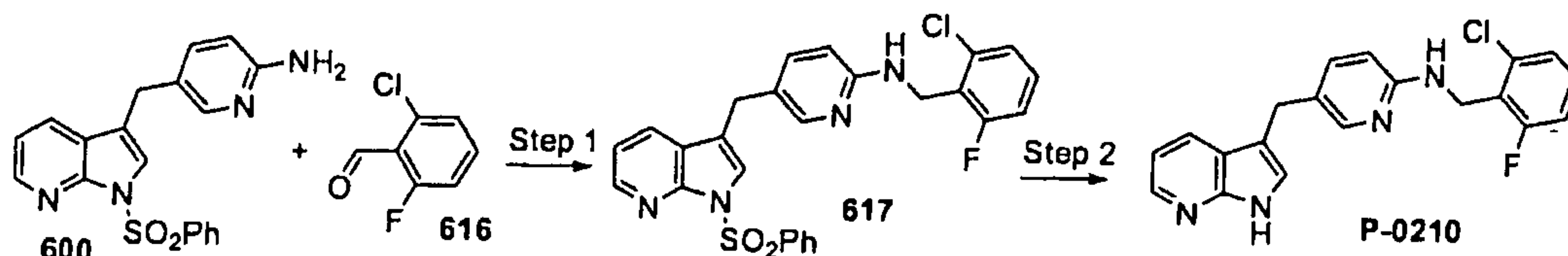
Scheme 195
