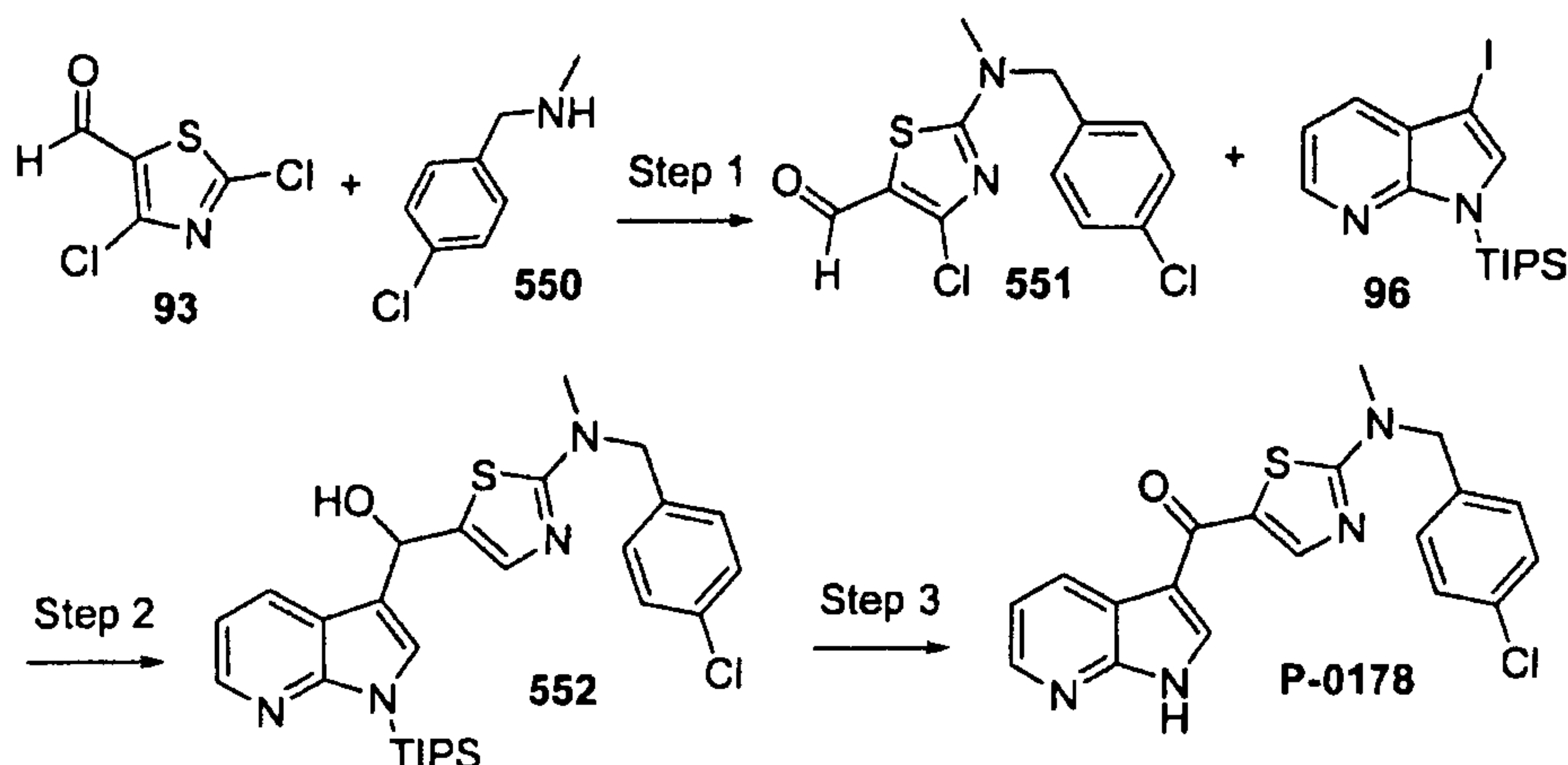
Scheme 174
