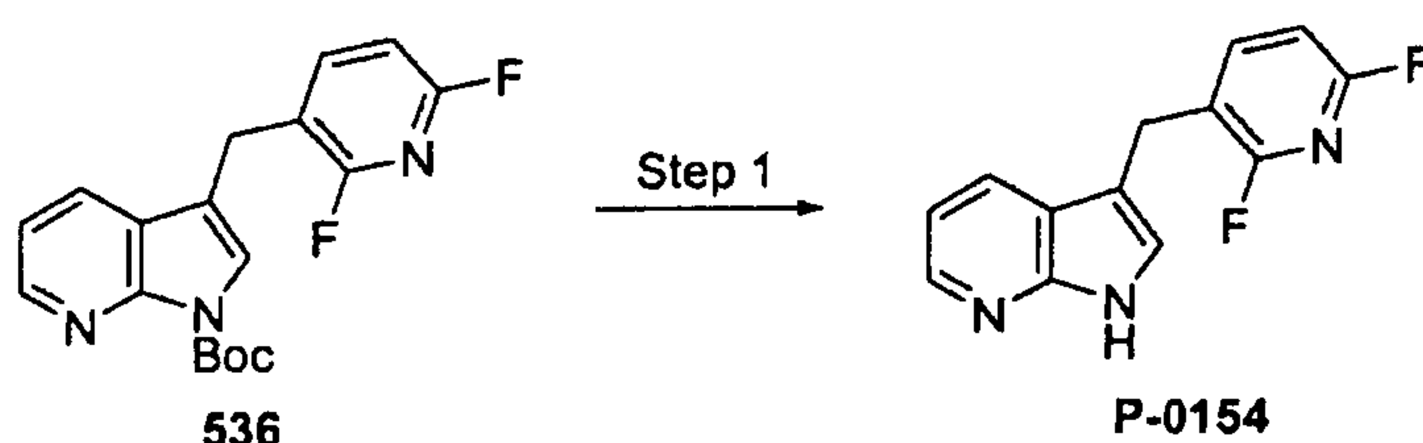
Scheme 167
