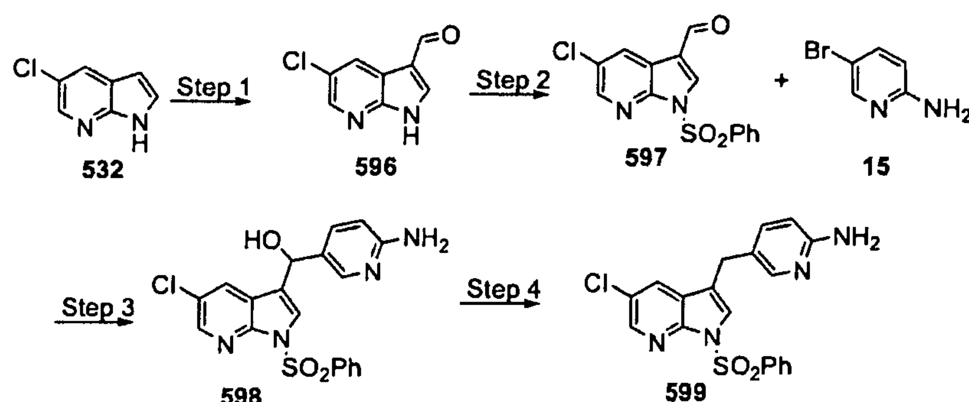
Scheme 185
