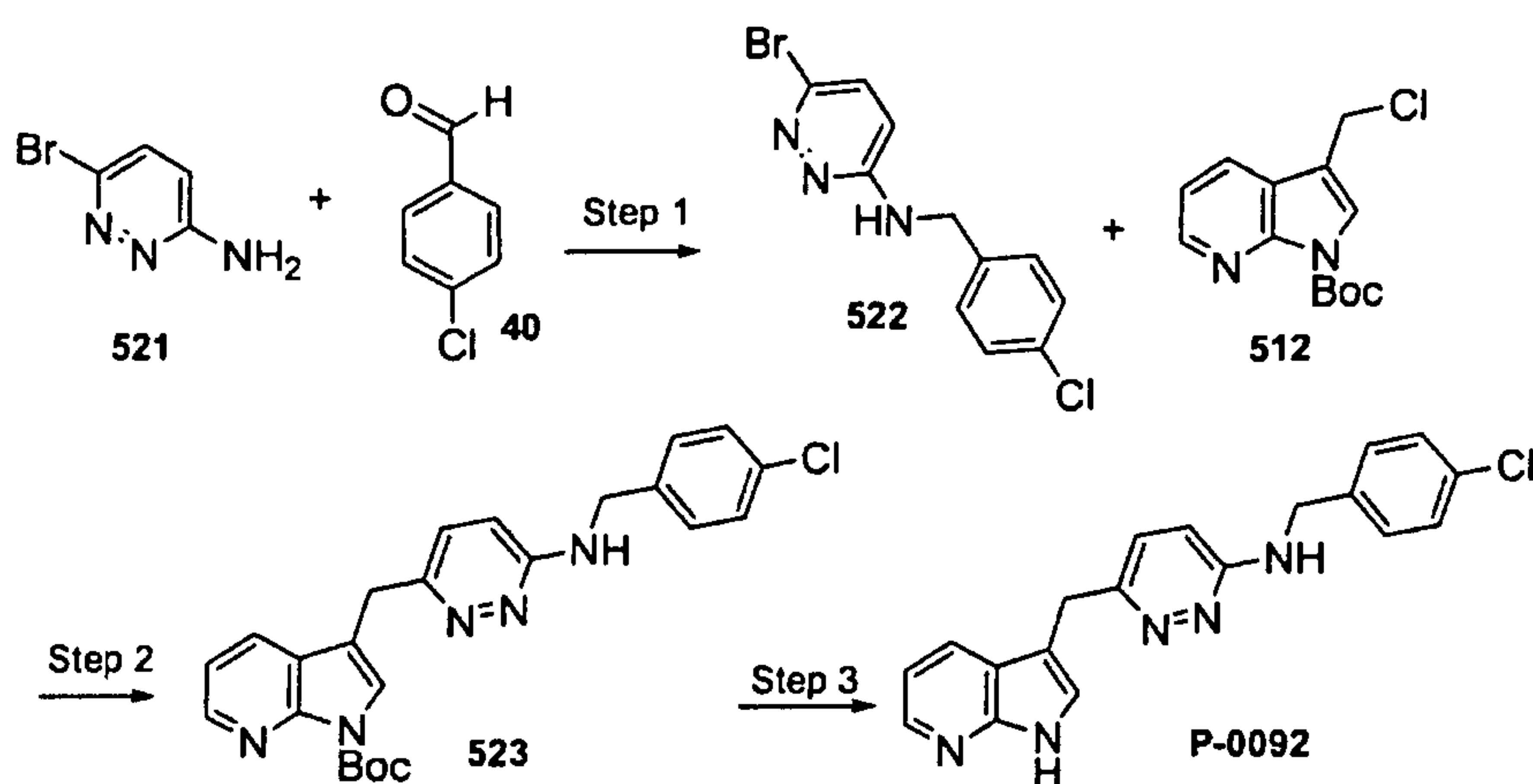
Scheme 161
