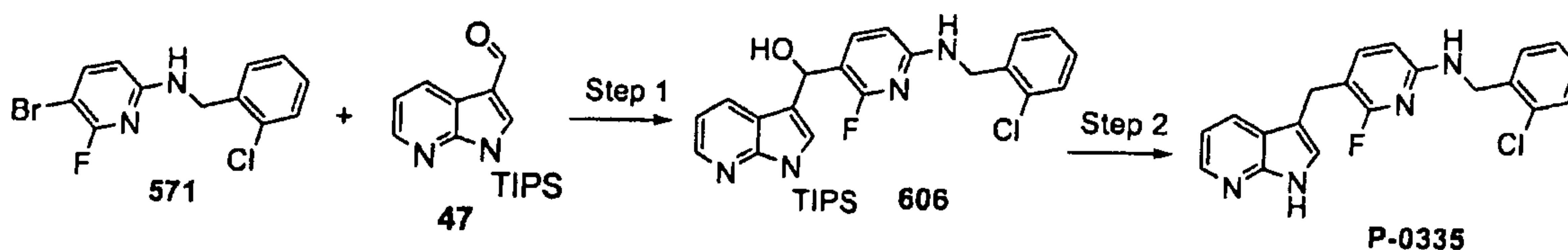
Scheme 190
