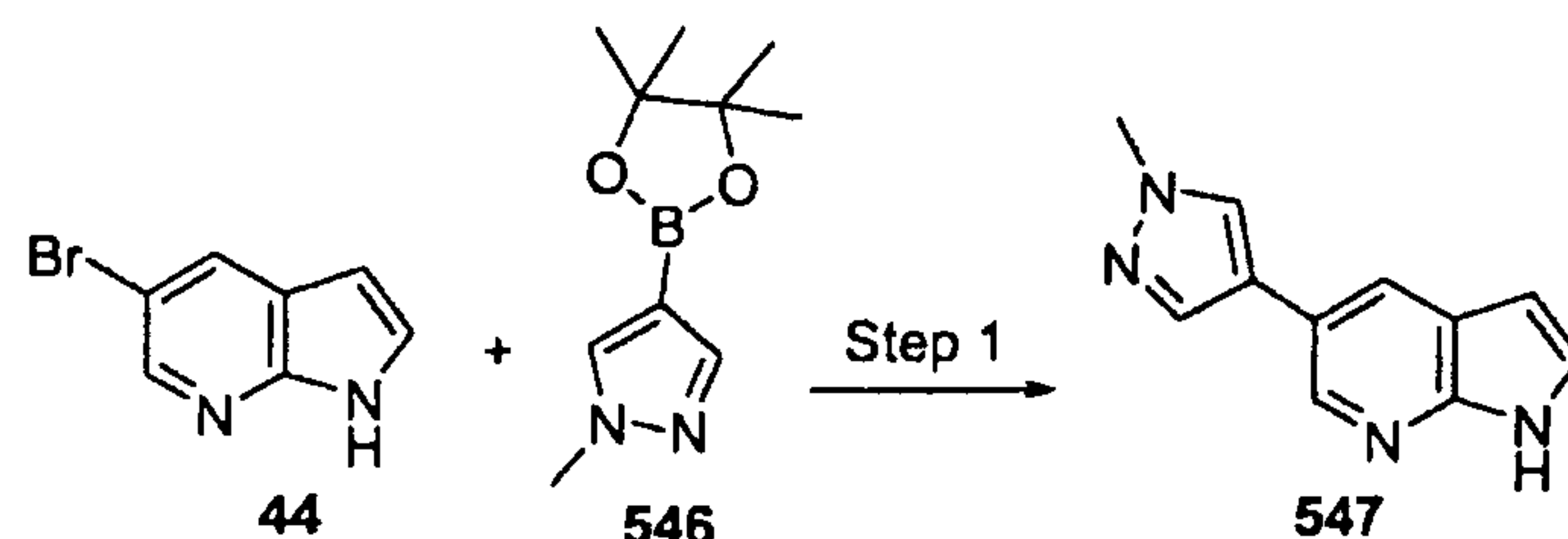
Scheme 172
