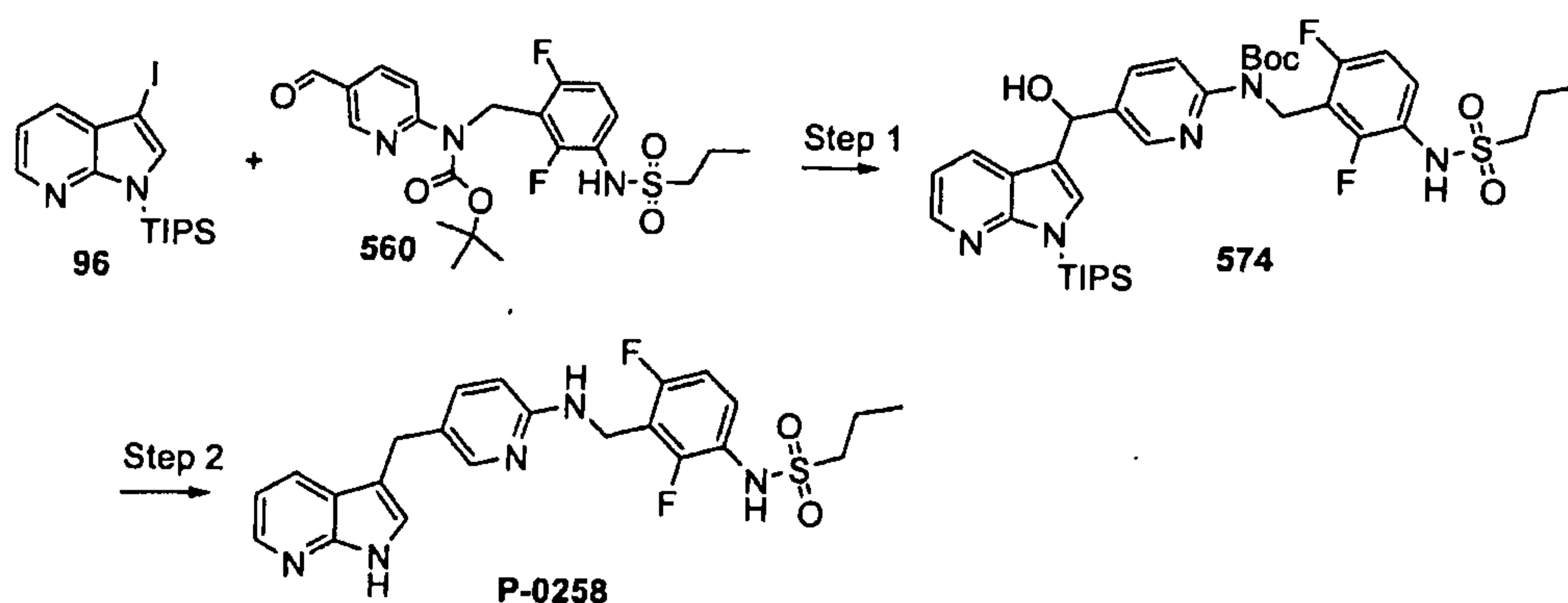
Scheme 178
