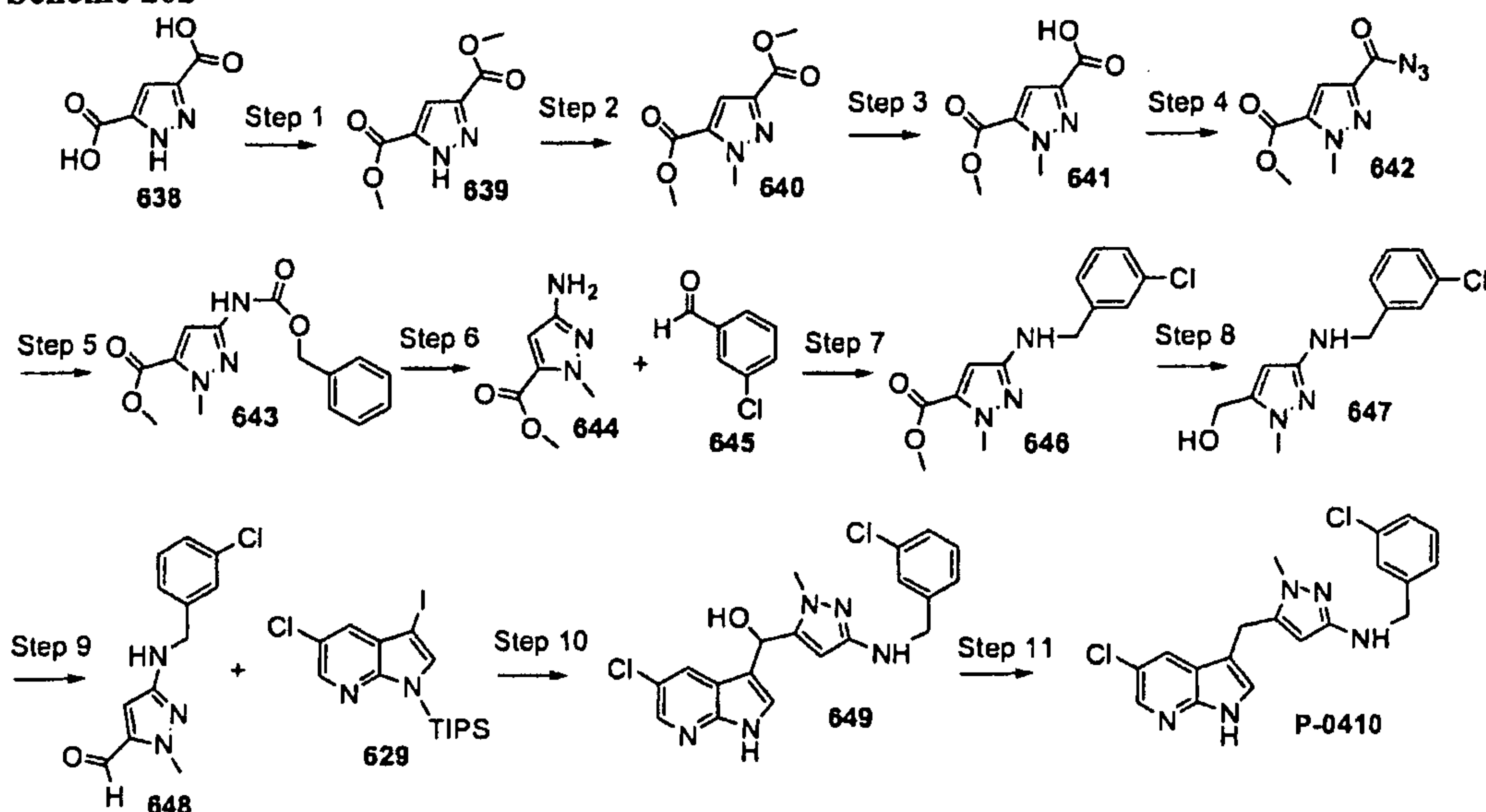
Scheme 202
