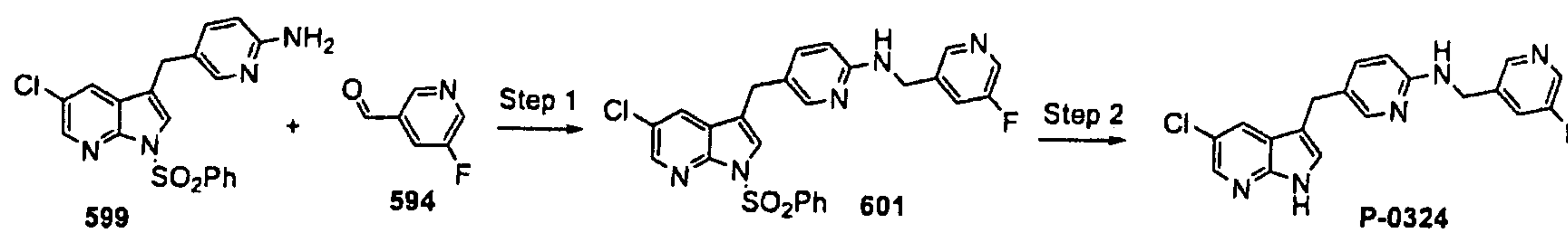
Scheme 186
