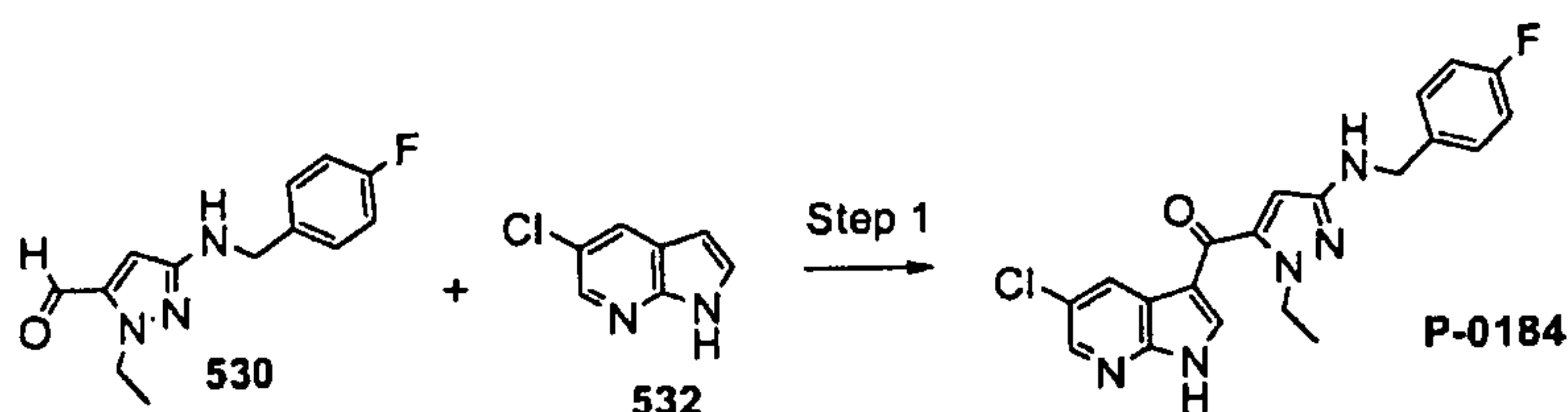
Scheme 199
