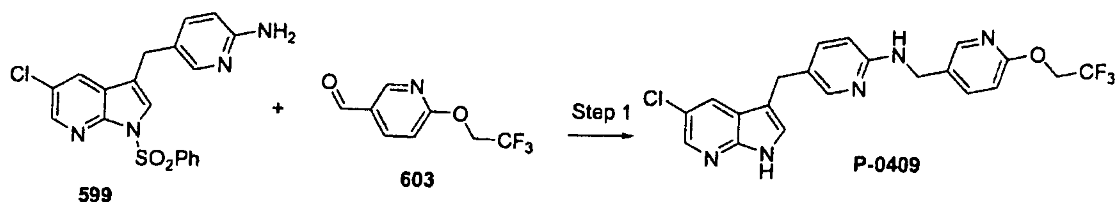
Scheme 188
