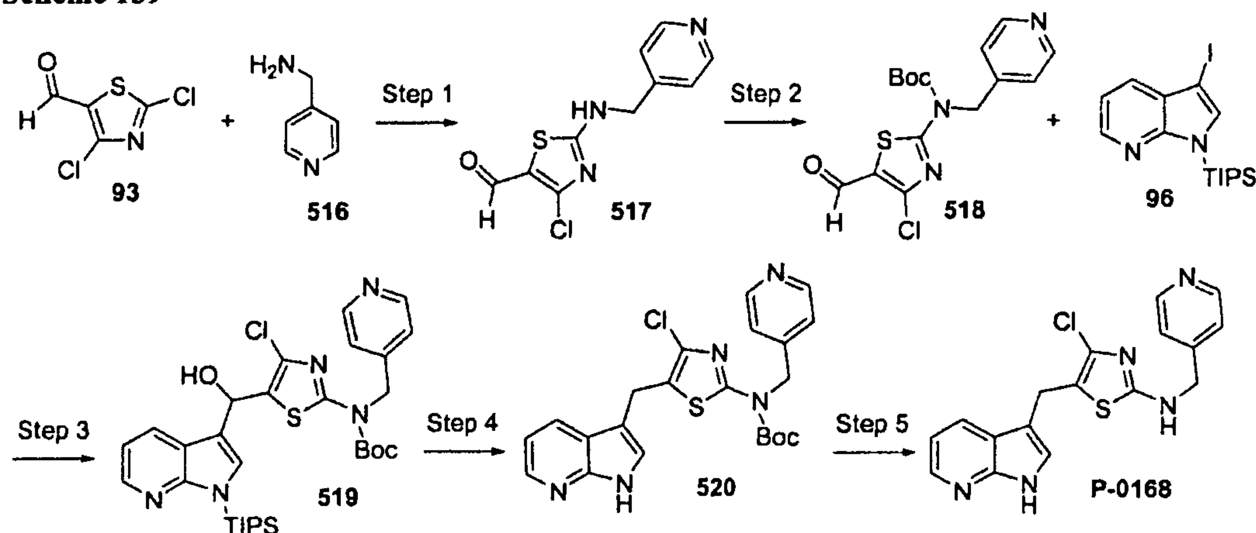
Scheme 159
