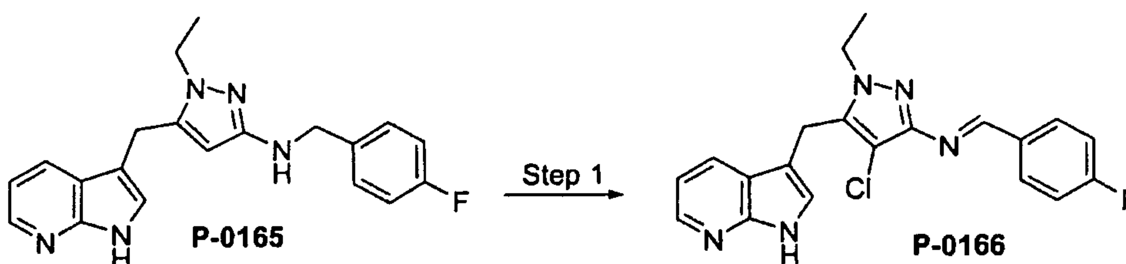
Scheme 163
