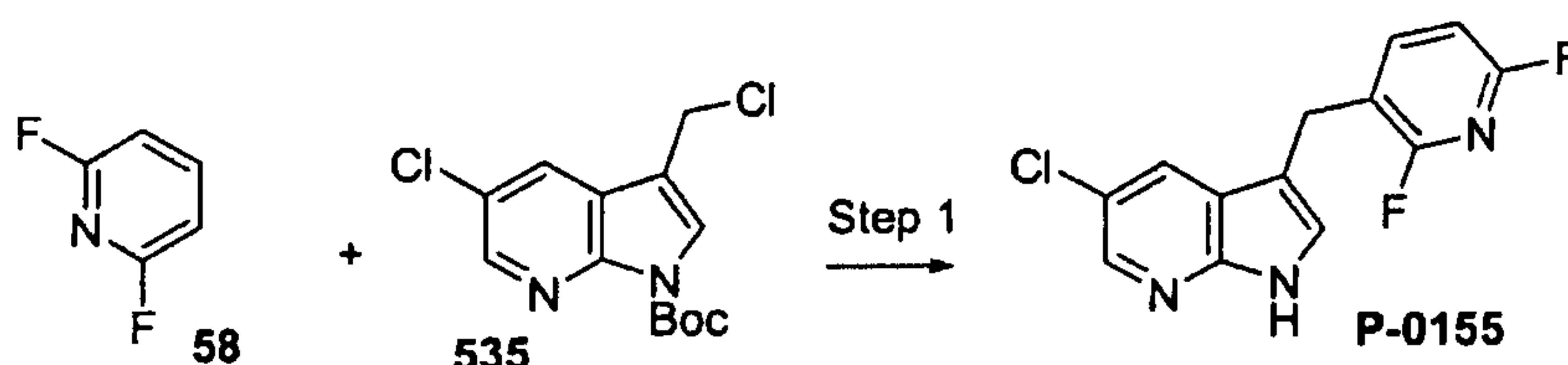
Scheme 166
