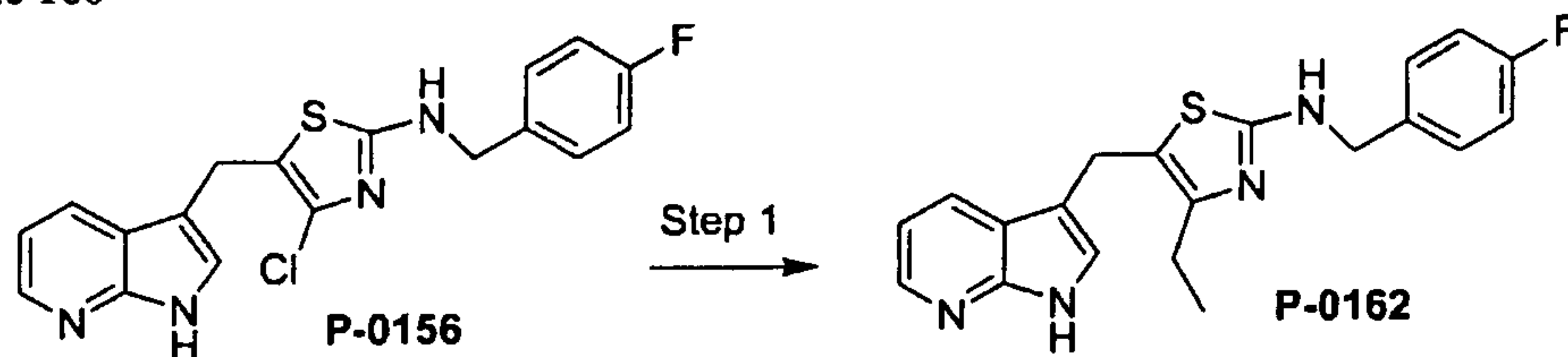
Scheme 160
