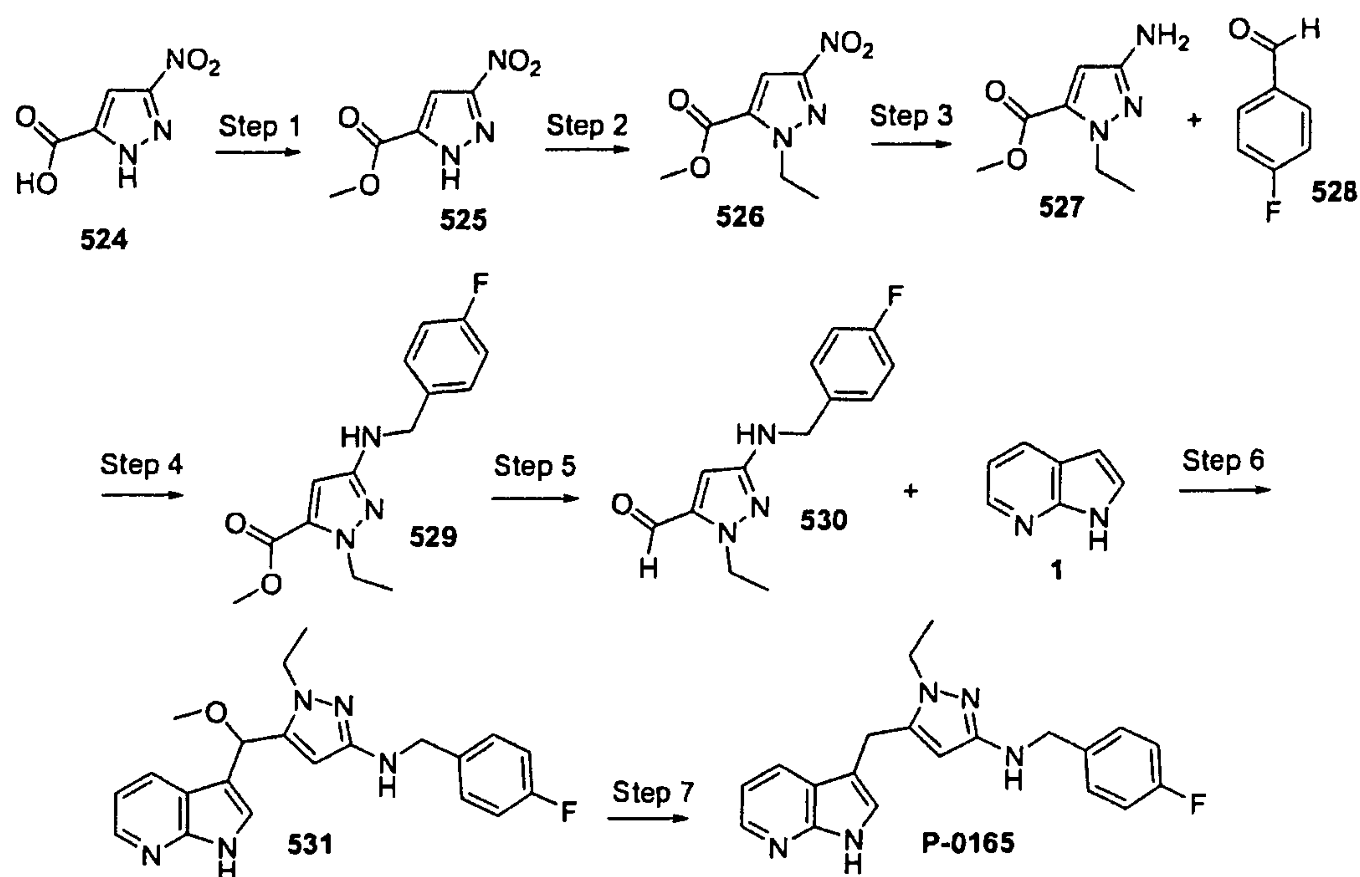
Scheme 162
