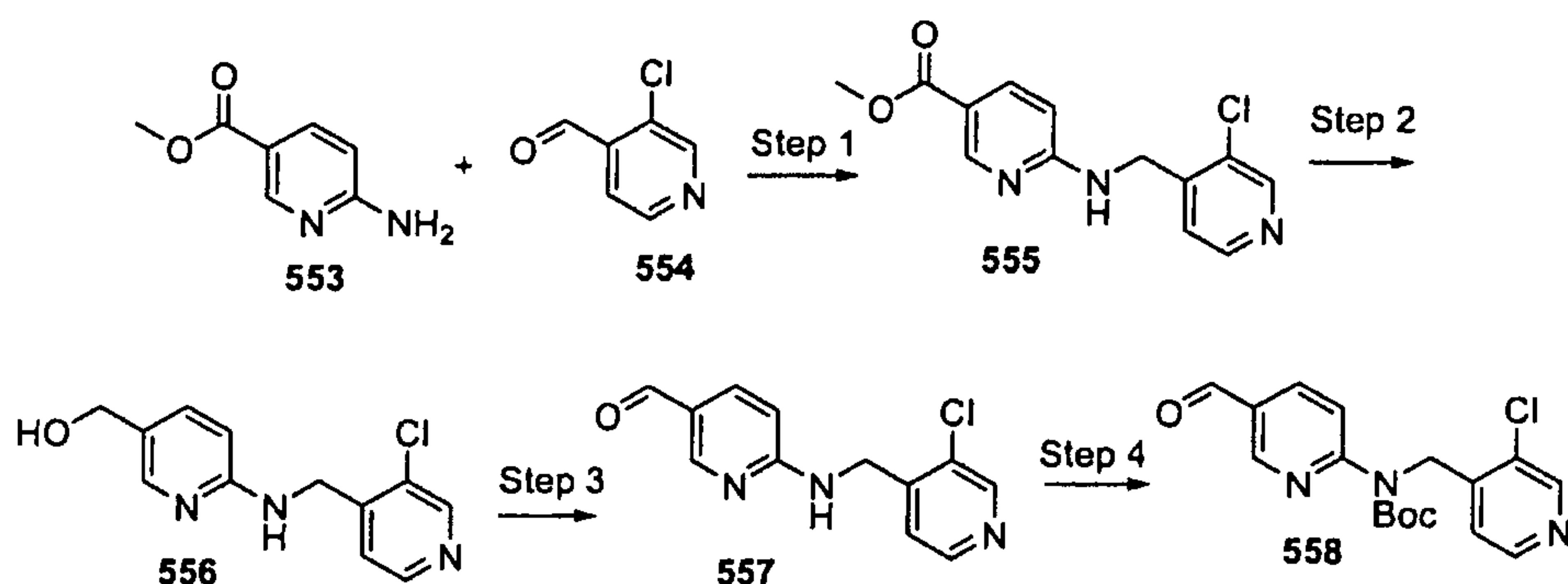
Scheme 175
