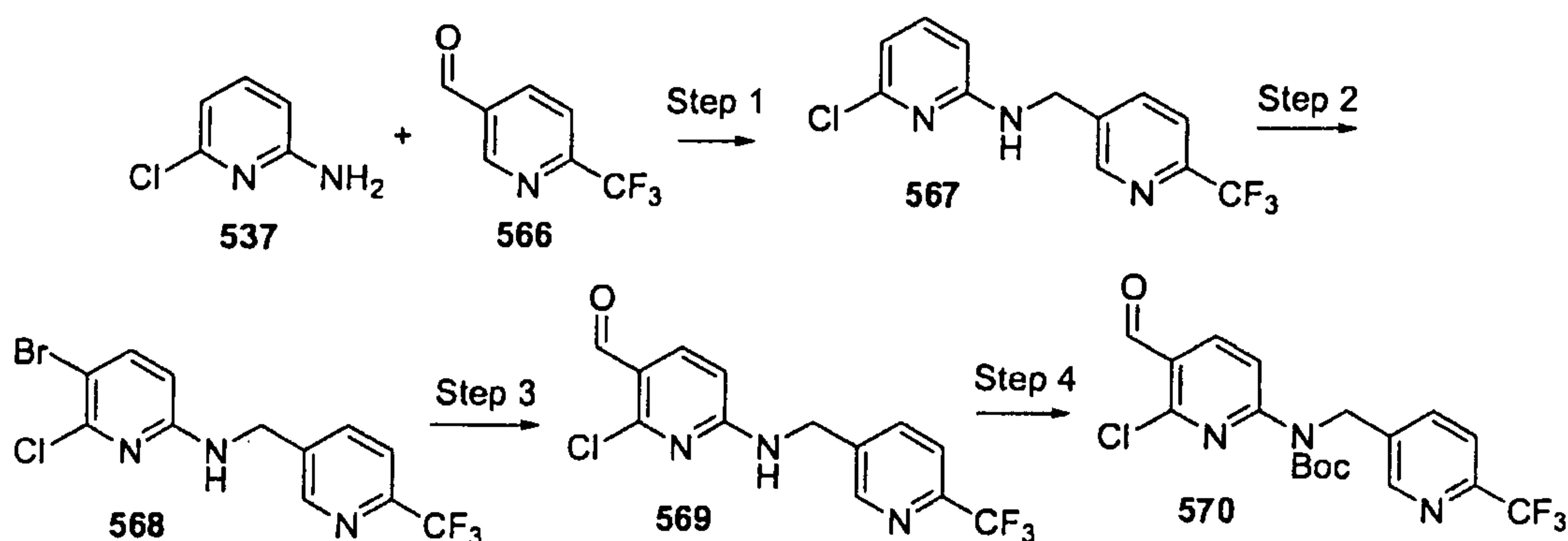
Scheme 177
