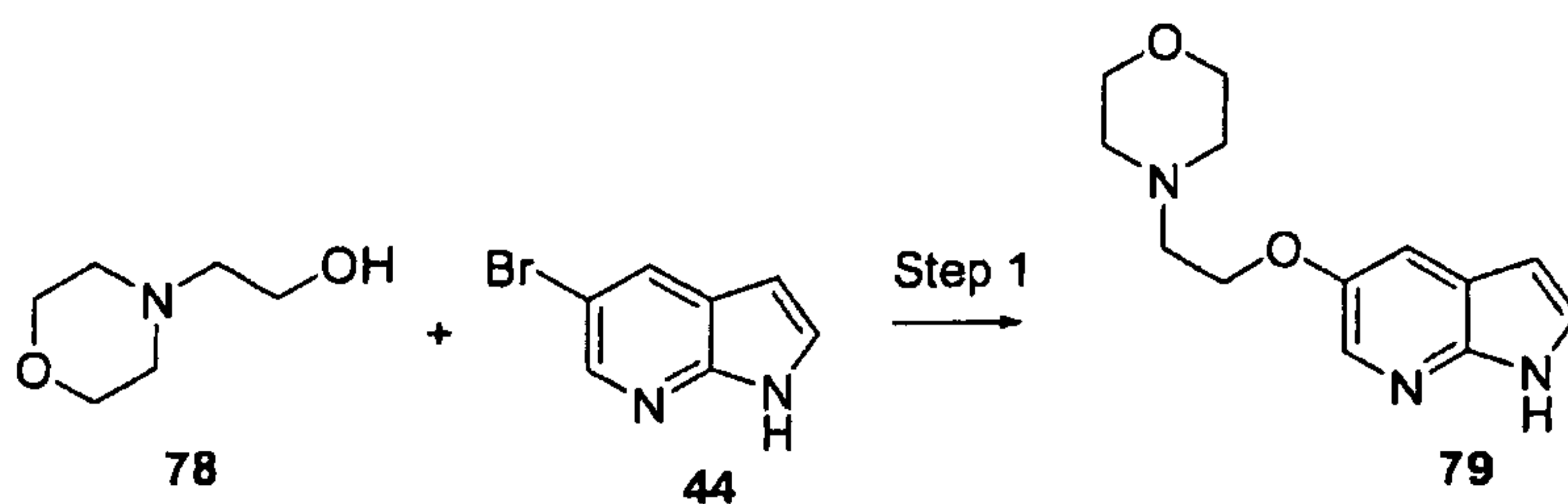
Scheme 31
