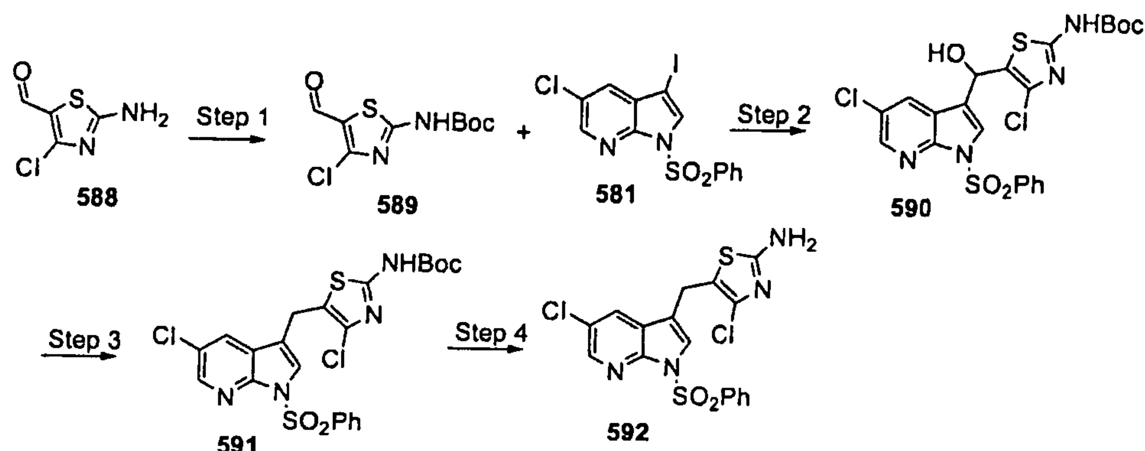
Scheme 183
