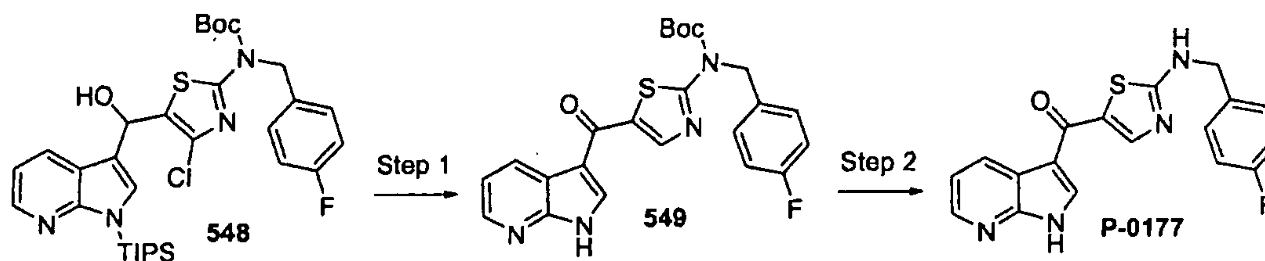
Scheme 173
