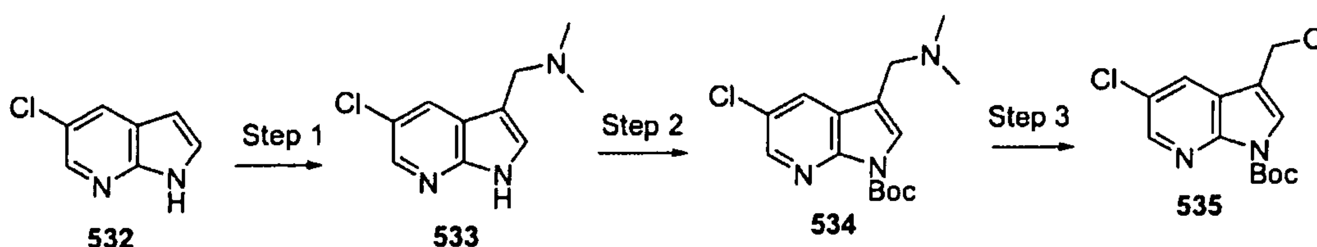
Scheme 164
