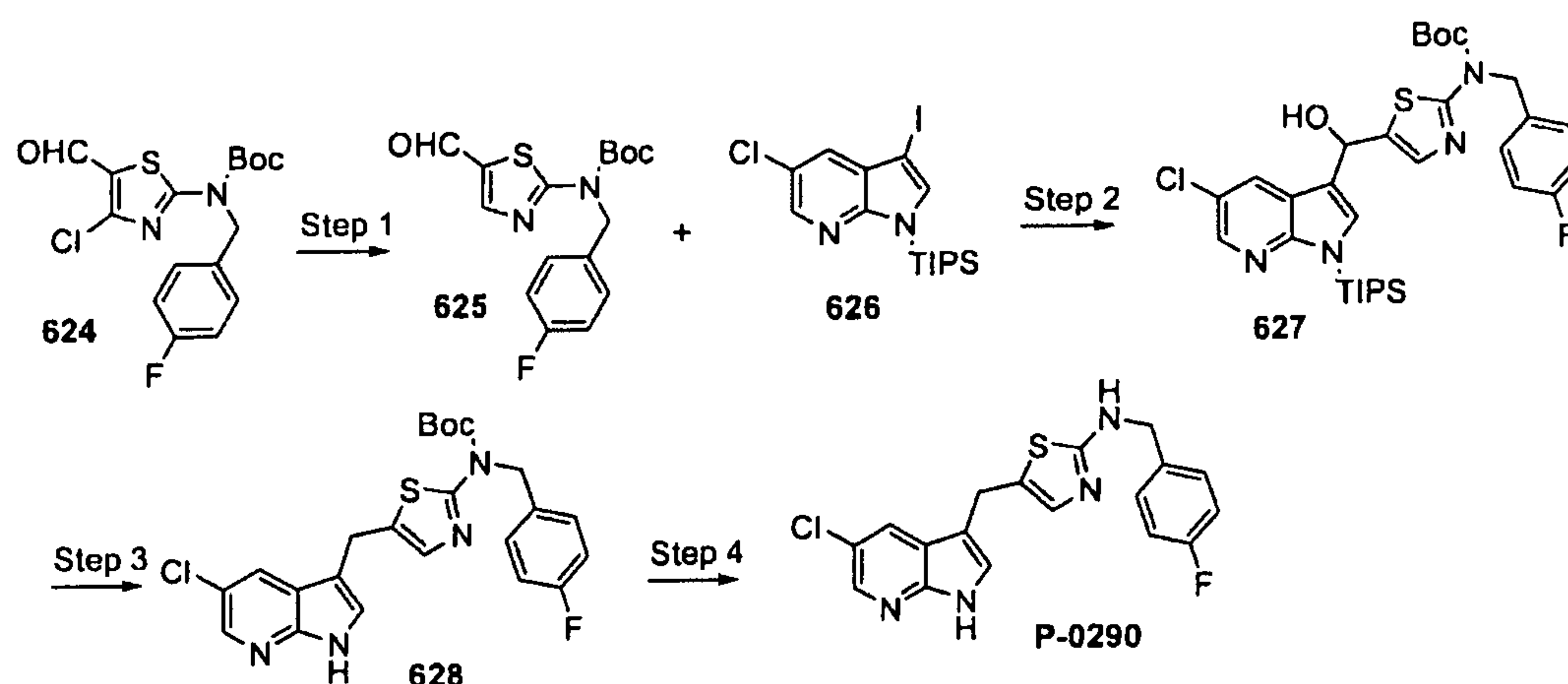
Scheme 198
