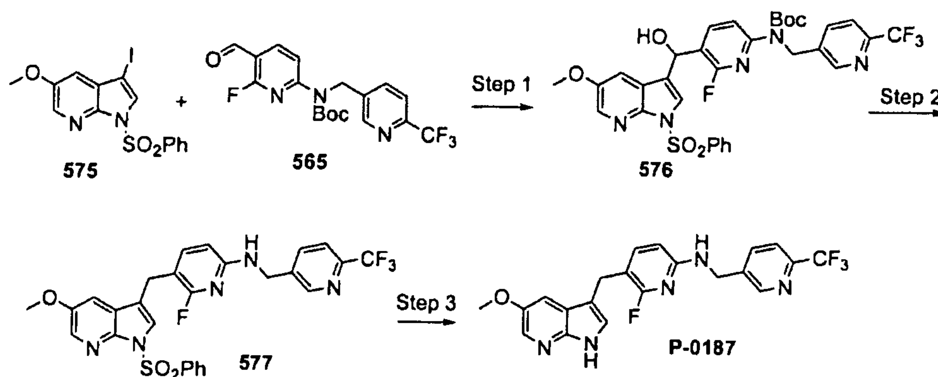
Scheme 179
