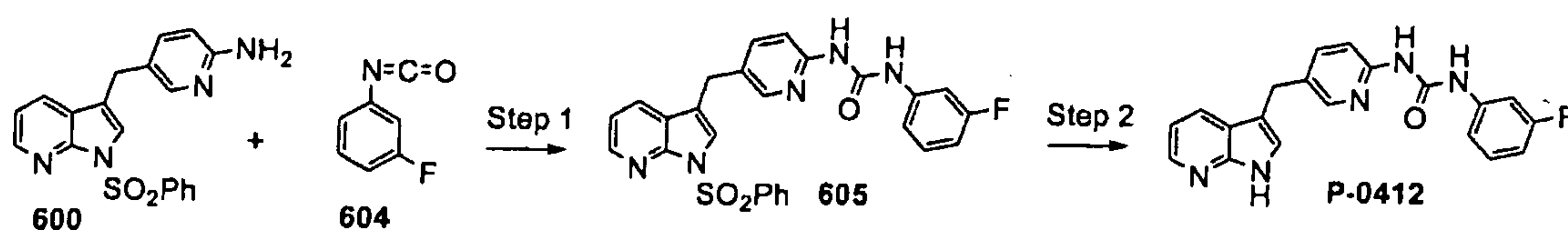
Scheme 189
