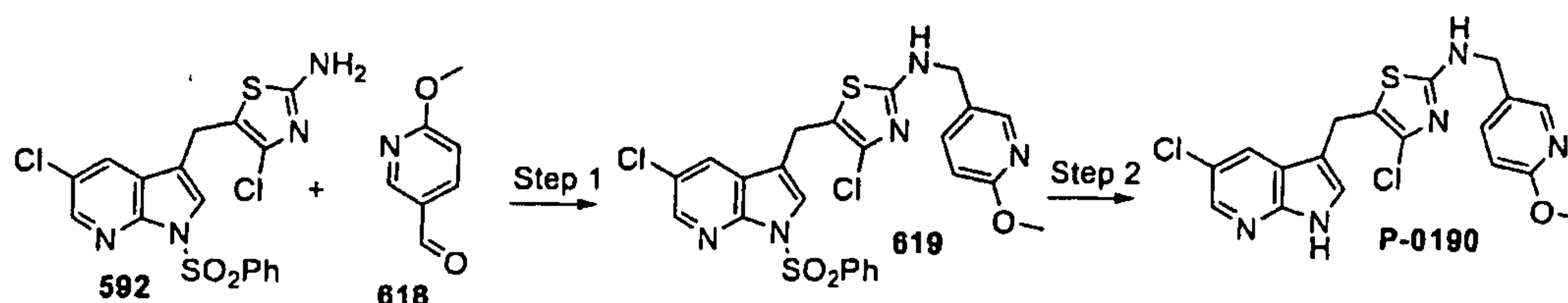
Scheme 196
