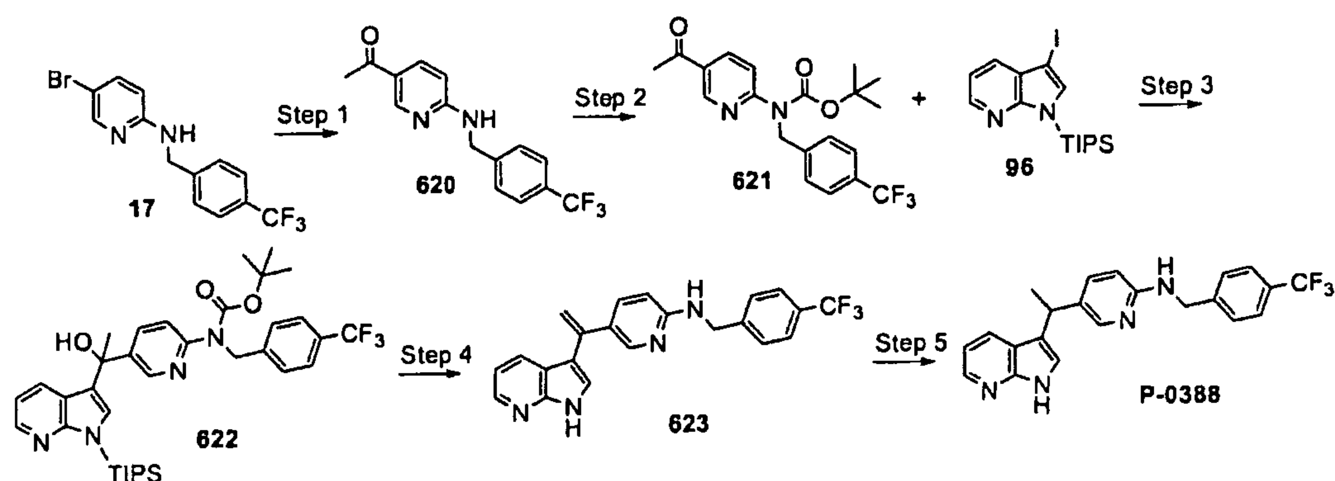
Scheme 197
