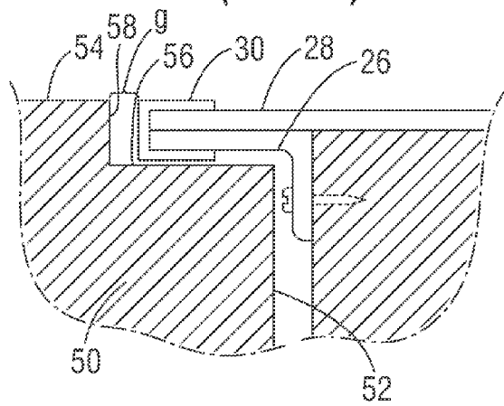
FIG. 5 (Prior Art)
