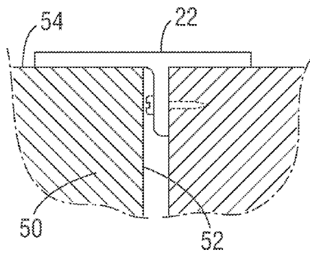
FIG. 4 (Prior Art)
