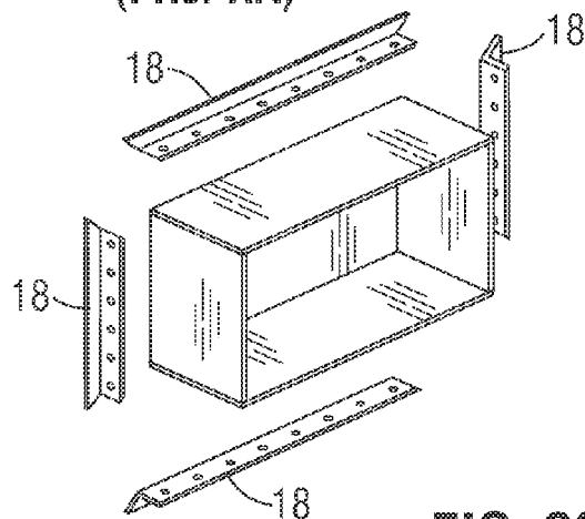
FIG. 2C (Prior Art)
