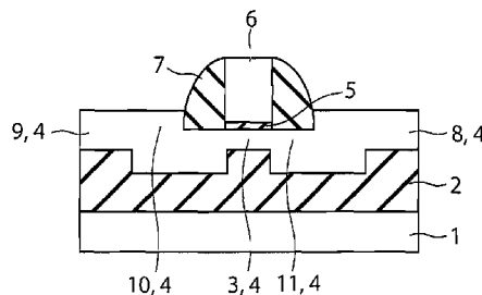
A-A CROSS-SECTION
