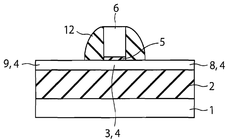
F-F CROSS-SECTION
