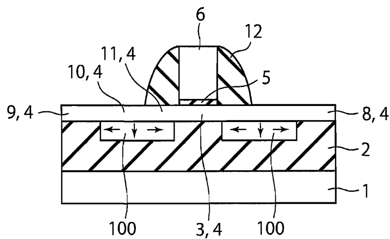
J-J CROSS-SECTION
