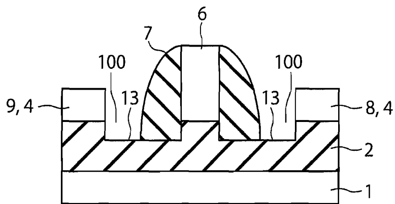
E-E CROSS-SECTION
