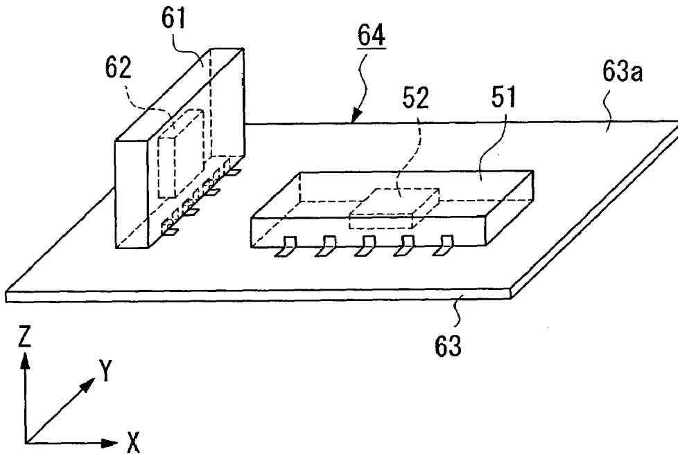
FIG. 83 (PRIOR ART)
