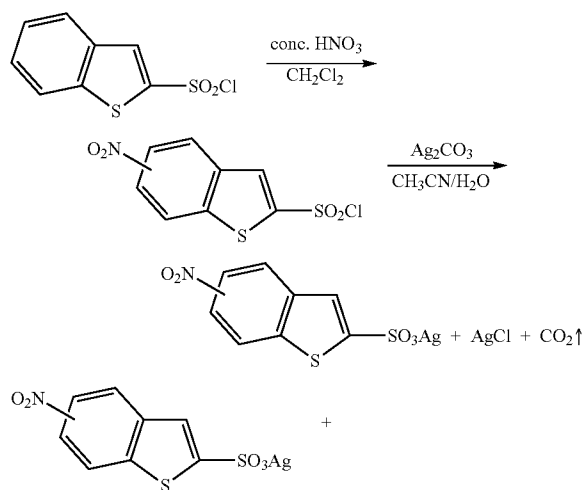
Scheme 1. Synthesis of fluorine-free fused-ring heteroaromatic PAGs.
