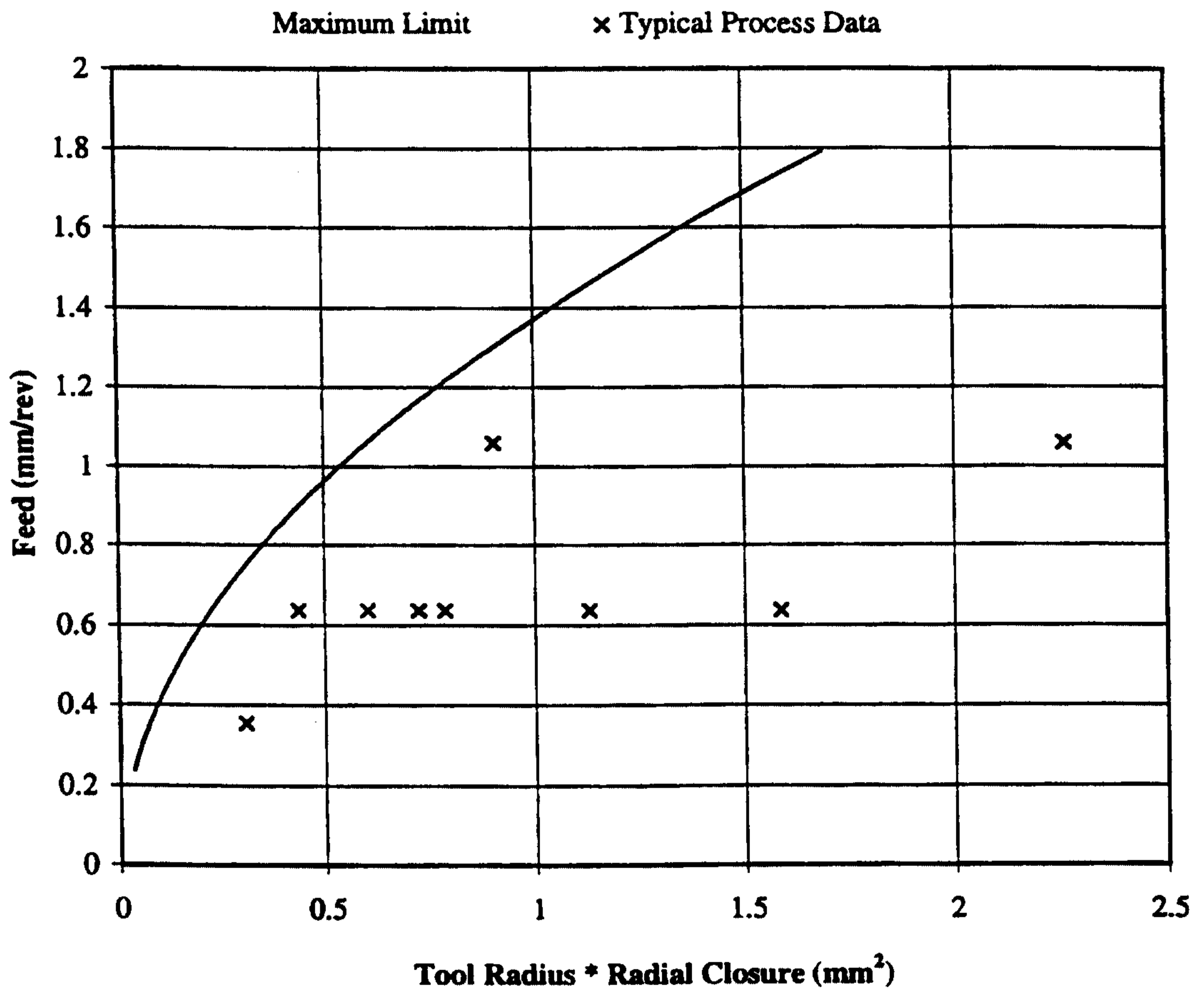
Figure 18: Point Contact Densification Limit Diagram
