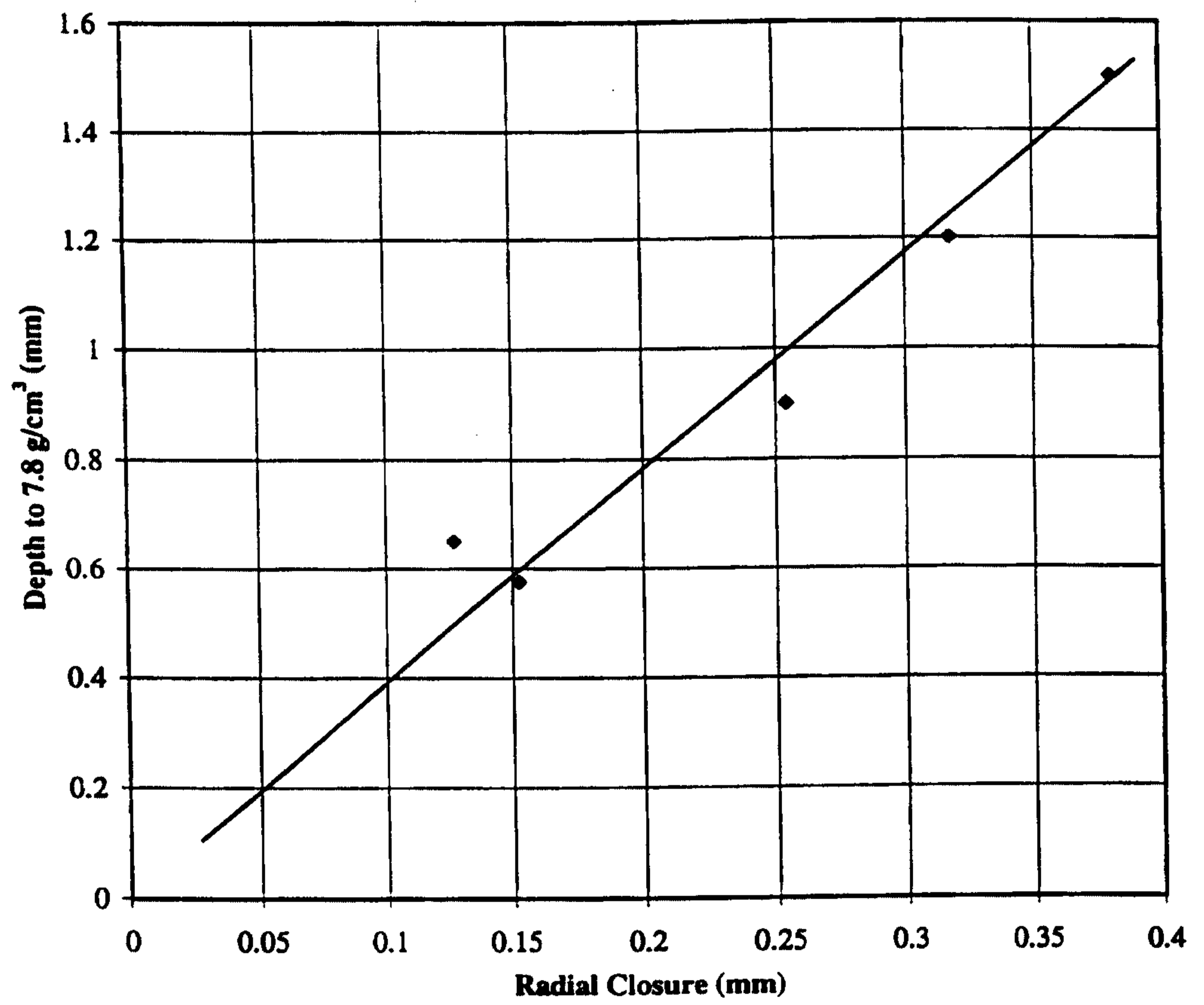
Figure 17: Typical Densification for 7.00 g/cm 3 Core Density
