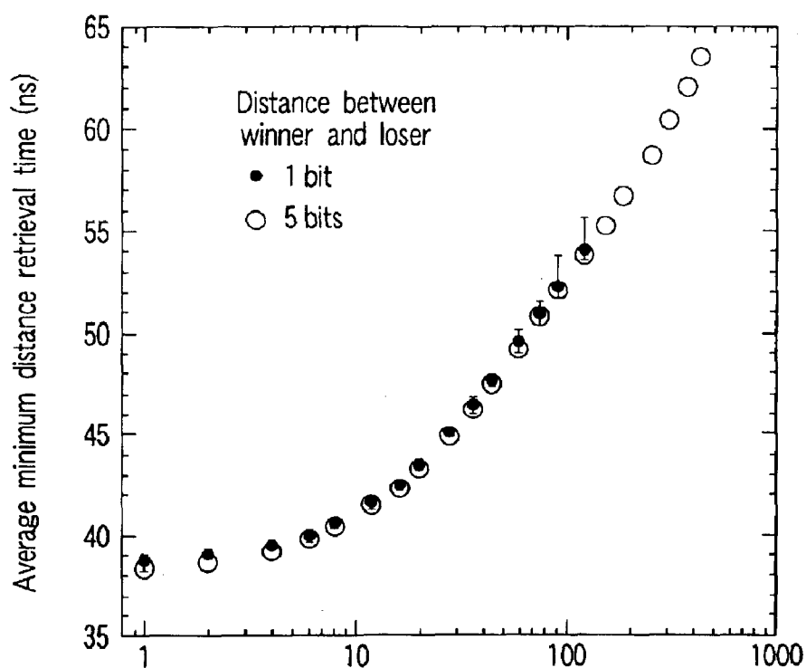
FIG. 7 Distance between winner and input (bit)
