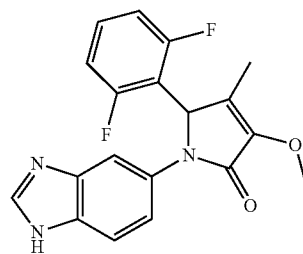
1-(1H-Benzo[d]imidazol-5-yl)-5-(2,6-difluorophenyl)-3-methoxy-4-methyl-1H-pyrrol-2(5H)-one;
