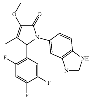
1-(1H-Benzo[d]imidazol-5-yl)-5-(2,4,5-trifluorophenyl)-3-methoxy-4-methyl-1H-pyrrol-2(5H)-one;
