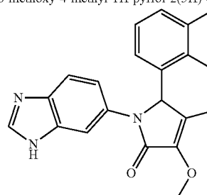
1-(1H-Benzo[d]imidazol-6-yl)-5-(2,3-difluorophenyl)-3-methoxy-4-methyl-1H-pyrrol-2(5H)-one;
