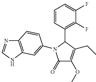
1-(1H-Benzo[d]imidazol-6-yl)-4-ethyl-5-(2,3-difluorophenyl)-3-methoxy-1H-pyrrol-2(5H)-one;
