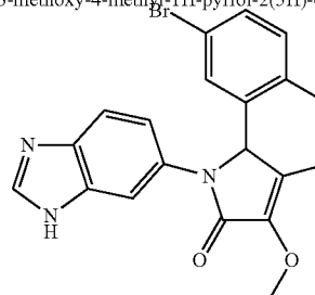
1-(1H-Benzo[d]imidazol-6-yl)-5-(5-bromo-2-fluorophenyl)-3-methoxy-4-methyl-1H-pyrrol-2(5H)-one;
