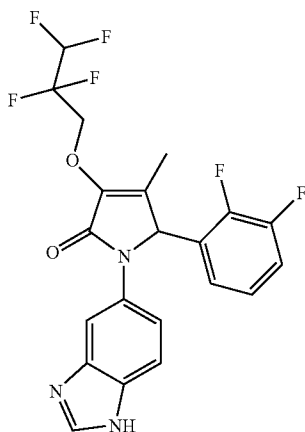
3-(2,2,3,3-Tetrafluoropropoxy)-1-(1H-benzo[d]imidazol-5-yl)-5-(2,3-difluorophenyl)-4-methyl-1H-pyrrol-2(5H)-one; and
