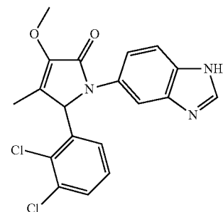
1-(1H-Benzo[d]imidazol-6-yl)-5-(2,3-dichlorophenyl)-3-methoxy-4-methyl-1H-pyrrol-2(5H)-one;
