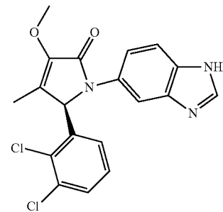
(R)-1-(1H-Benzo[d]imidazol-5-yl)-5-(2,3-dichlorophenyl)-3-methoxy-4-methyl-1H-pyrrol-2(5H)-one;
