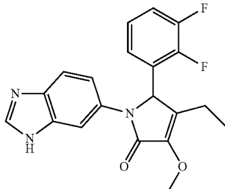
1-(1H-Benzo[d]imidazol-6-yl)-4-ethyl-5-(2,3-difluorophenyl)-3-methoxy-1H-pyrrol-2(5H)-one;
