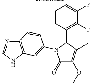
1-(1H-Benzo[d]imidazol-6-yl)-5-(2,3-difluorophenyl)-3-methoxy-4-methyl-1H-pyrrol-2(5H)-one;
