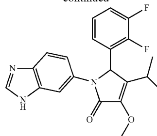
1-(1H-Benzo[d]imidazol-6-yl)-5-(2,3-difluorophenyl)-4-isopropyl-3-methoxy-1H-pyrrol-2(5H)-one;
