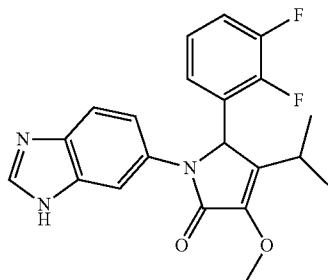
1-(1H-Benzo[d]imidazol-6-yl)-5-(2,3-difluorophenyl)-4-isopropyl-3-methoxy-1H-pyrrol-2(5H)-one;
