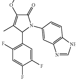
1-(1H-Benzo[d]imidazol-5-yl)-5-(2,4,5-trifluorophenyl)-3-methoxy-4-methyl-1H-pyrrol-2(5H)-one;
