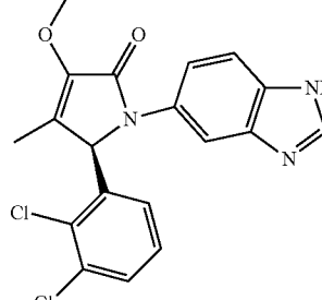
(R)-1-(1H-Benzo[d]imidazol-5-yl)-5-(2,3-dichlorophenyl)-3-methoxy-4-methyl-1H-pyrrol-2(5H)-one;
