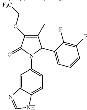
3-(2,2,2-Trifluoroethoxy)-1-(1H-benzo[d]imidazol-5-yl)-5-(2,3-difluorophenyl)-4-methyl-1H-pyrrol-2(5H)-one.
