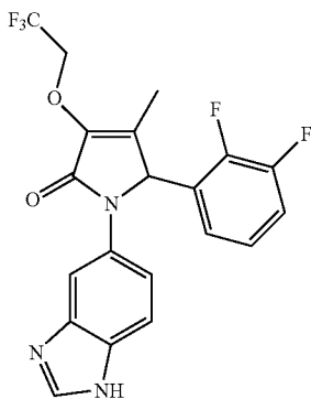
3-(2,2,2-Trifluoroethoxy)-1-(1H-benzo[d]imidazol-5-yl)-5-(2,3-difluorophenyl)-4-methyl-1H-pyrrol-2(5H)-one.
