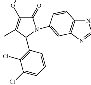
1-(1H-Benzo[d]imidazol-6-yl)-5-(2,3-dichlorophenyl)-3-methoxy-4-methyl-1H-pyrrol-2(5H)-one;
