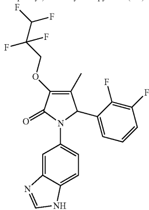
3-(2,2,3,3-Tetrafluoropropoxy)-1-(1H-benzo[d]imidazol-5-yl)-5-(2,3-difluorophenyl)-4-methyl-1H-pyrrol-2(5H)-one; and
