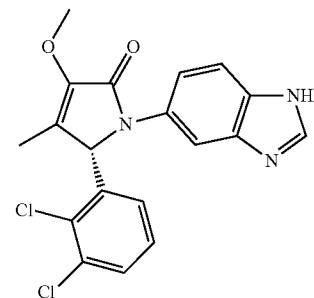
(S)-1-(1H-Benzo[d]imidazol-5-yl)-5-(2,3-dichlorophenyl)-3-methoxy-4-methyl-1H-pyrrol-2(5H)-one;
