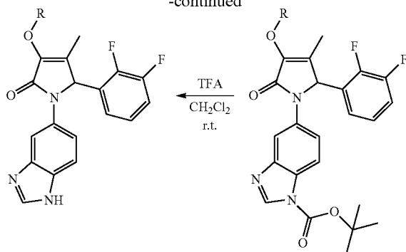
Tert-butyl 5-(2-(2,3-difluorophenyl)-4-hydroxy-3-methyl-5-oxo-2H-pyrrol-1(5H)-yl)-1H-benzo[d]imidazole-1-carboxylate
