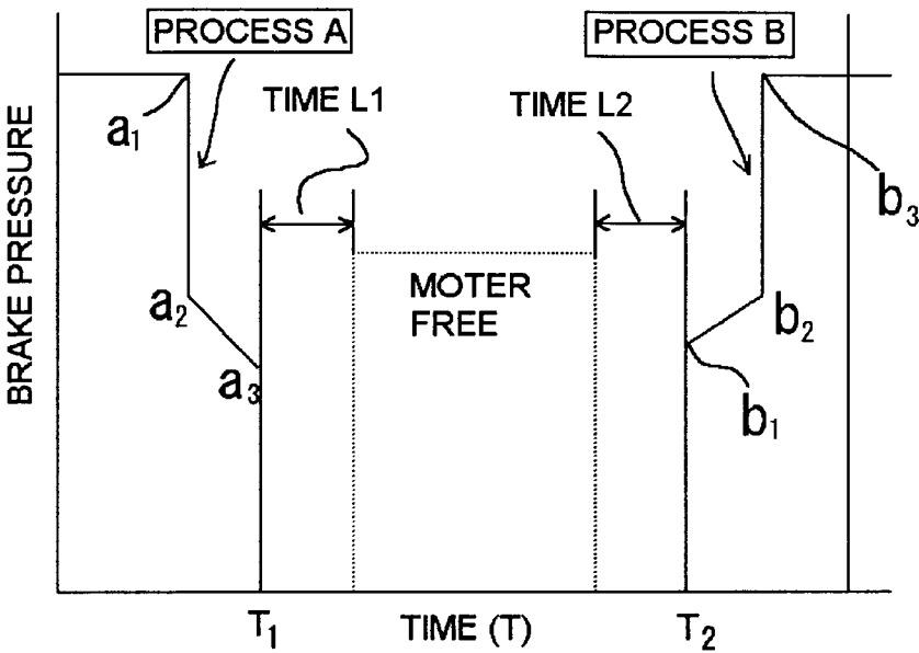
(b) CHARACTERISTIC GRAPH OF PIVOT TURN CONTROL
