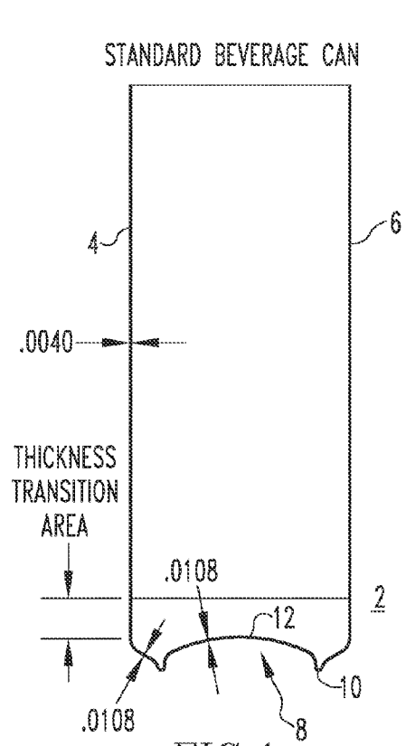
FIG. 1 PRIOR ART
