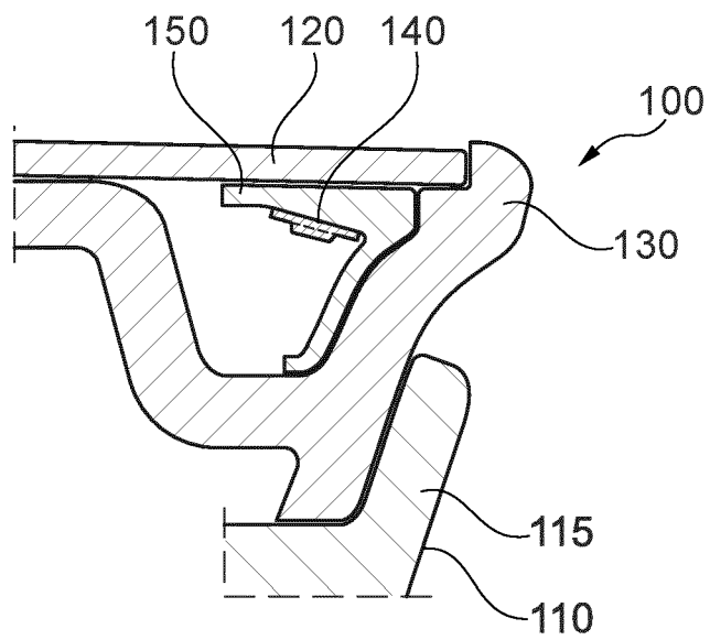
Section Cut A-A
