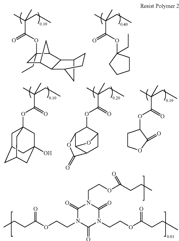
Synthesis Example 3
