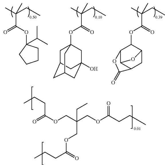
Resist Polymer 1
