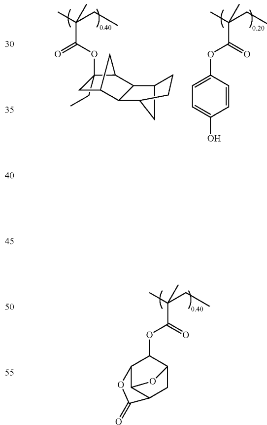
Comparative Resist Polymer 2
