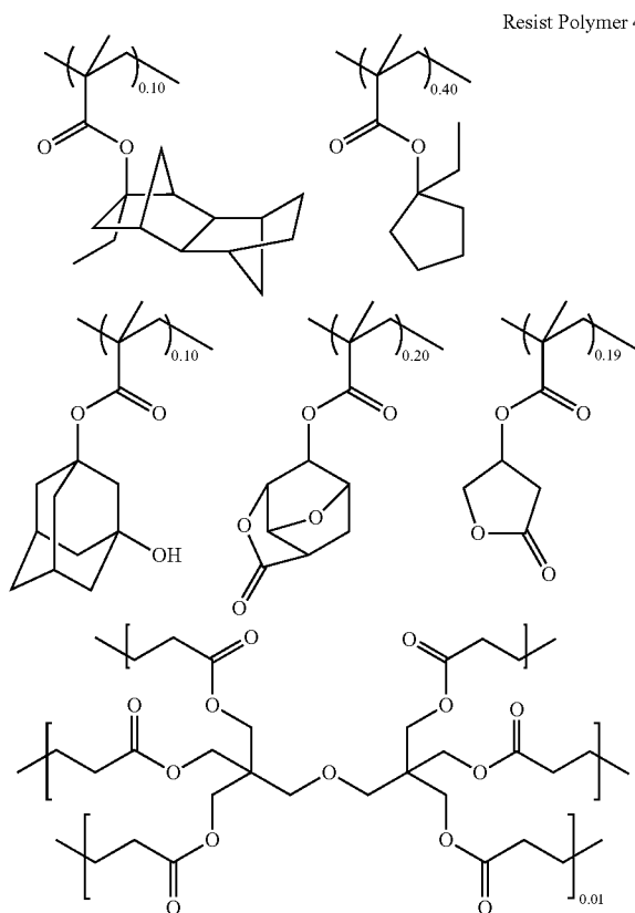
Synthesis Example 5
