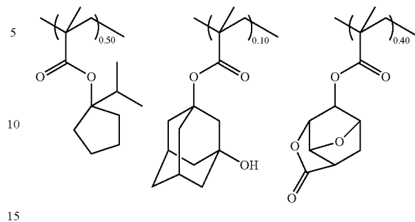
Comparative Resist Polymer 1
