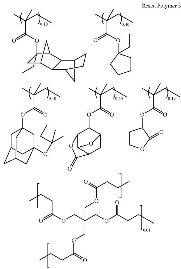
Synthesis Example 4
