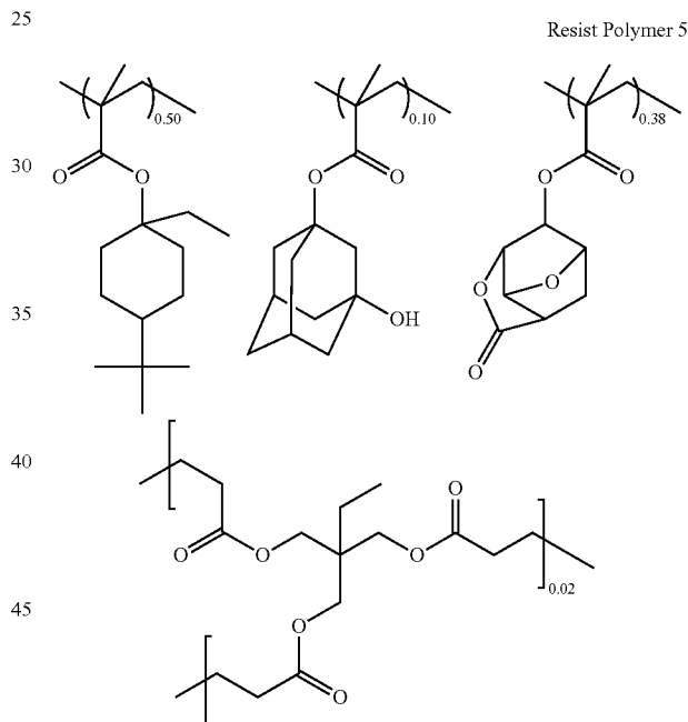
Synthesis Example 6
