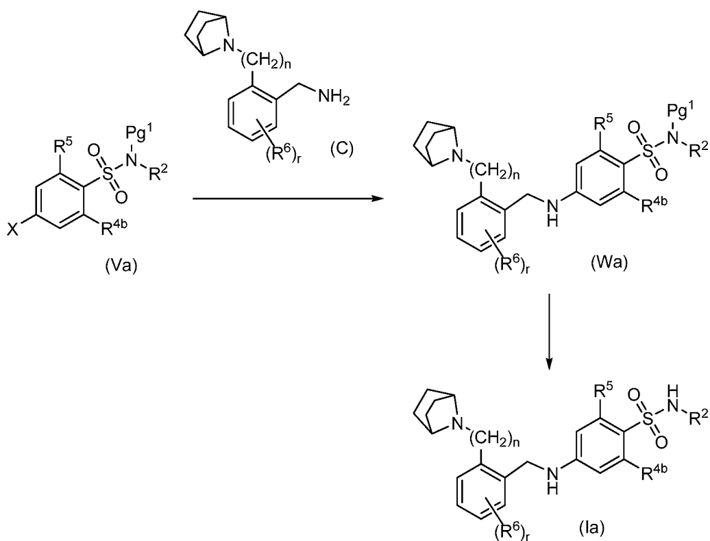
REACTION SCHEME 6
