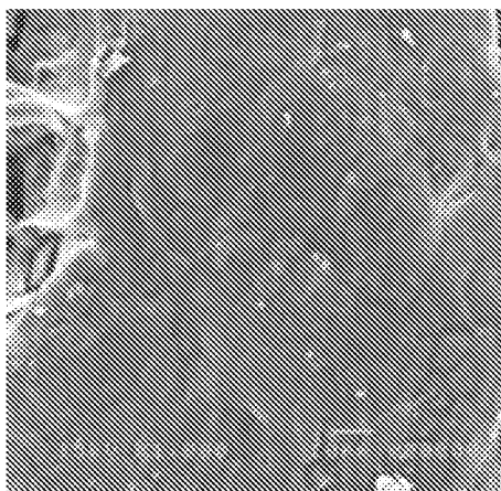
CRANBERRY + E.coli 10000X
