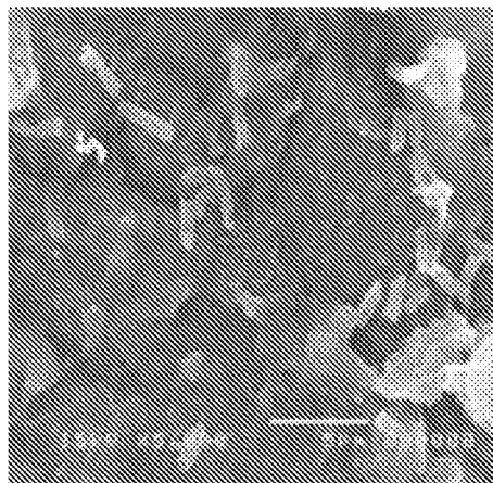
CRANBERRY + E.coli 5000X
