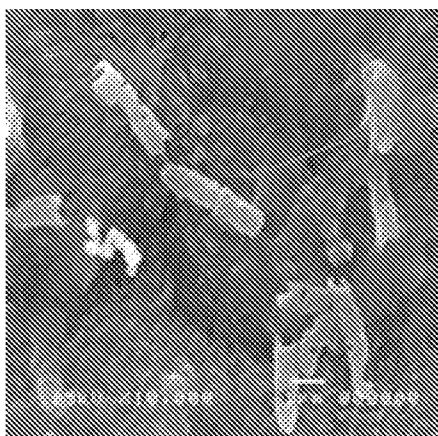
CRANBERRY + E.coli 10000X
