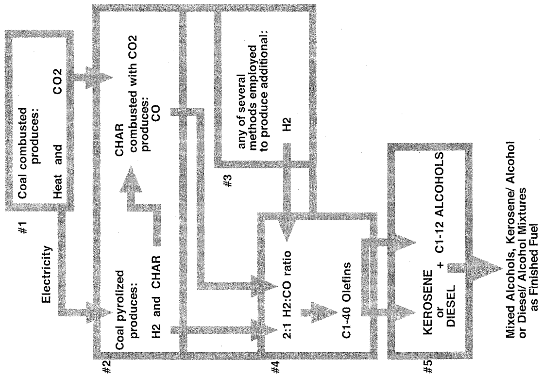
FIG. 1 (PRIOR ART)
