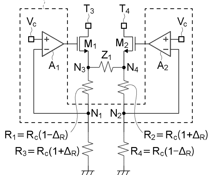
CONTROL CIRCUIT
