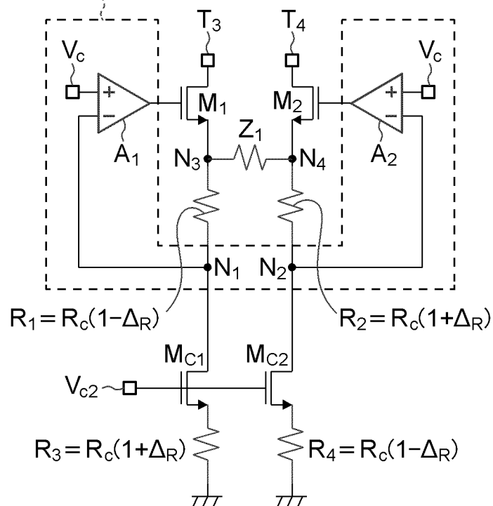
CONTROL CIRCUIT
