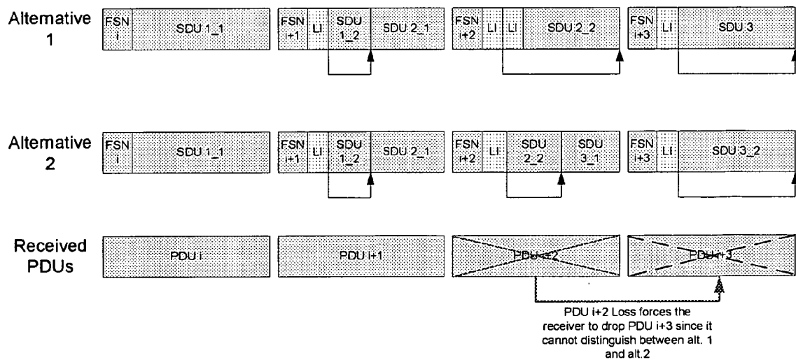
Figure 8 - Error propagation in UMTS R99
