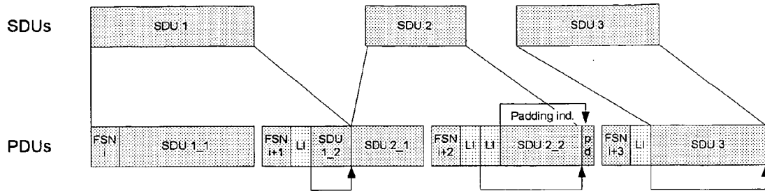
Figure 5 - SAR signaling with length indicators
