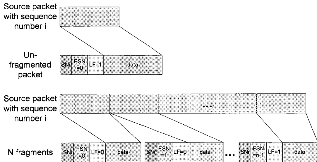
Figure 3 - SAR signaling by fragment numbering
