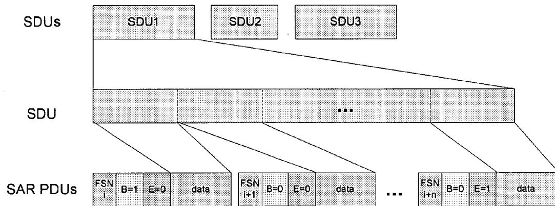
Figure 4 - SAR signaling with Beginning and End flags
