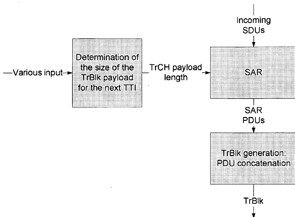
Figure 9 - Proposed SAR and concatenation processes
