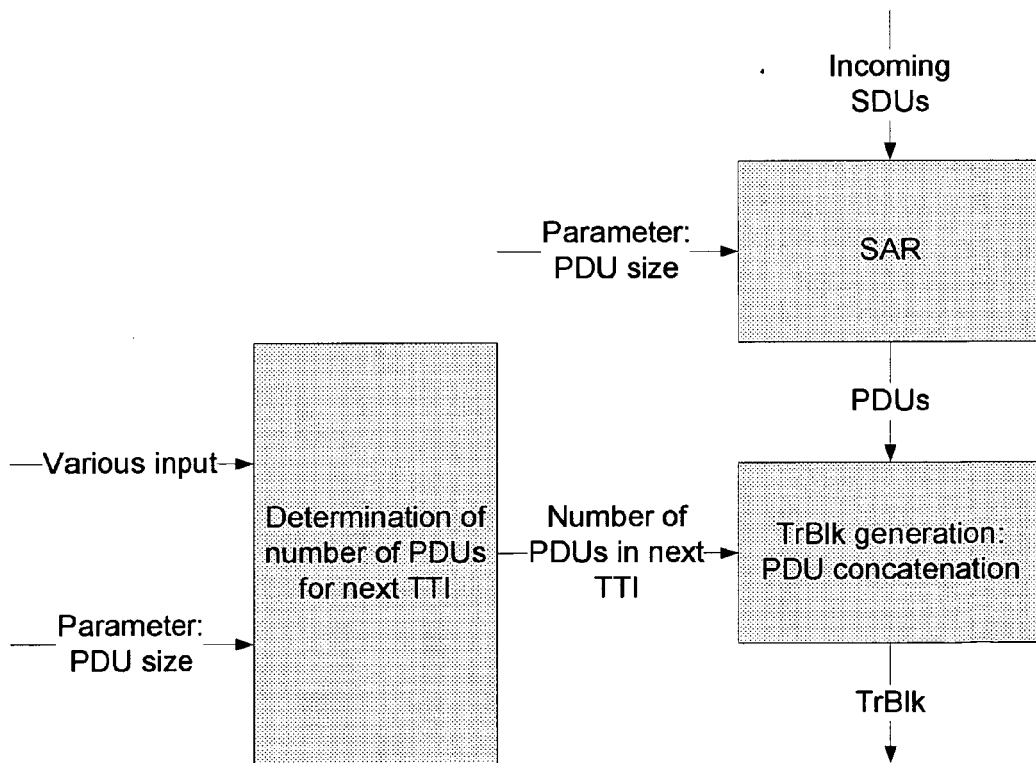
Figure 6 - SDU Segmentation and PDU concatenation Processes
