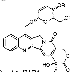
R = Ac, HAR4 R = OH, HAR7
