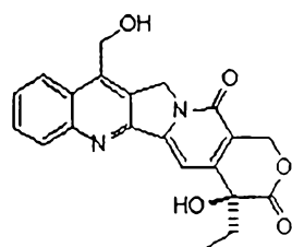
7-hydroxymethyl camptothecin HAR8
