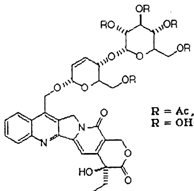
7-hydroxymethyl camptothecin HAR8
