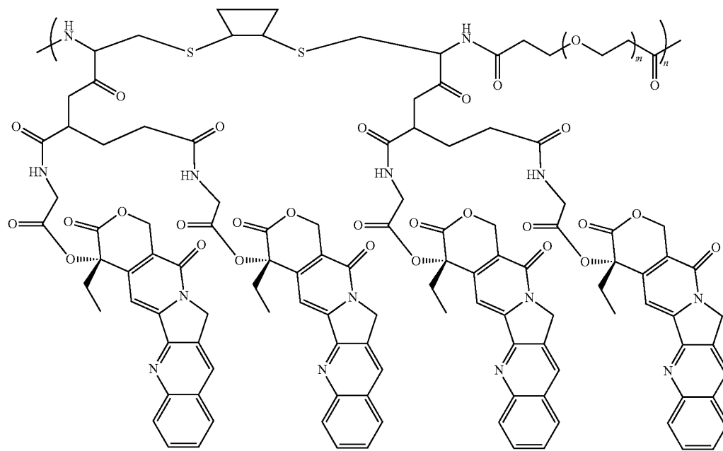
43 PEG Mw = 3400 4 CPT per CD Maximum drug loading 25%
