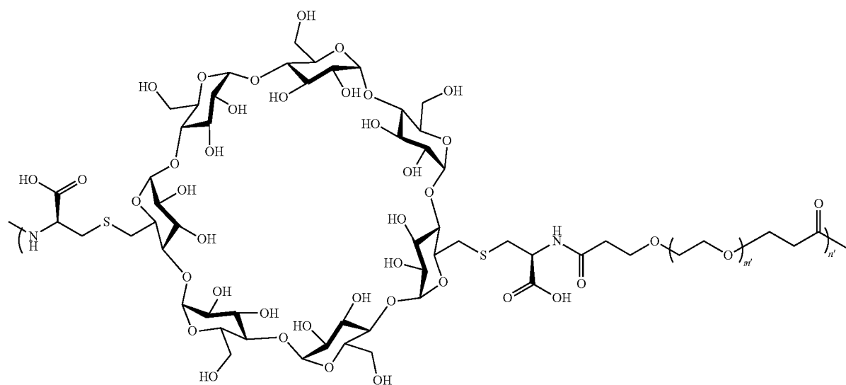
36a-f Poly(CDDCCys-PA-PEG) Abbr: PA = propanoicamide bond between PEG and CD
