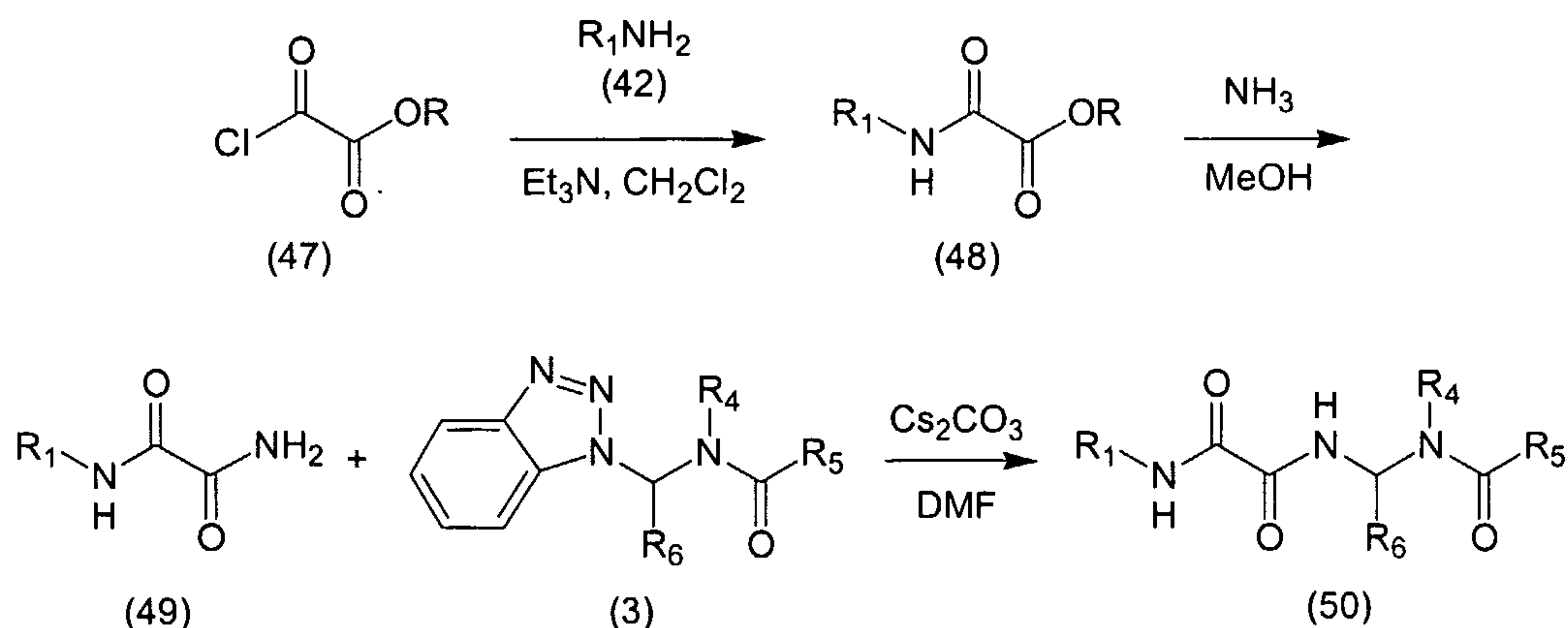
Scheme 13
