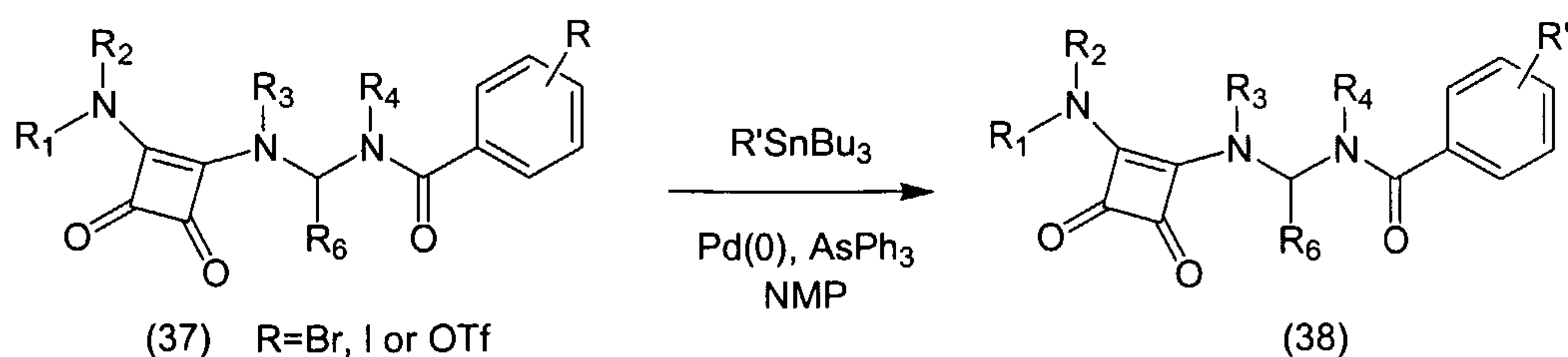
Scheme 10
