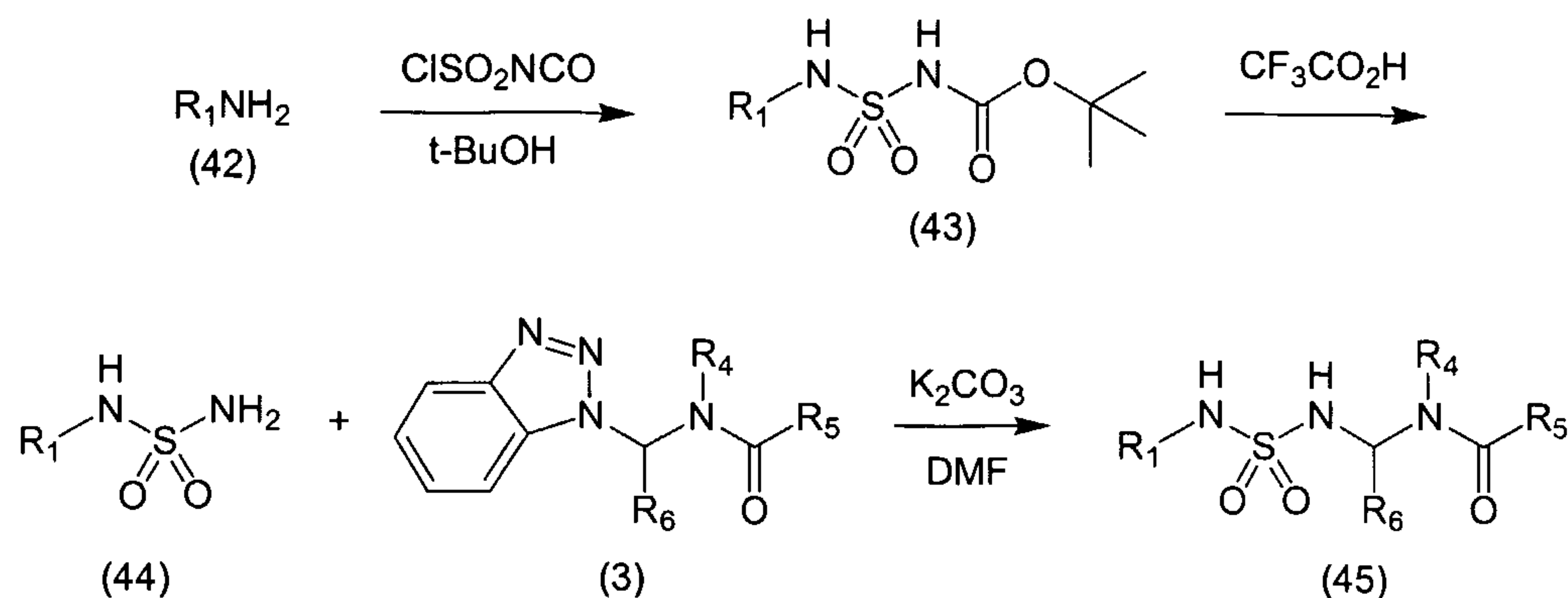
Scheme 12
