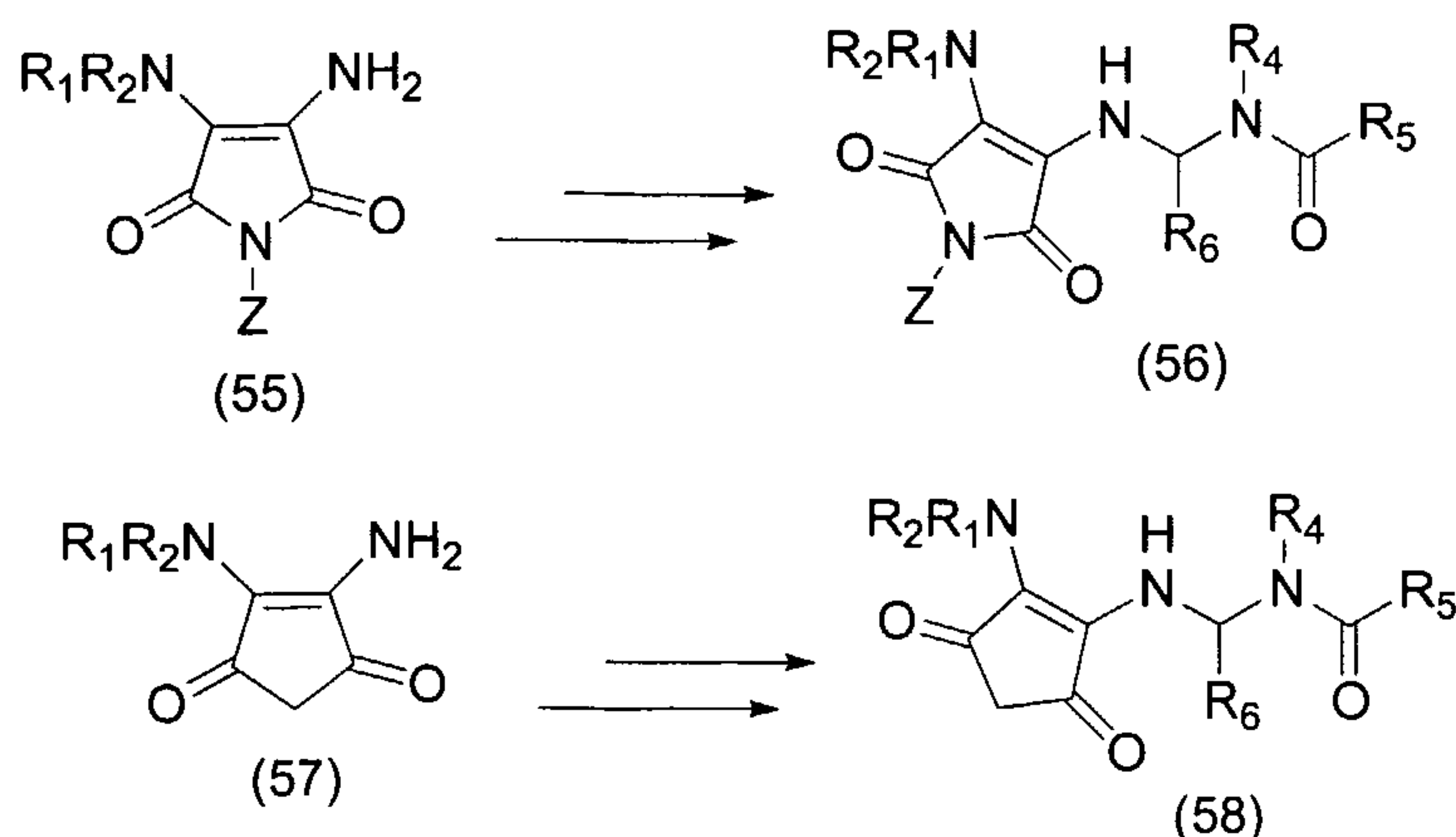
Scheme 15
