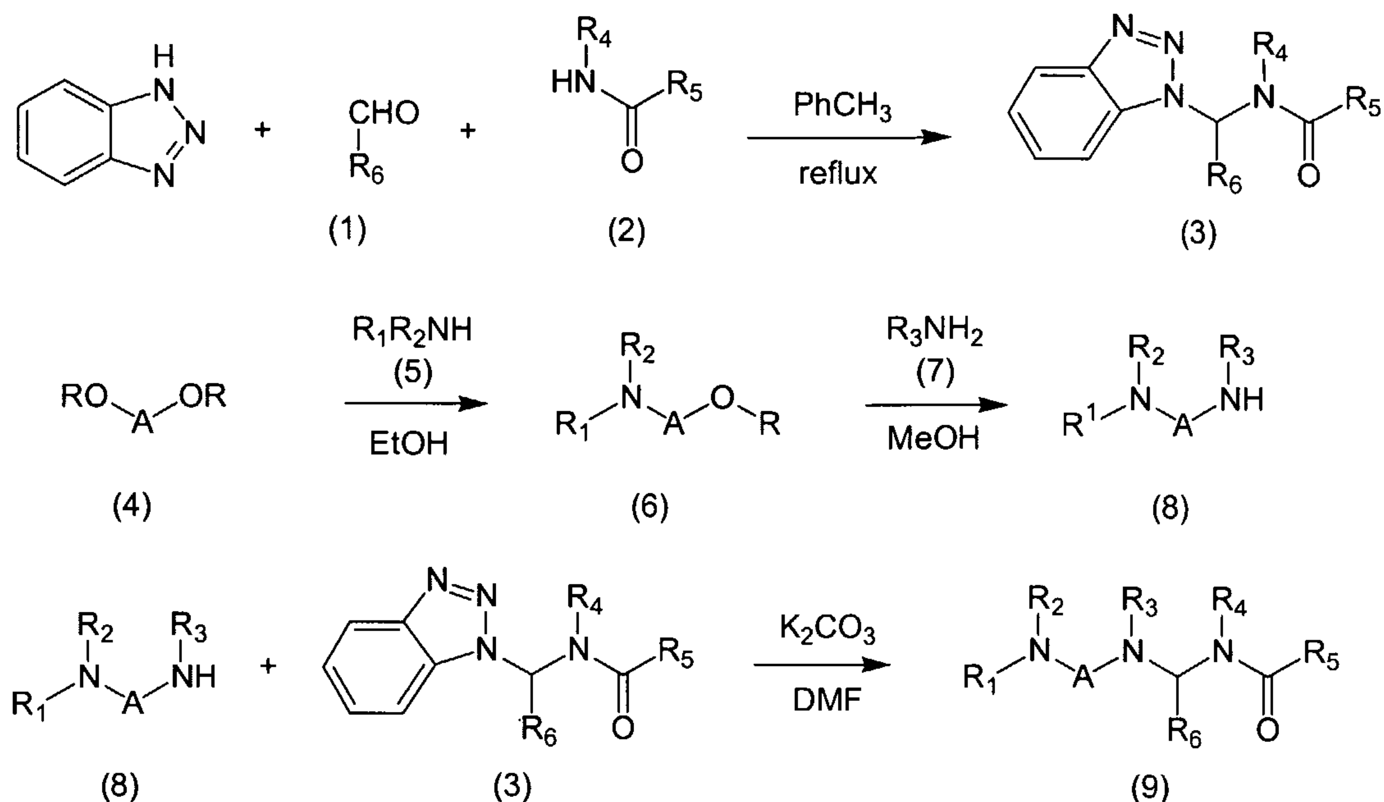
Scheme 1
