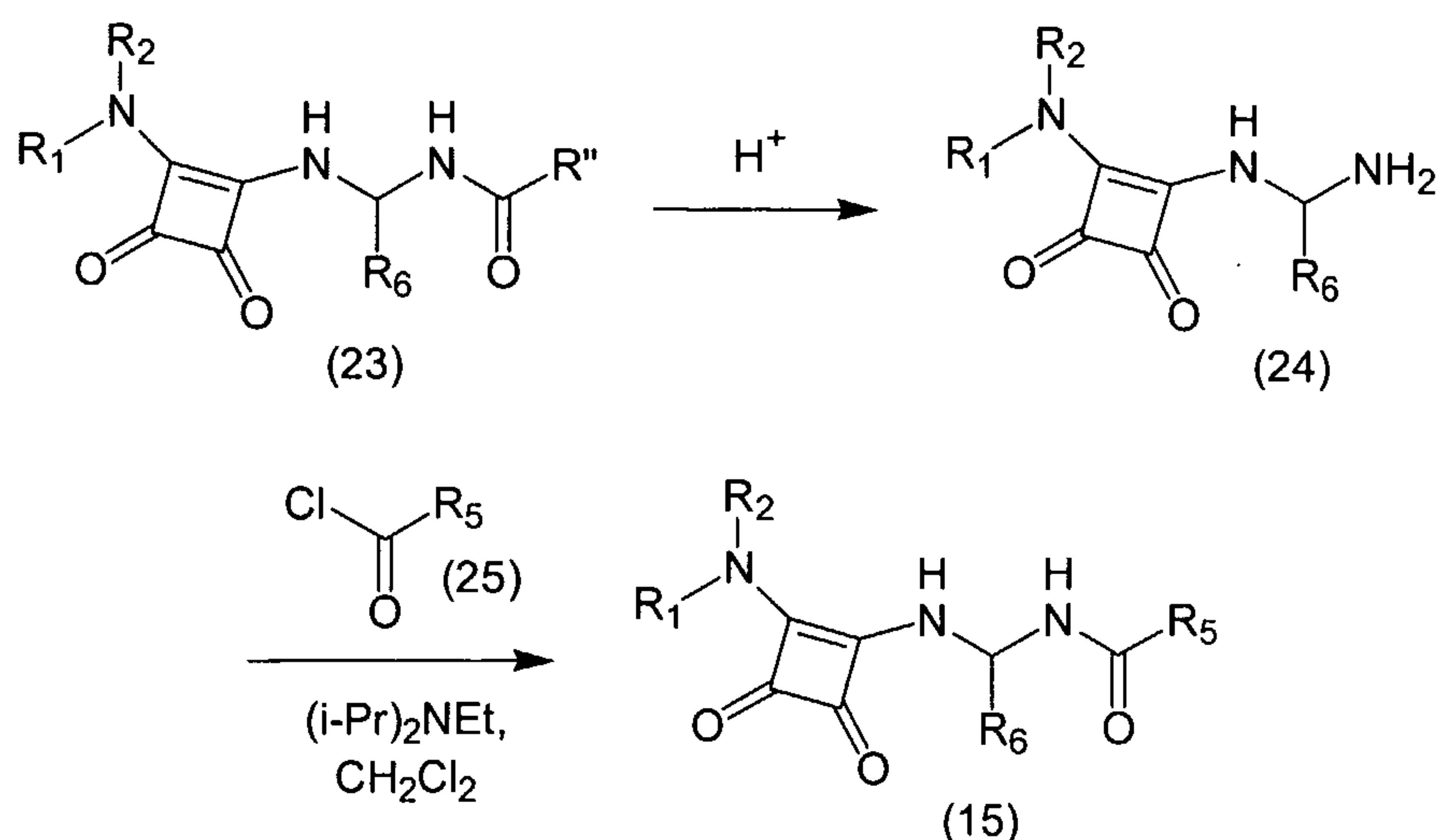
Scheme 5
