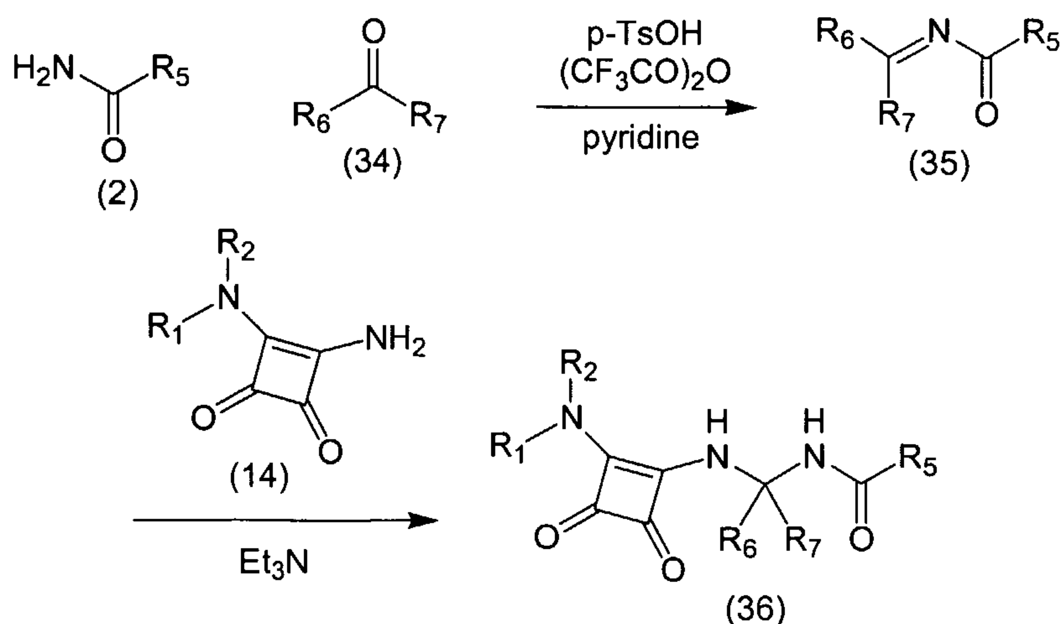
Scheme 9
