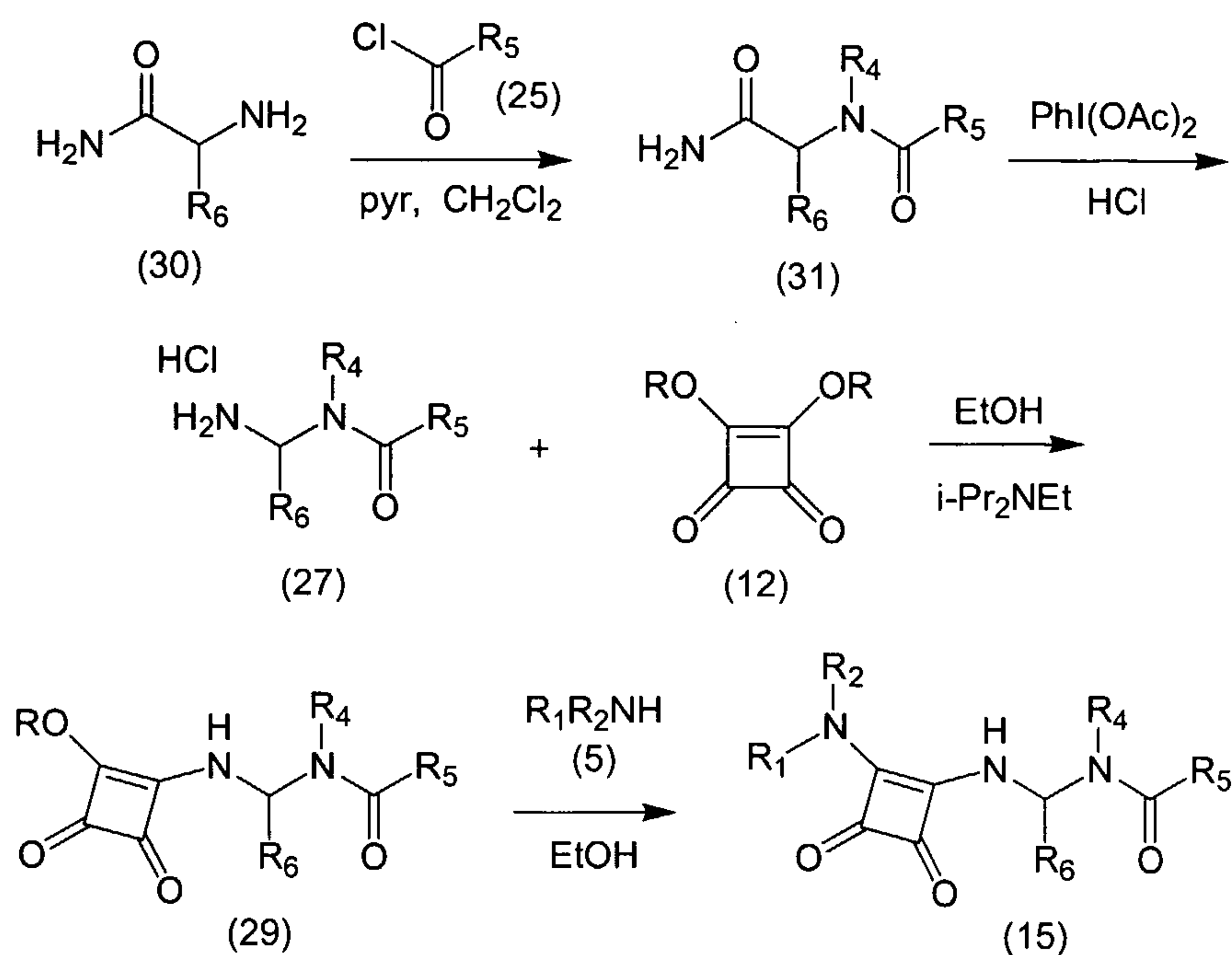
Scheme 8
