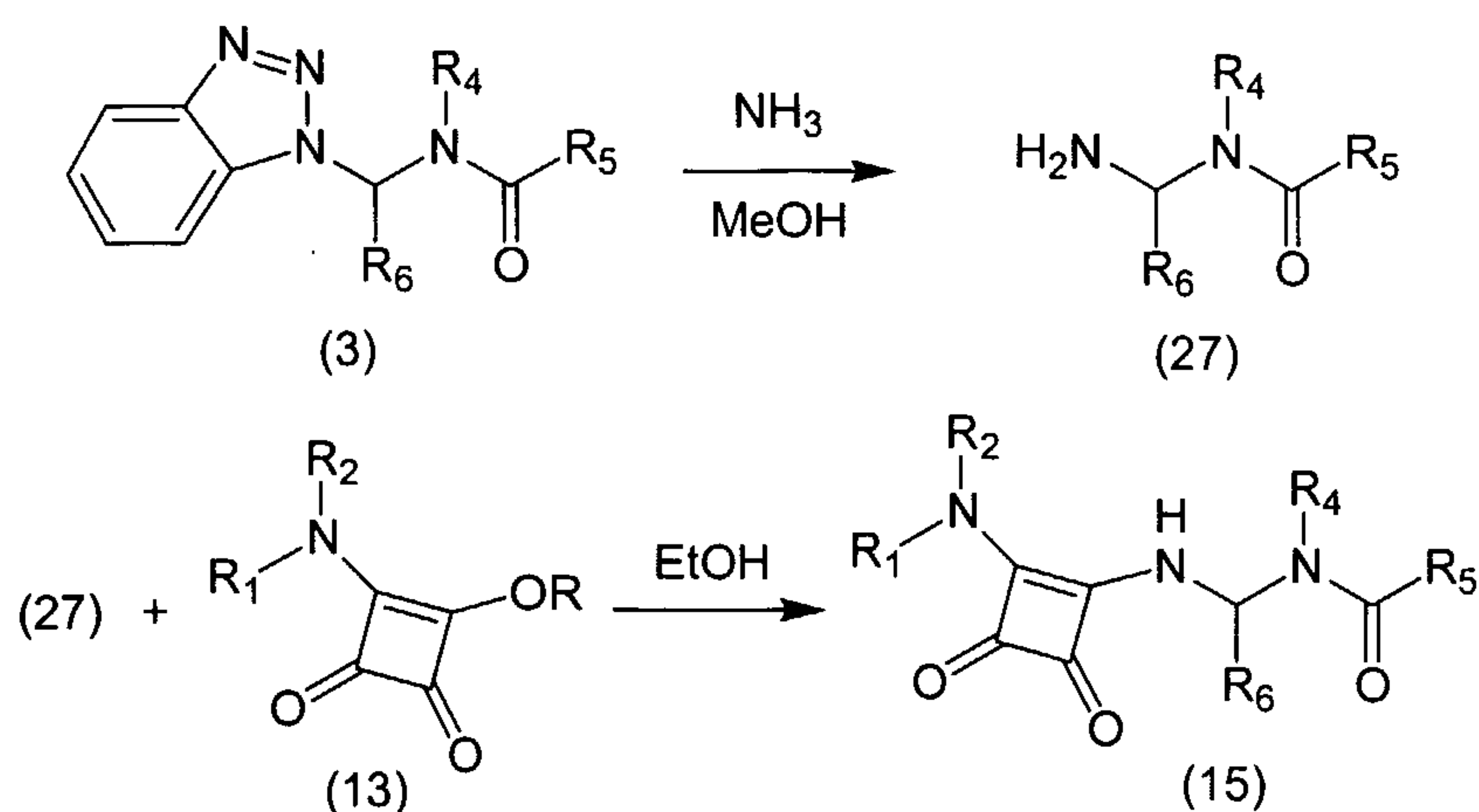
Scheme 6
