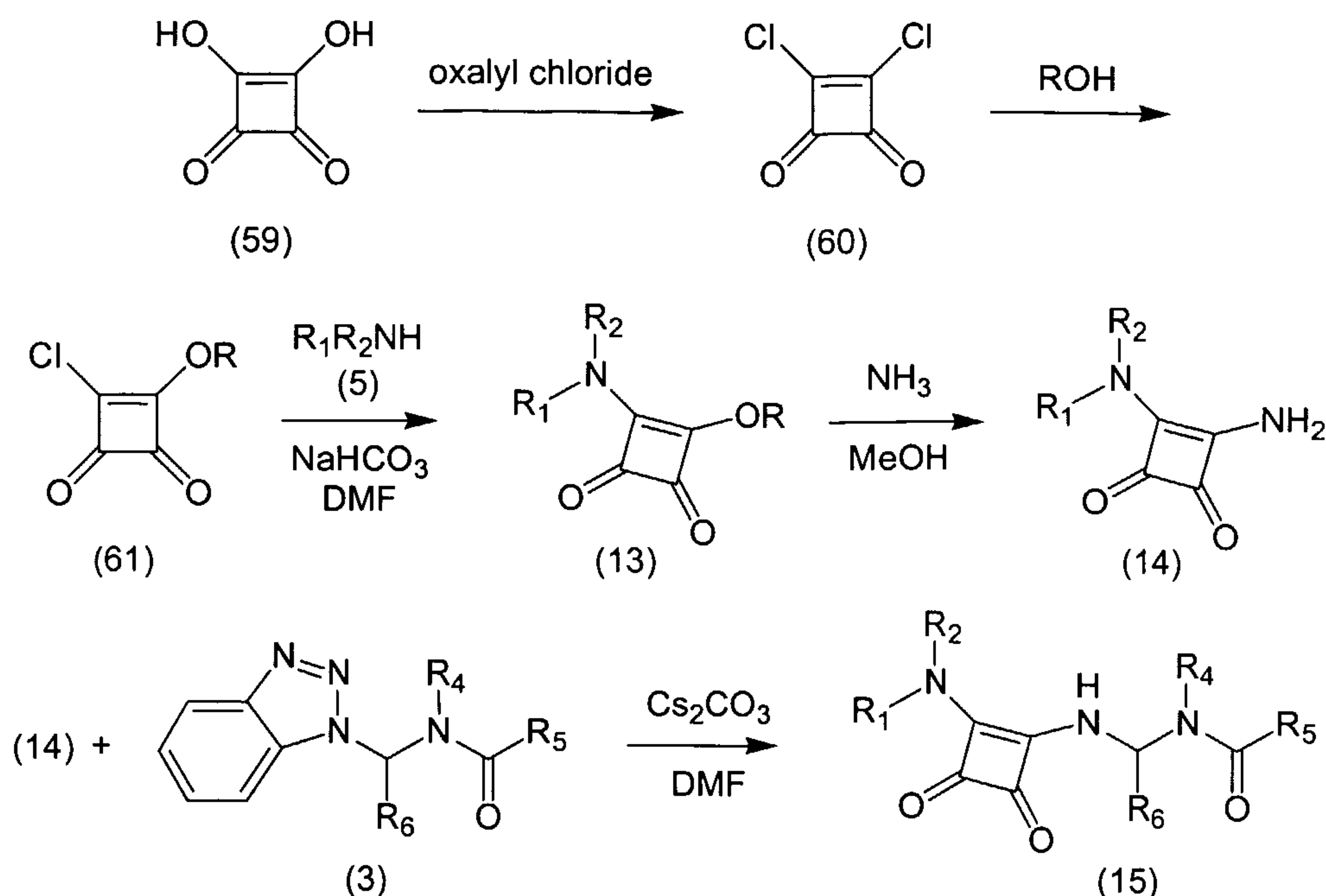
Scheme 16
