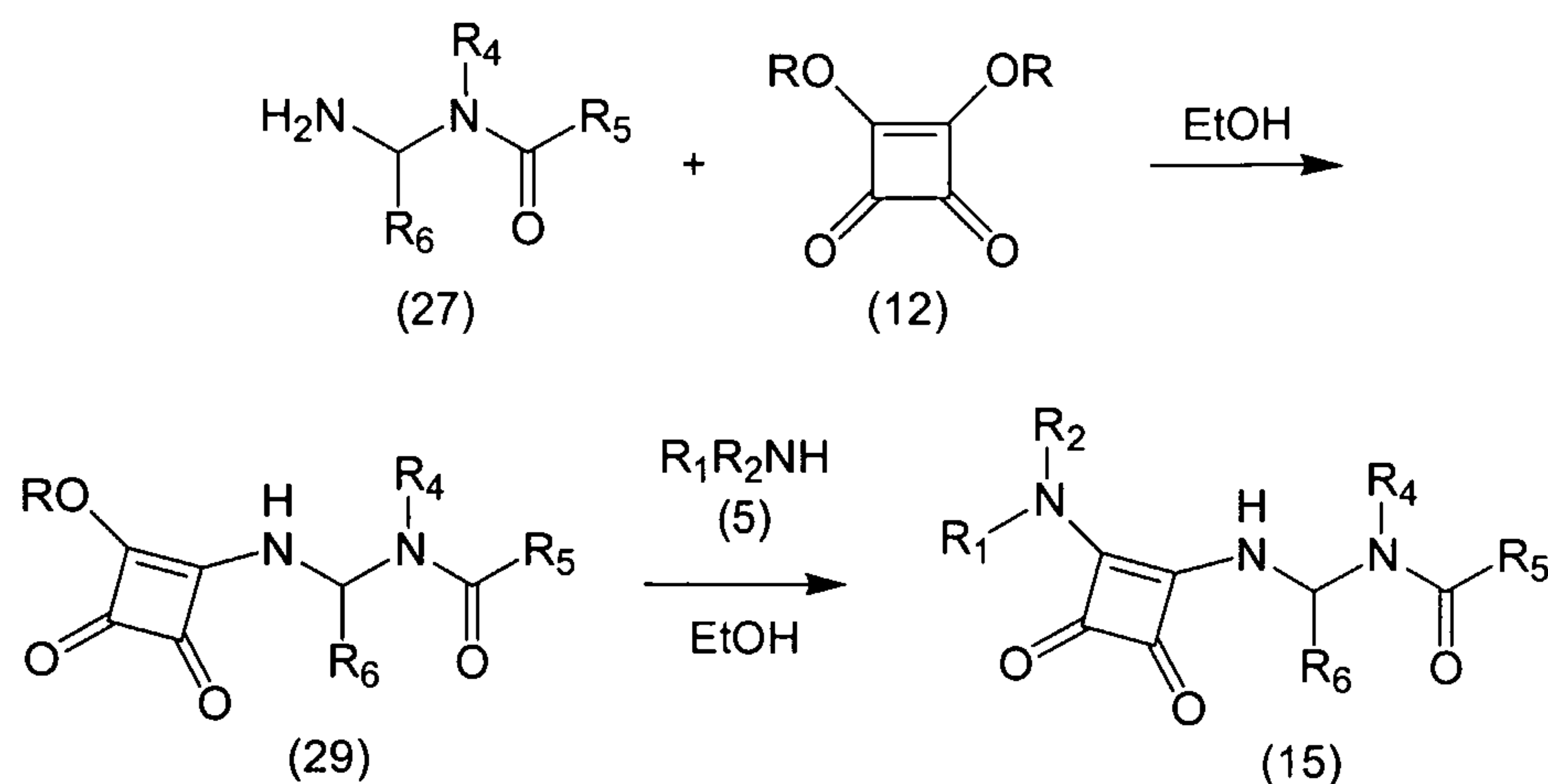
Scheme 7
