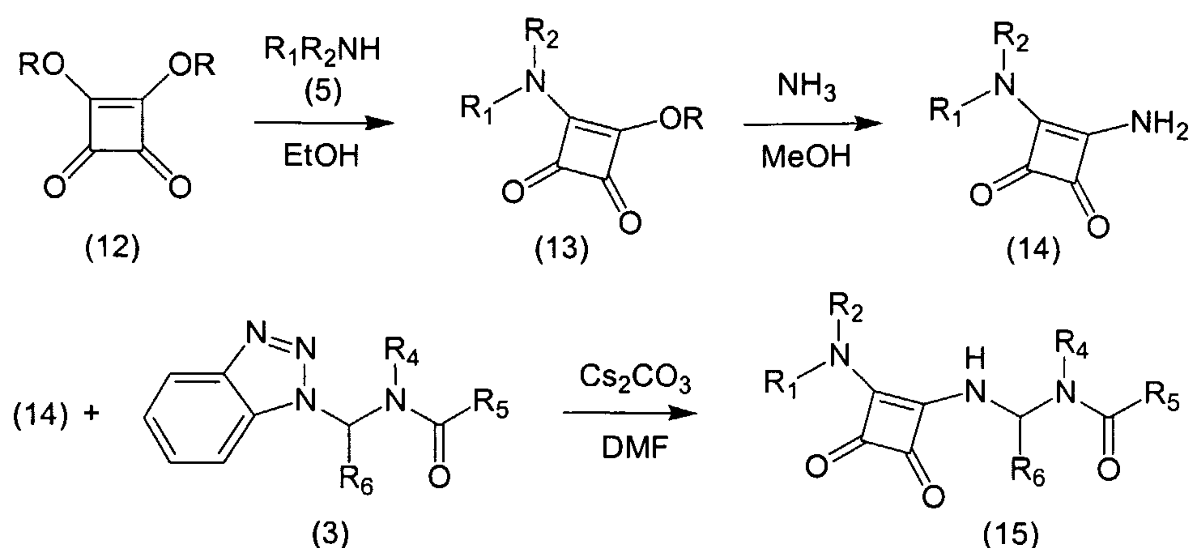
Scheme 2
