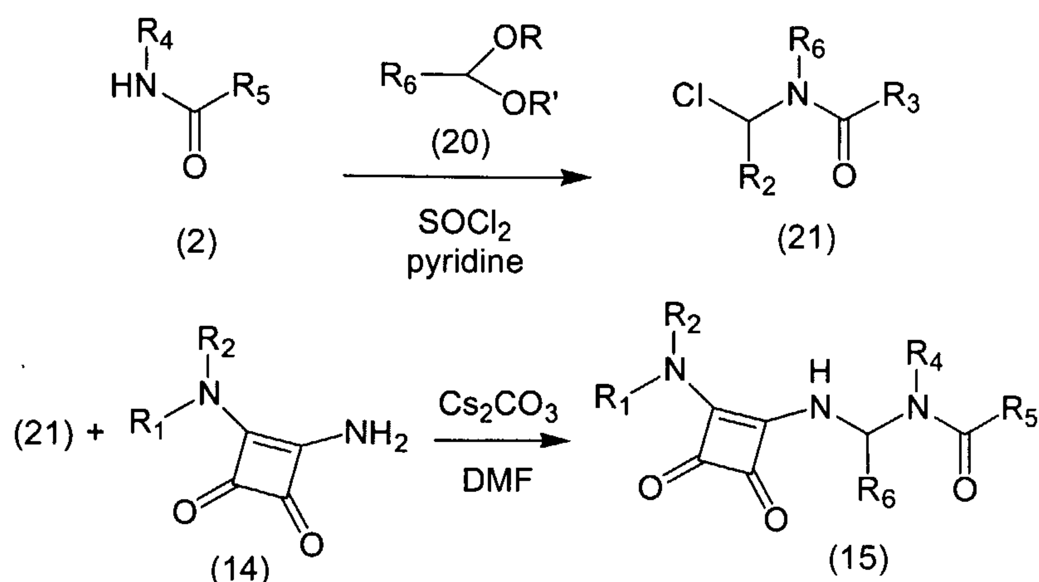
Scheme 4
