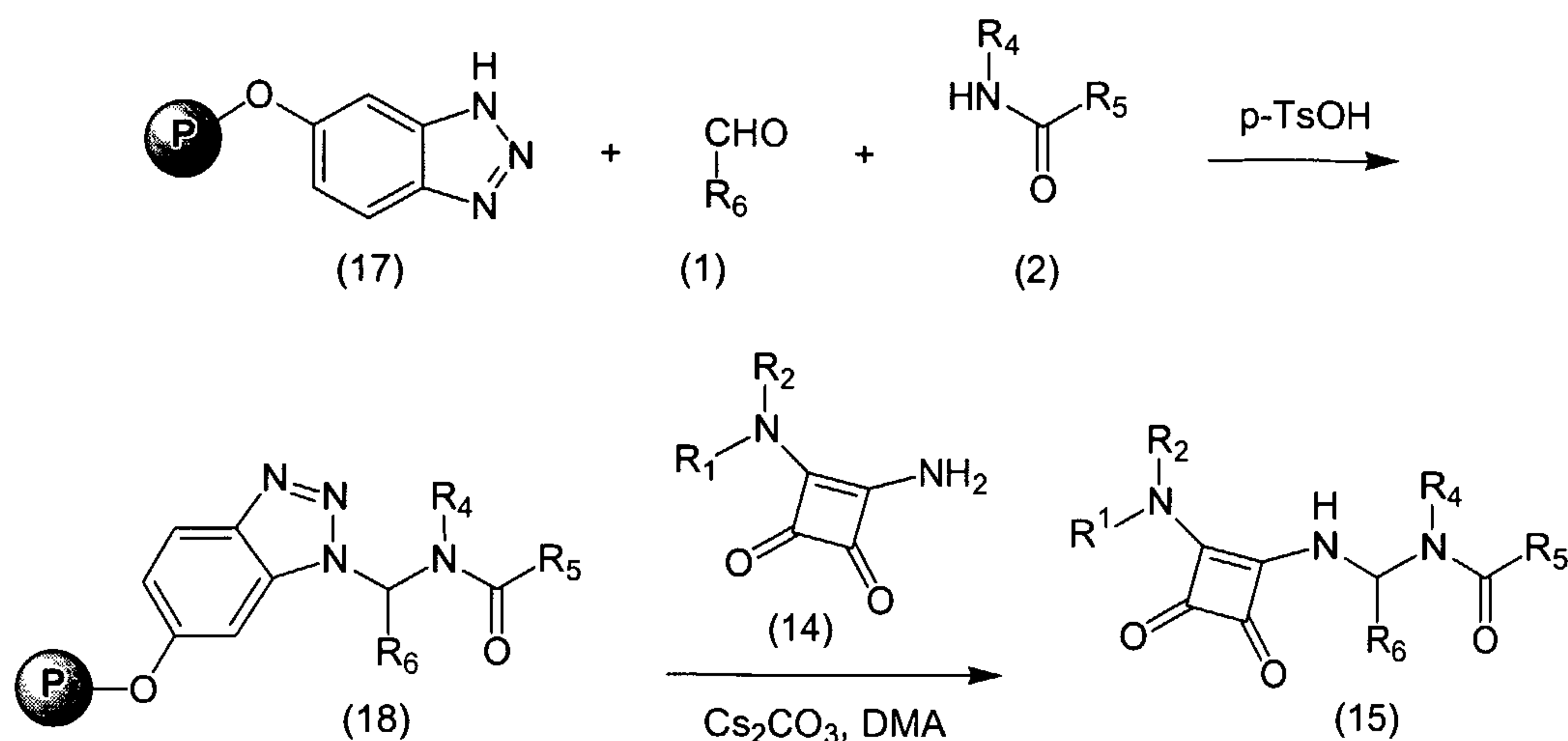
Scheme 3
