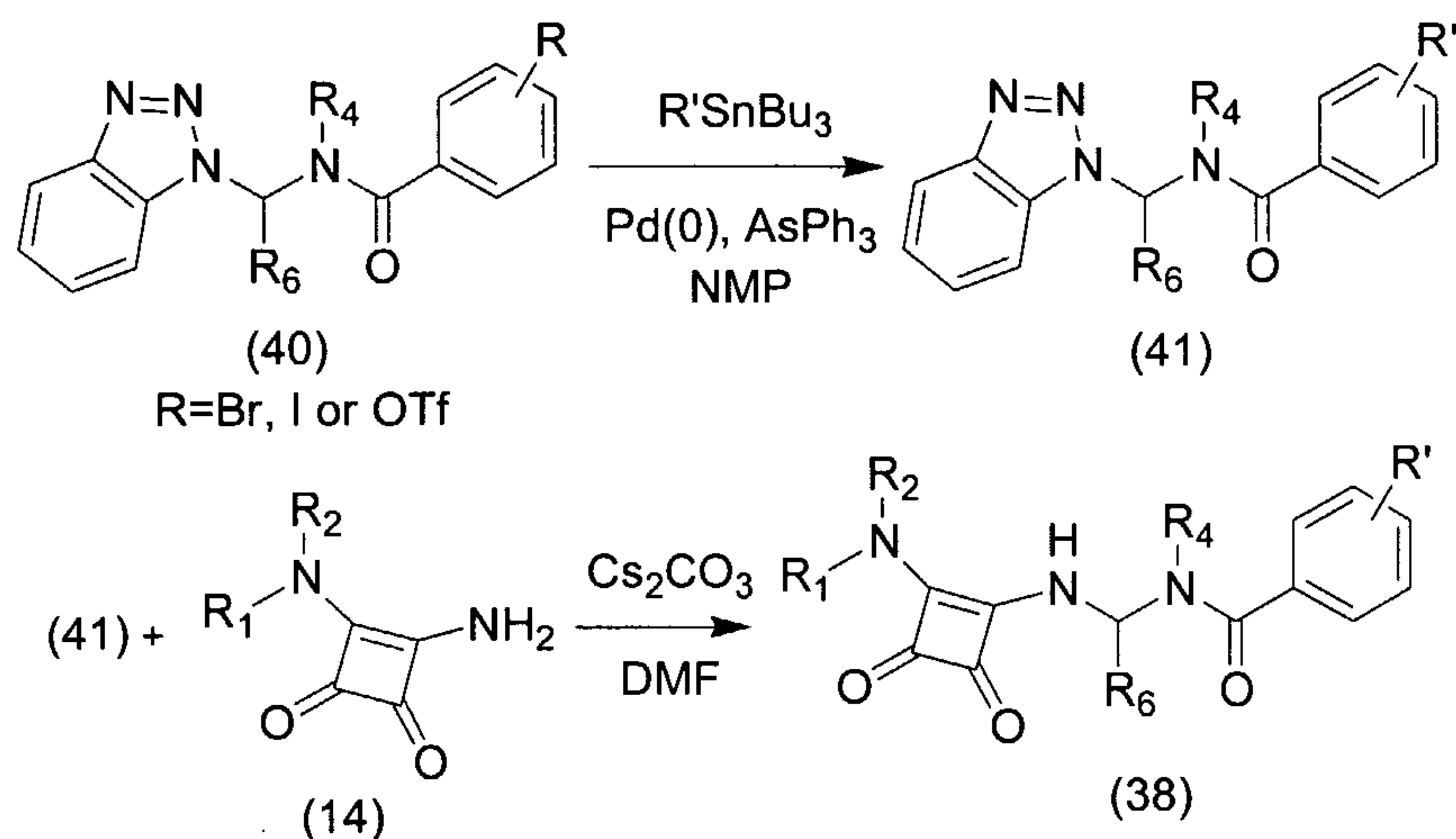
Scheme 11
