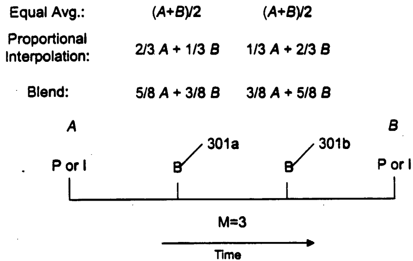
FIG. 3 Blended Pixel Value Weighting
