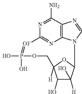
Fludarabine phosphate
