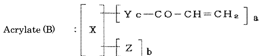
Structural Formula (2)
