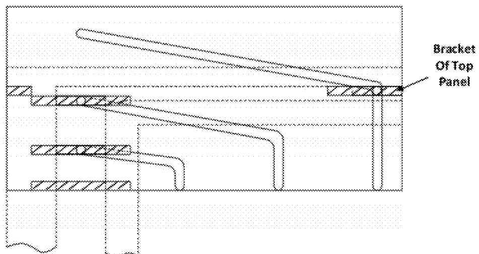
FIG. 6B Top Panel Partially Deployed
