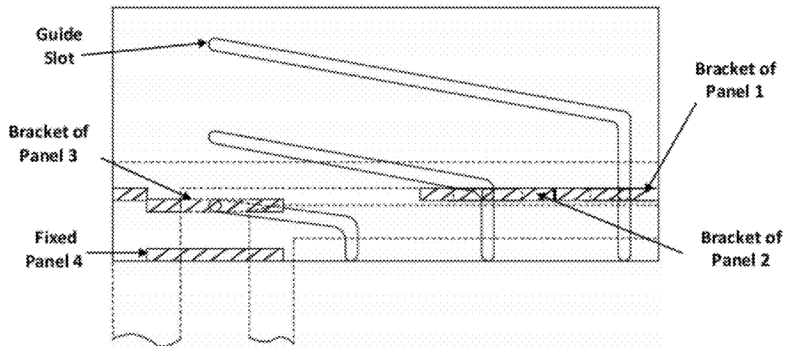
FIG. 6C Top and Second Panels Partially Deployed
