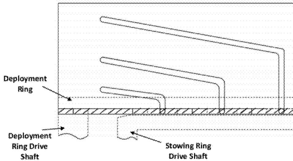
FIG. 6D Fully Deployed Configuration
