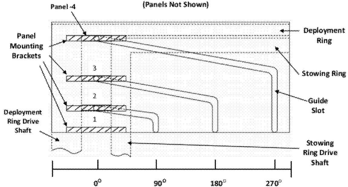
Fig. 6A Deployment Mast Wall Flattened Stowed Configuration (Panels Not Shown)
