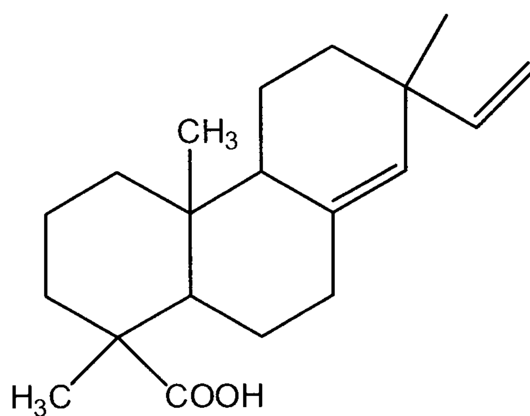
Sandaracopimaric Acid
