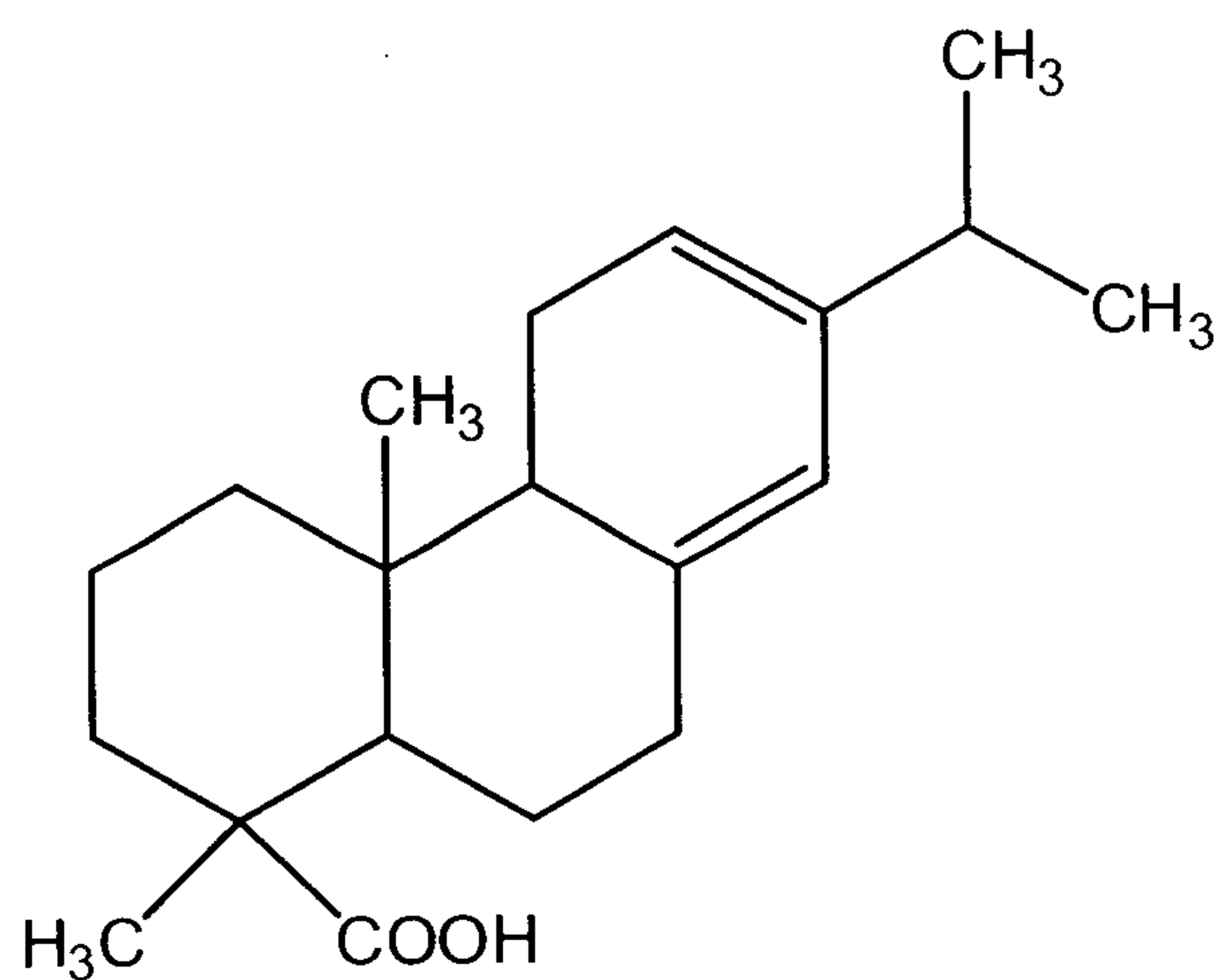
Levo-Pimaric Acid
