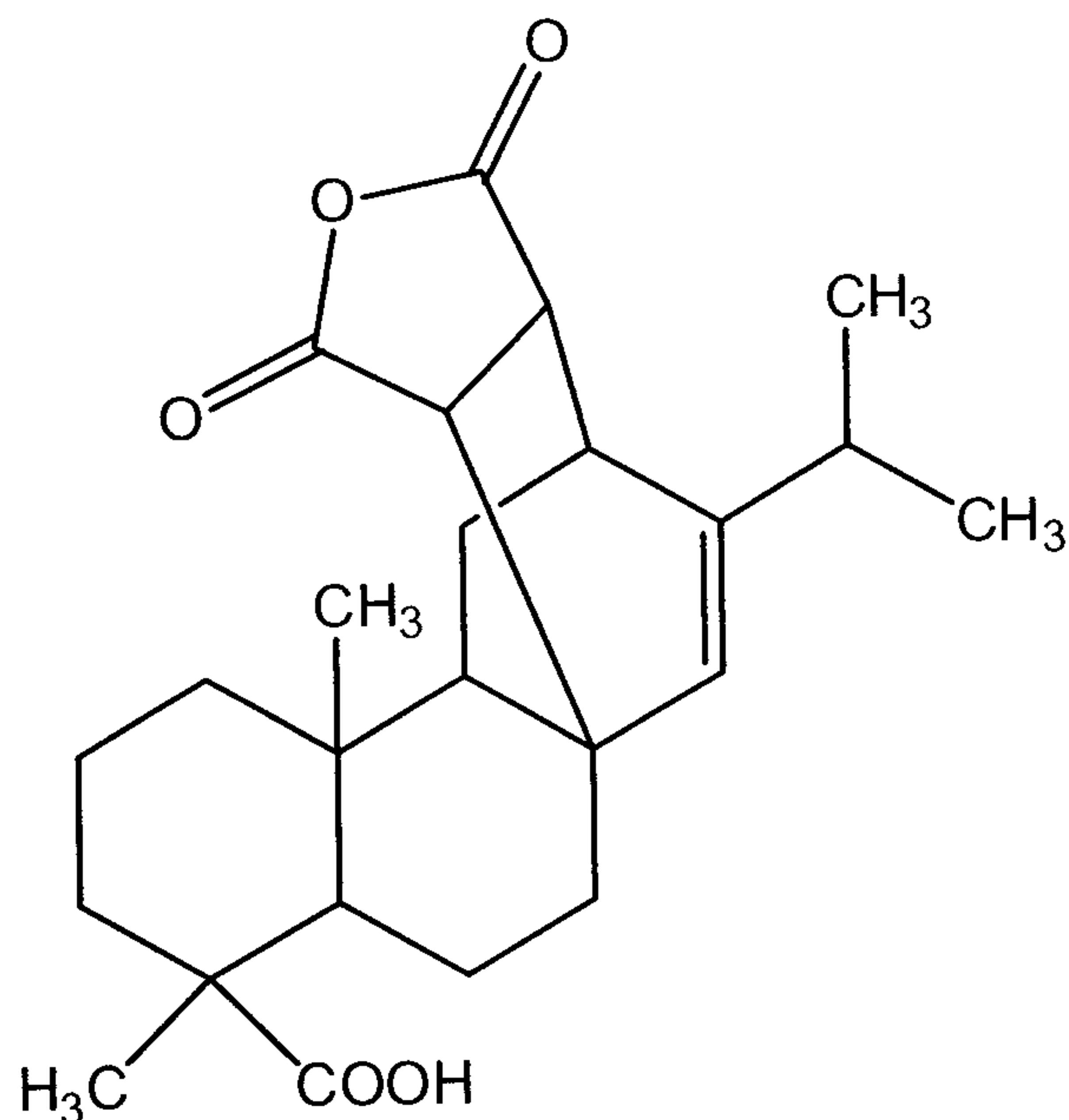
Maleic Anhydride-Modified Abietic Acid
