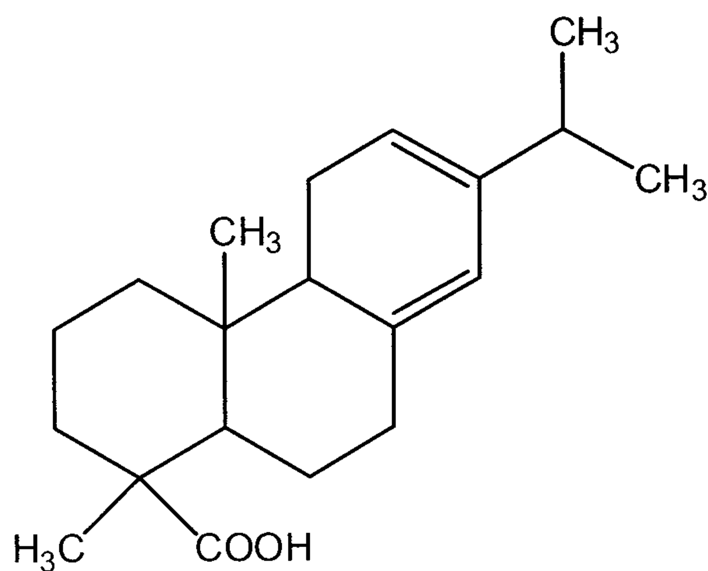
Dehydroabietic Acid
