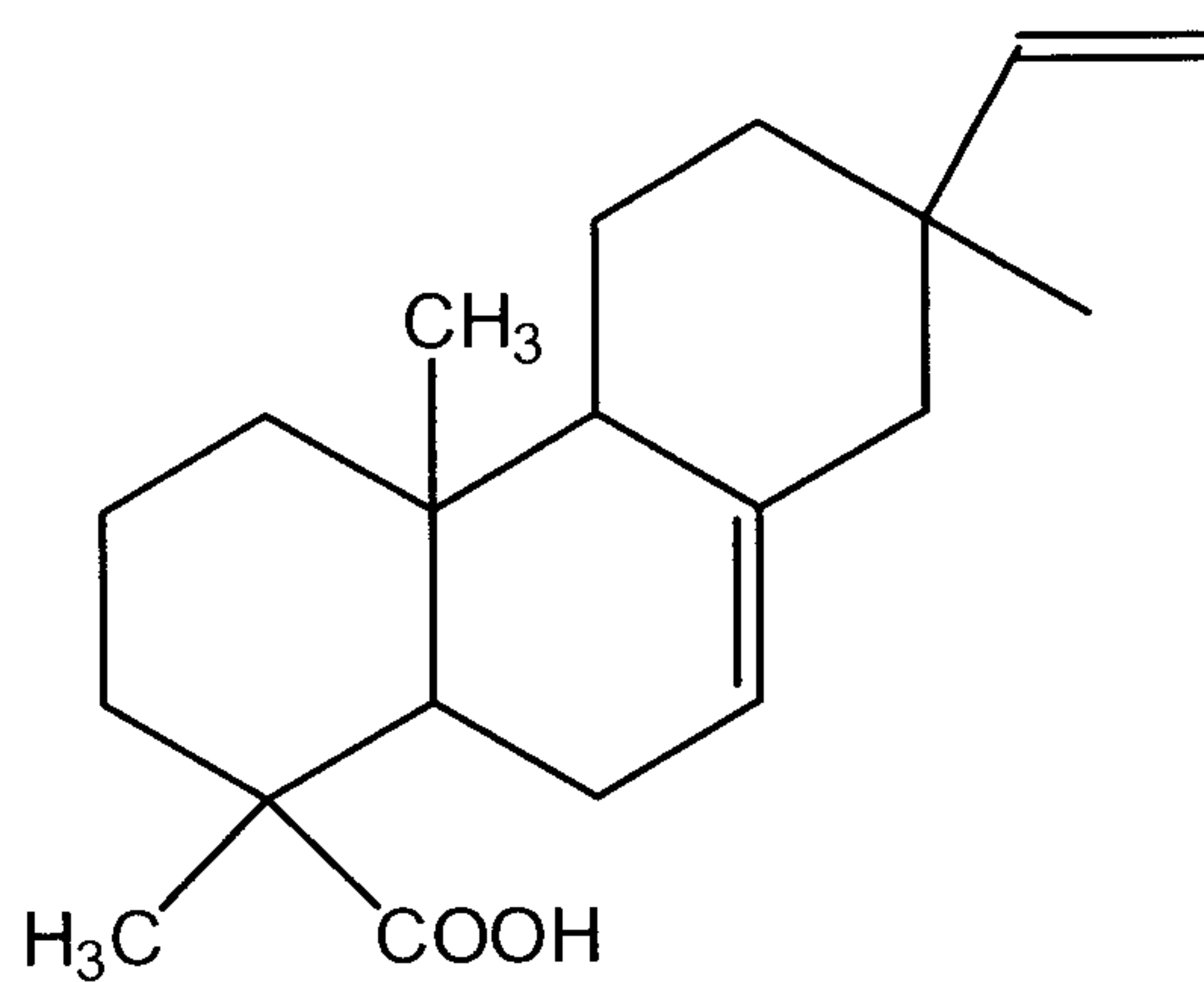
Isopimaric Acid
