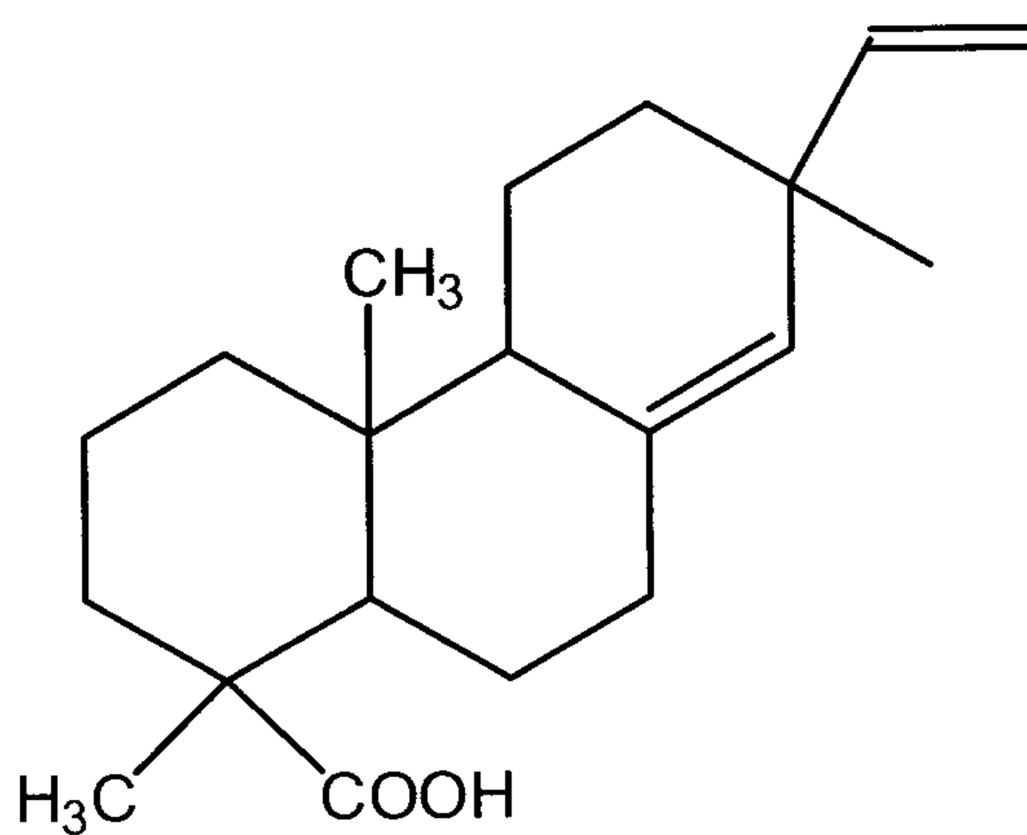
Pimaric Acid
