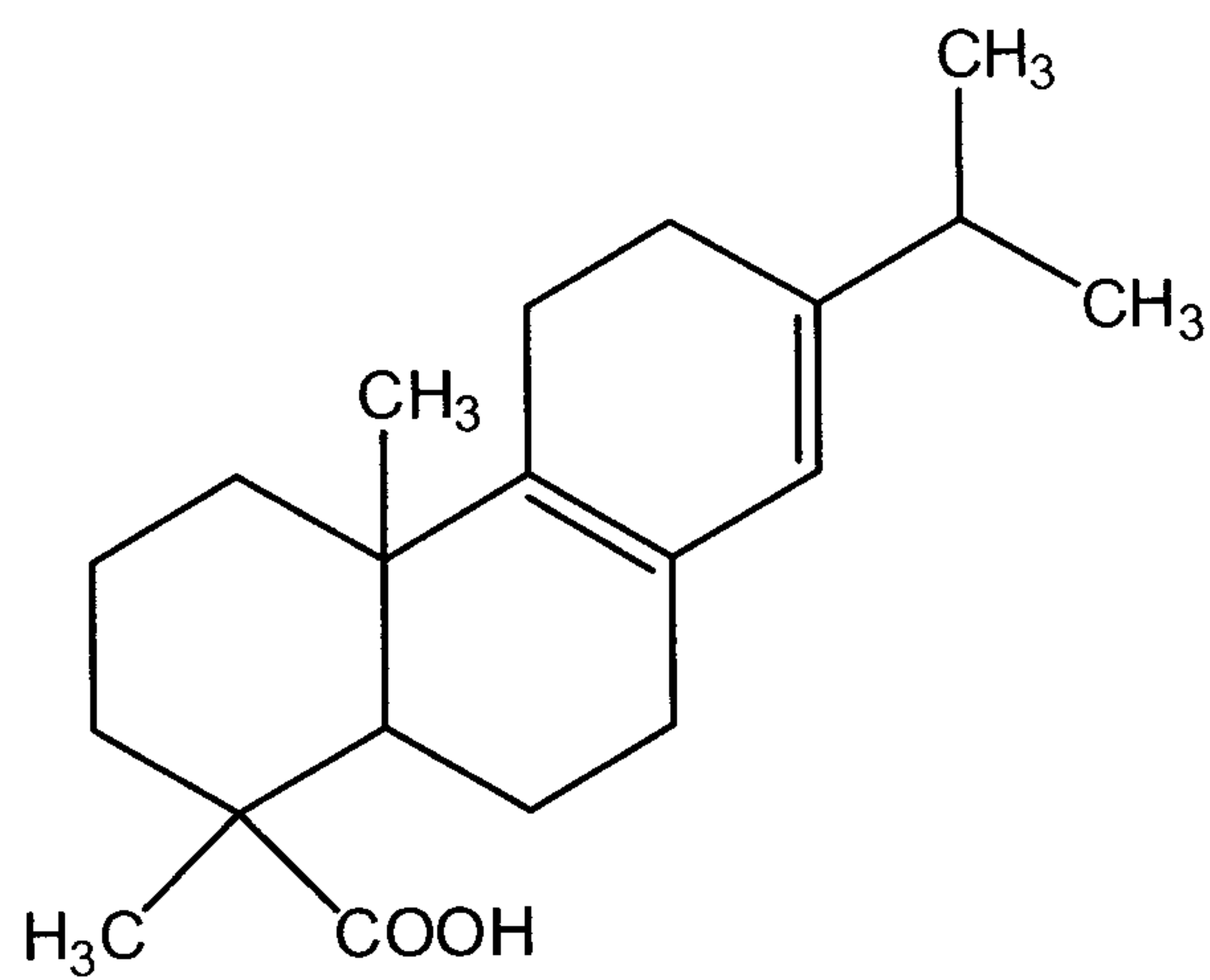
Palustric Acid
