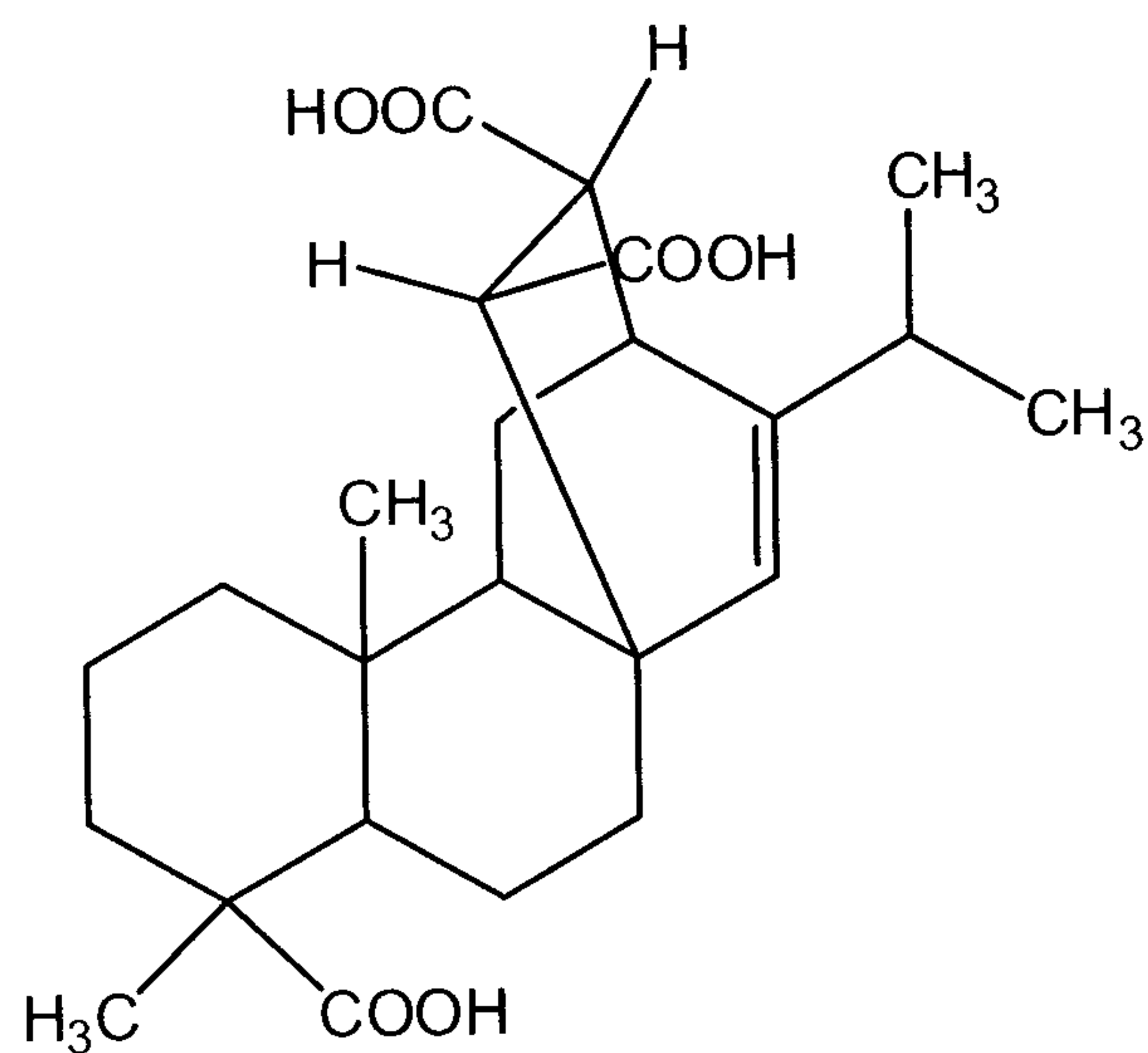
Fumaric Acid-Modified Abietic Acid
