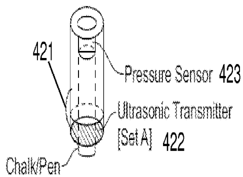
Chalk/Pen Holder 420
