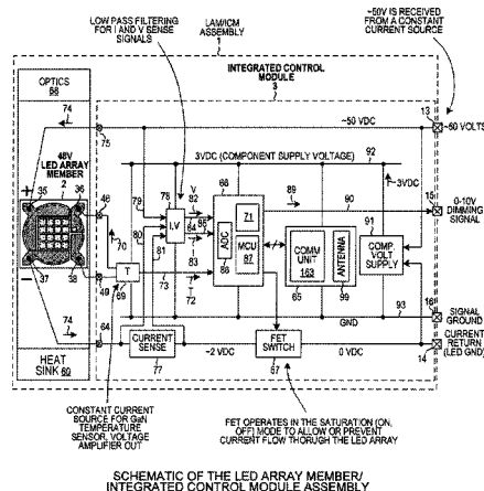
SCHEMATIC OF THE LED ARRAY MEMBER/ INTEGRATED CONTROL MODULE ASSEMBLY
