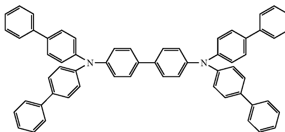
4,4'-bis[N-(4-biphenyl)-N-(4-biphenyl)amino]biphenyl
