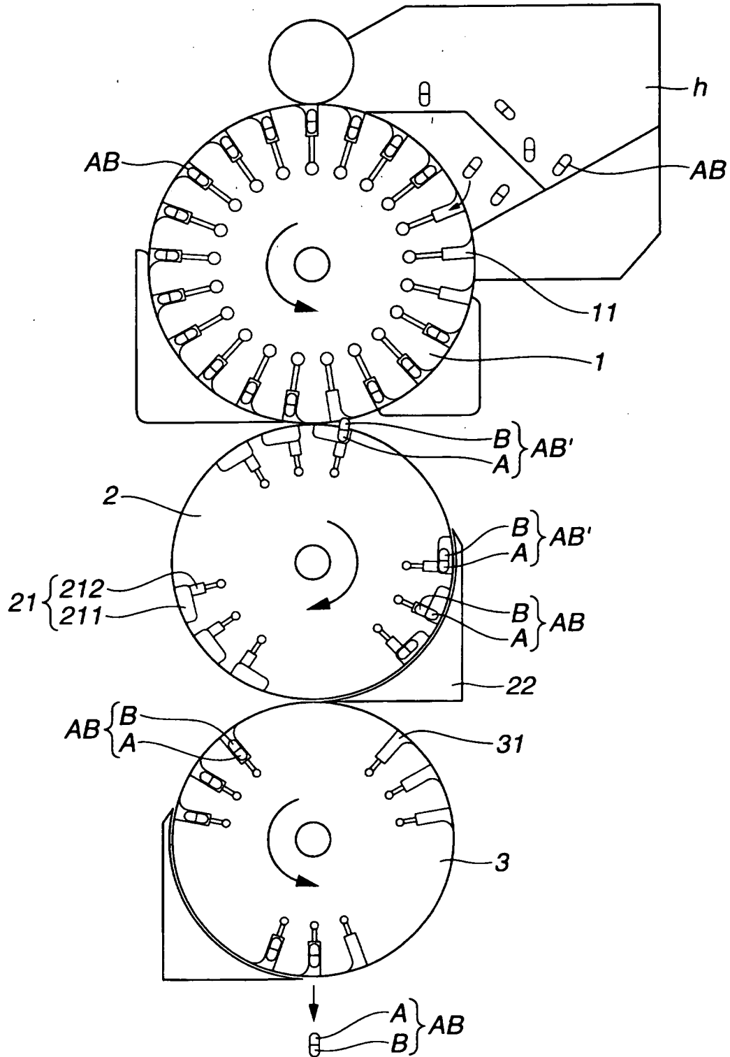
FIG.13 (PRIOR ART)
