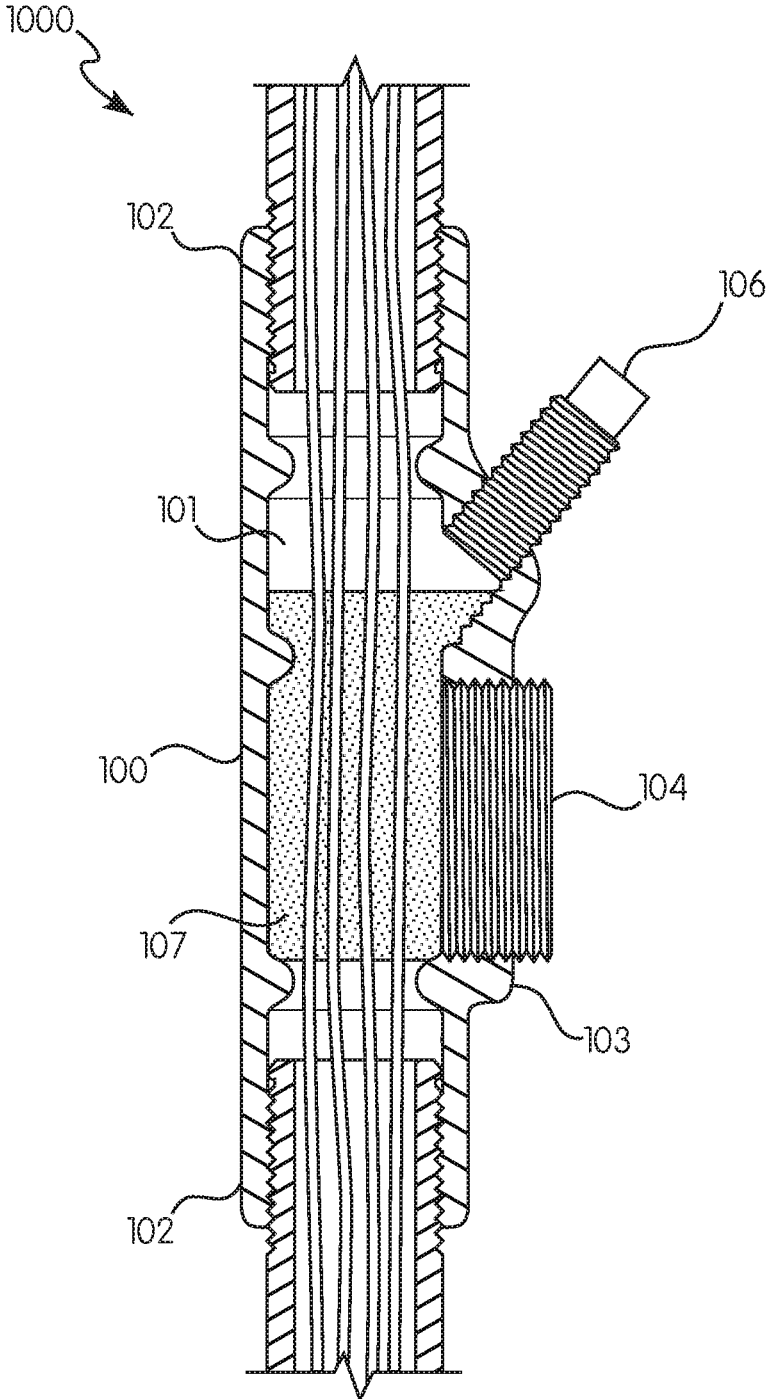
FIG. 3 (Prior Art)
