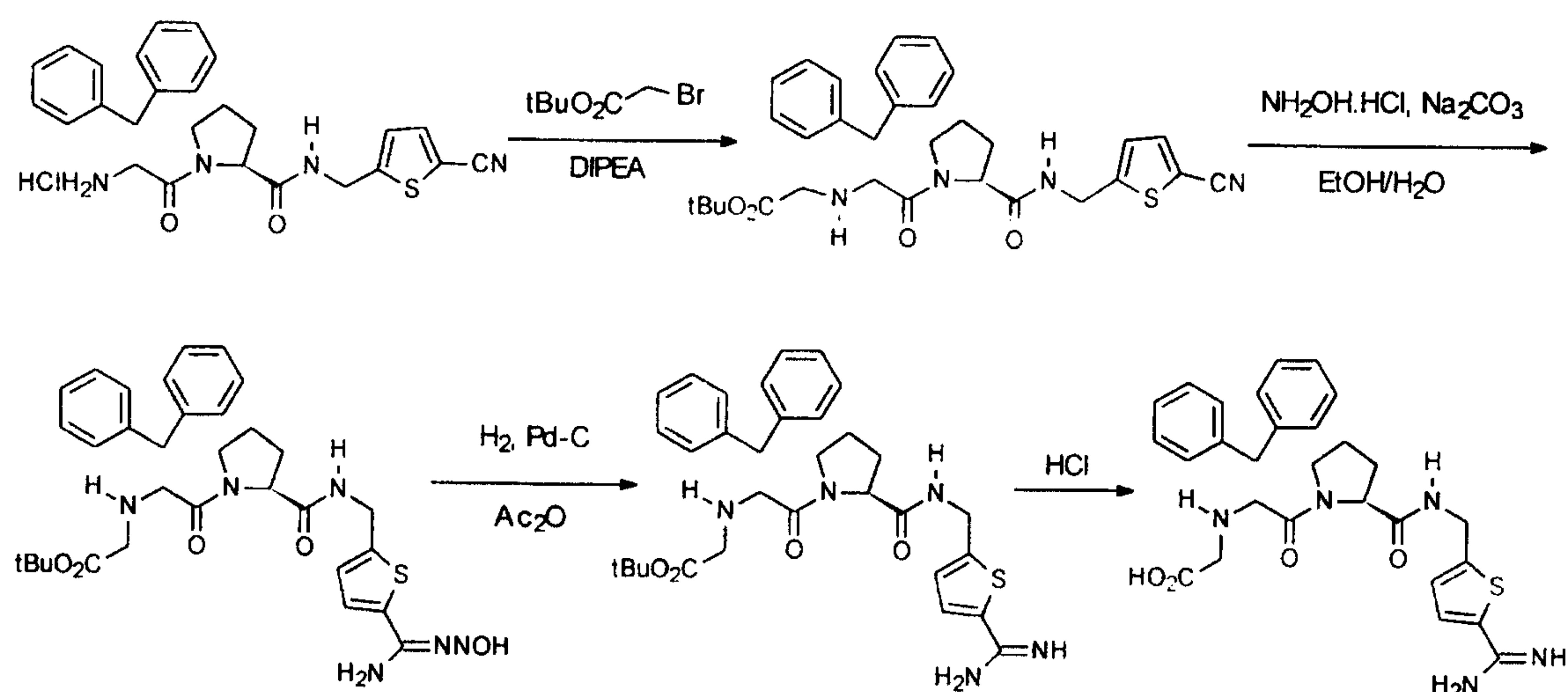
Scheme 4
