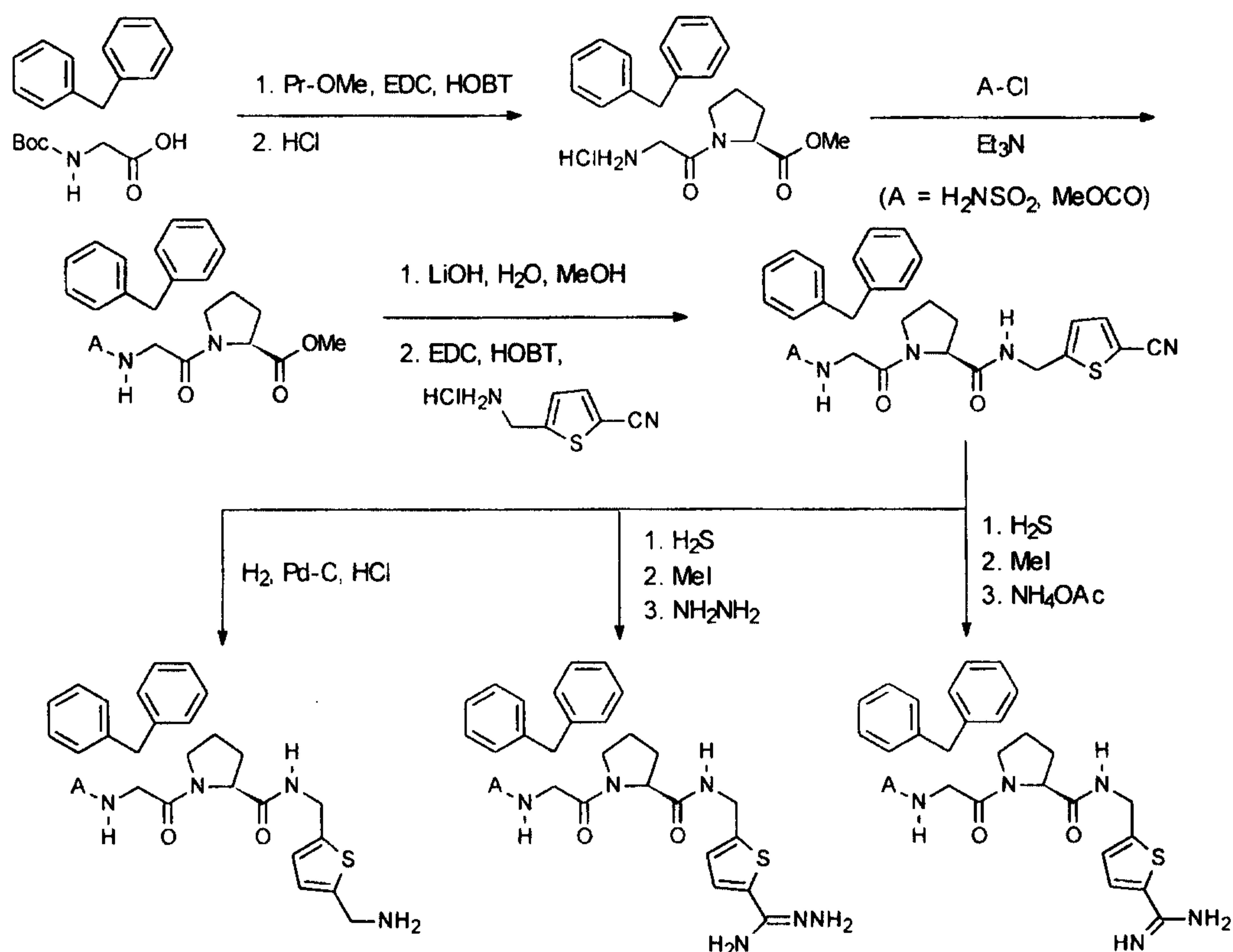
Scheme 1
