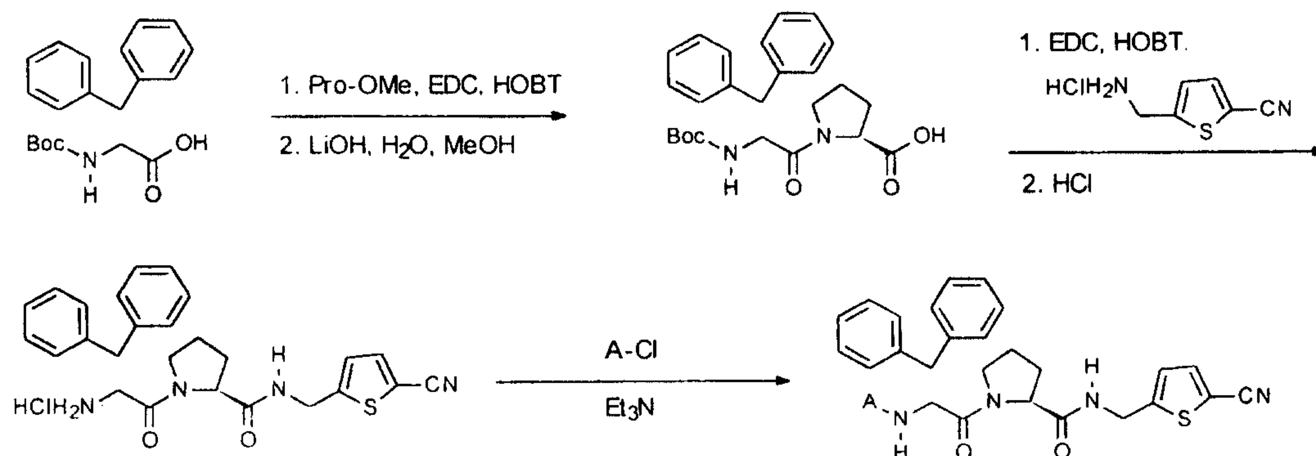
Scheme 2
