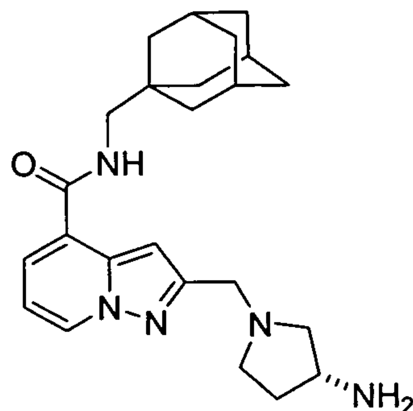
Compound 4
