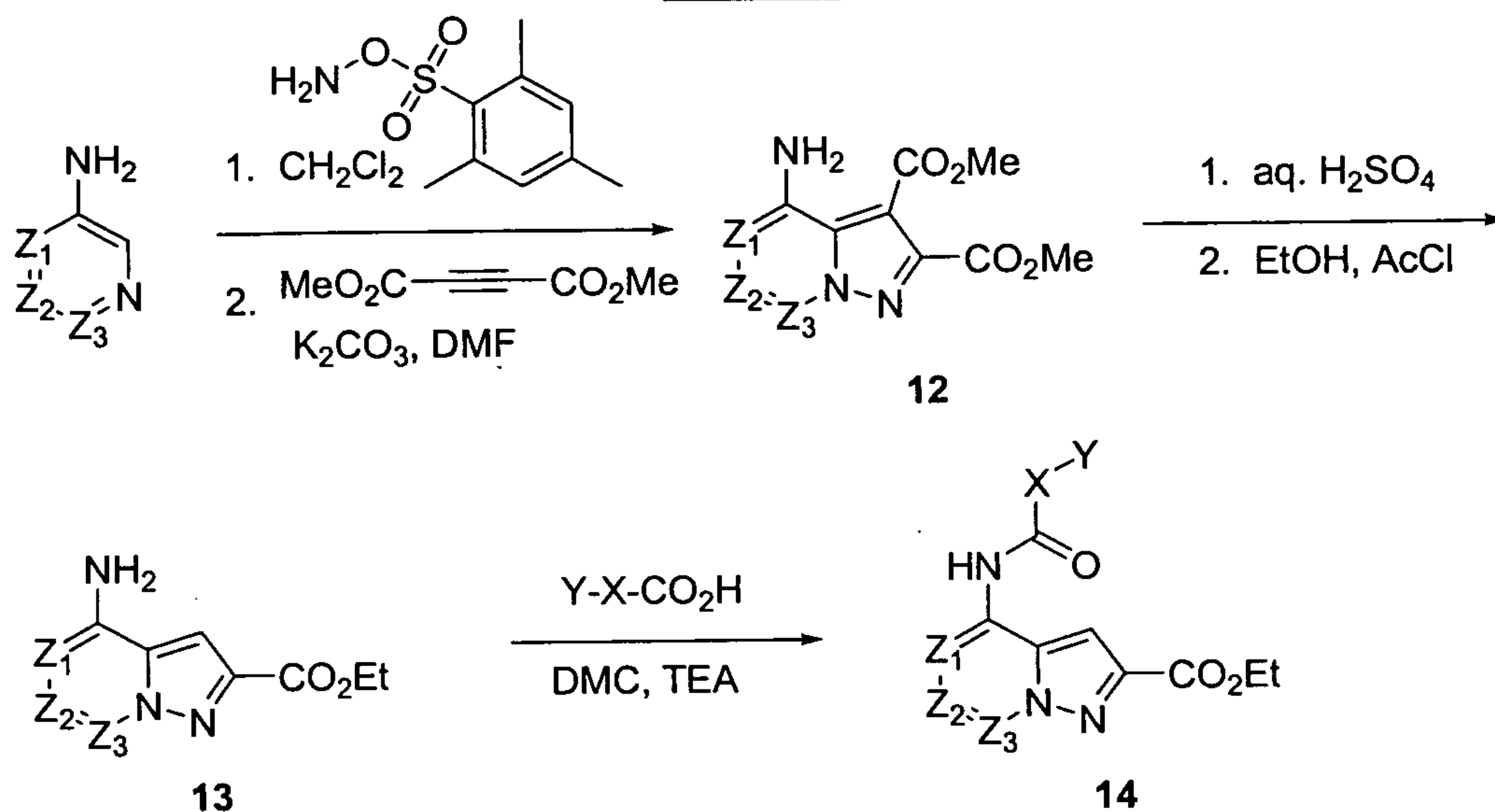
Scheme V
