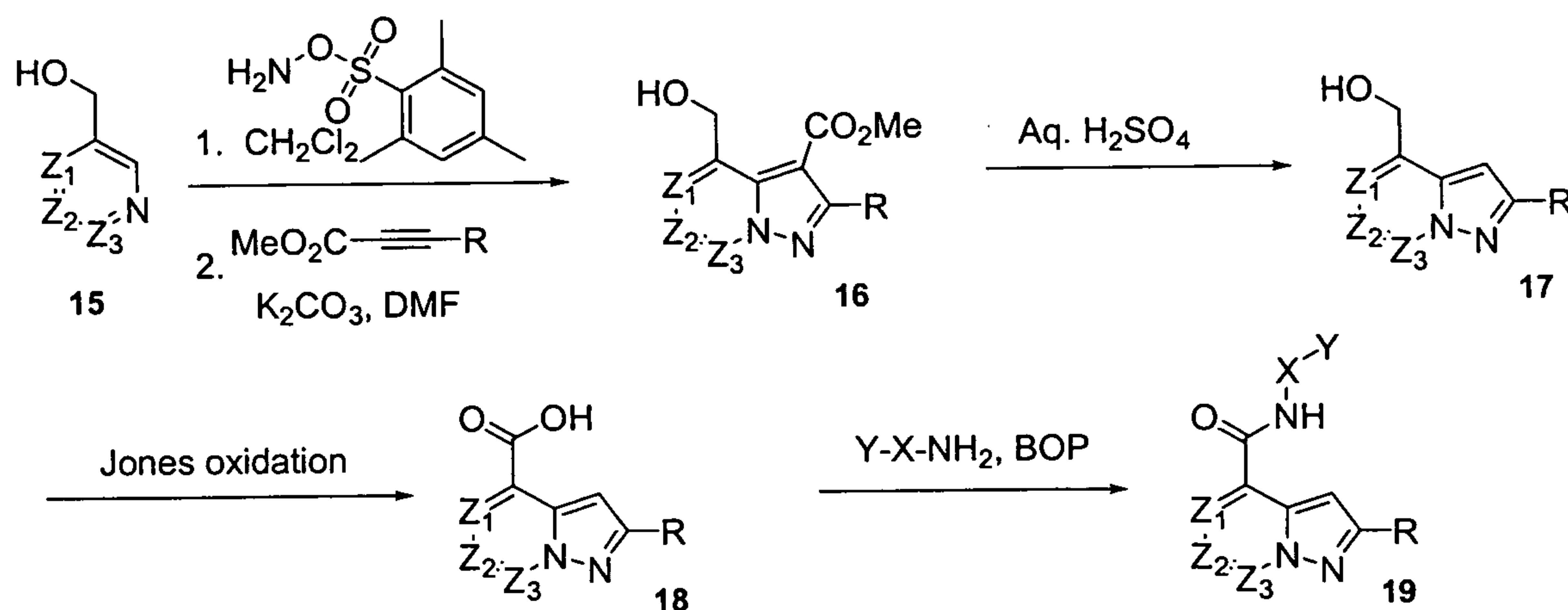
Scheme VII
