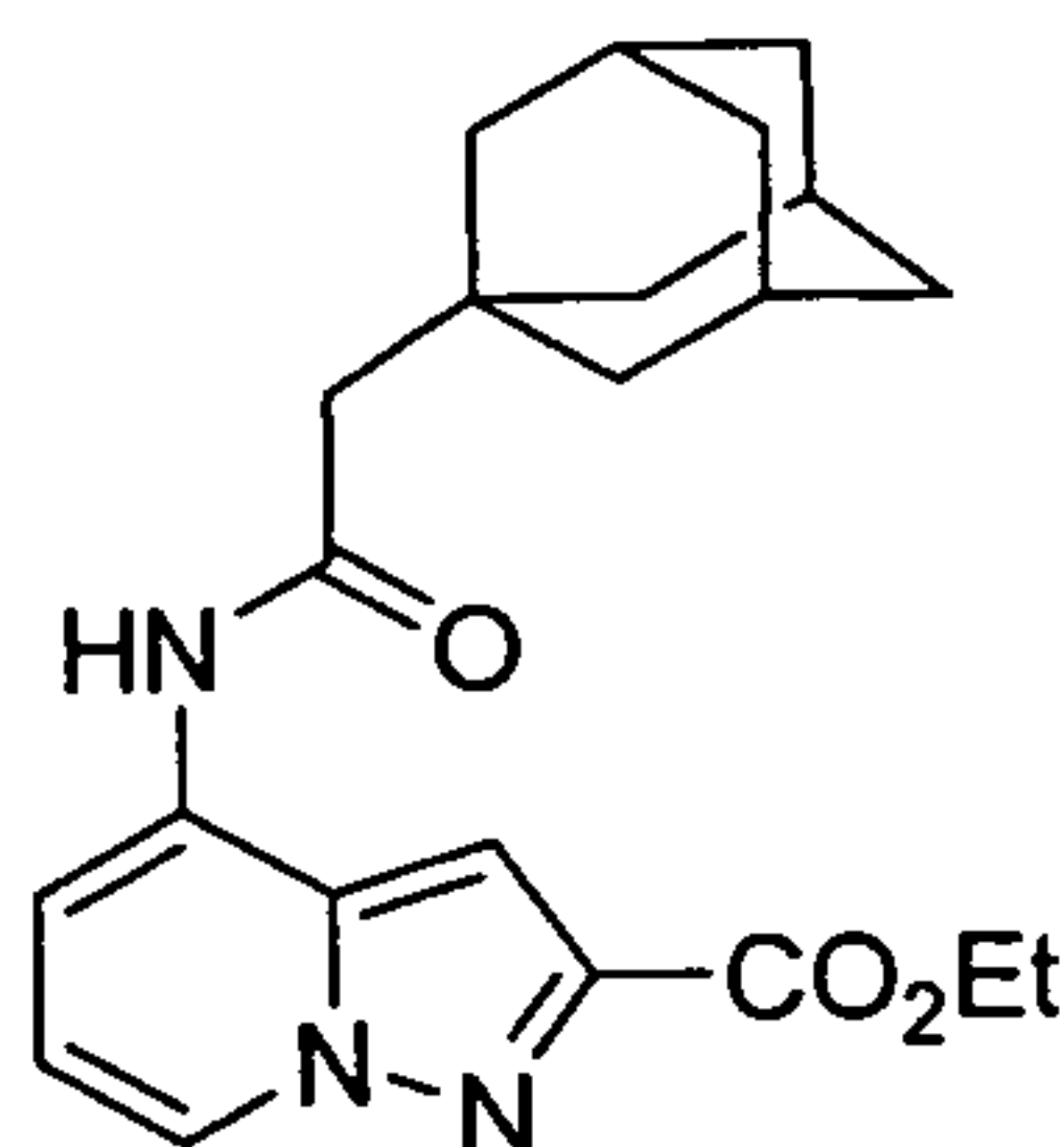
Compound 10
