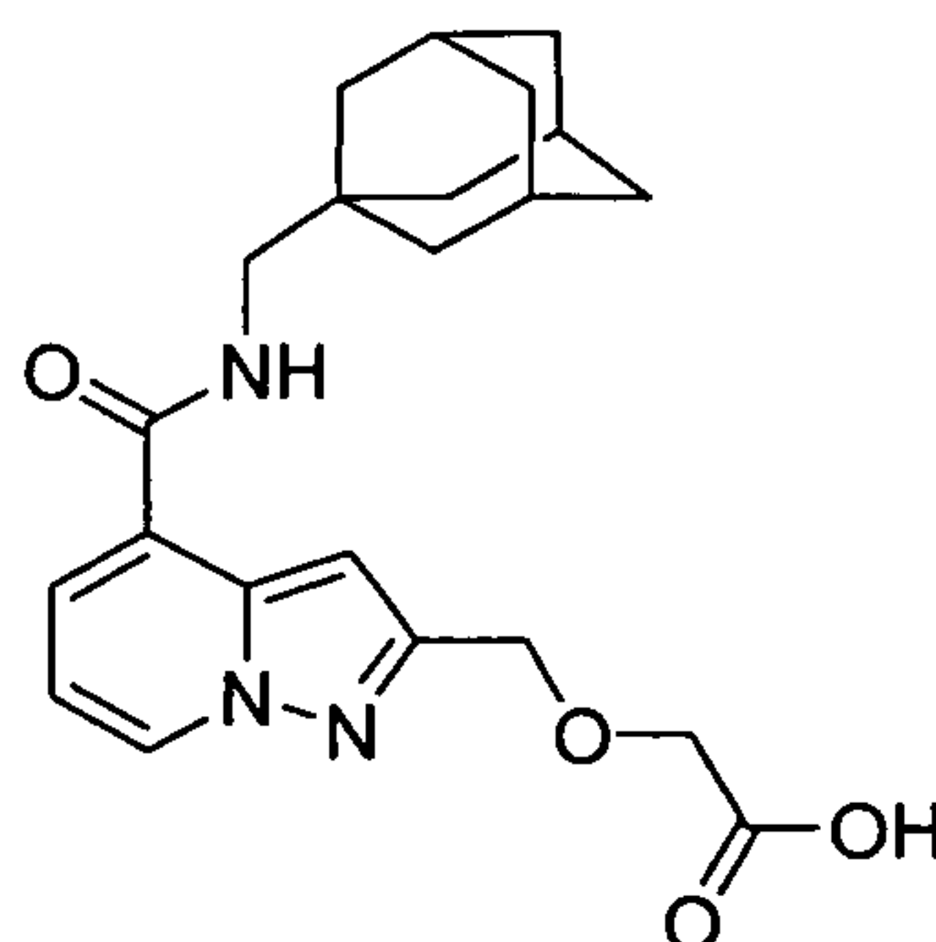
Compound 9
