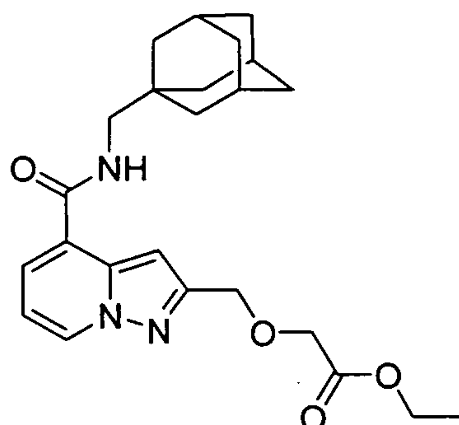
Compound 8
