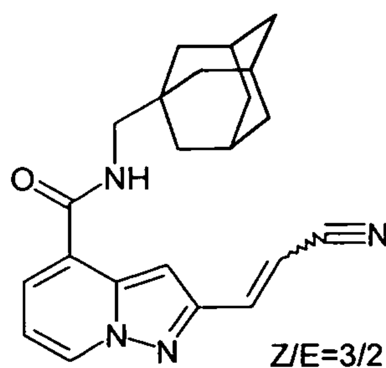
Compound 11
