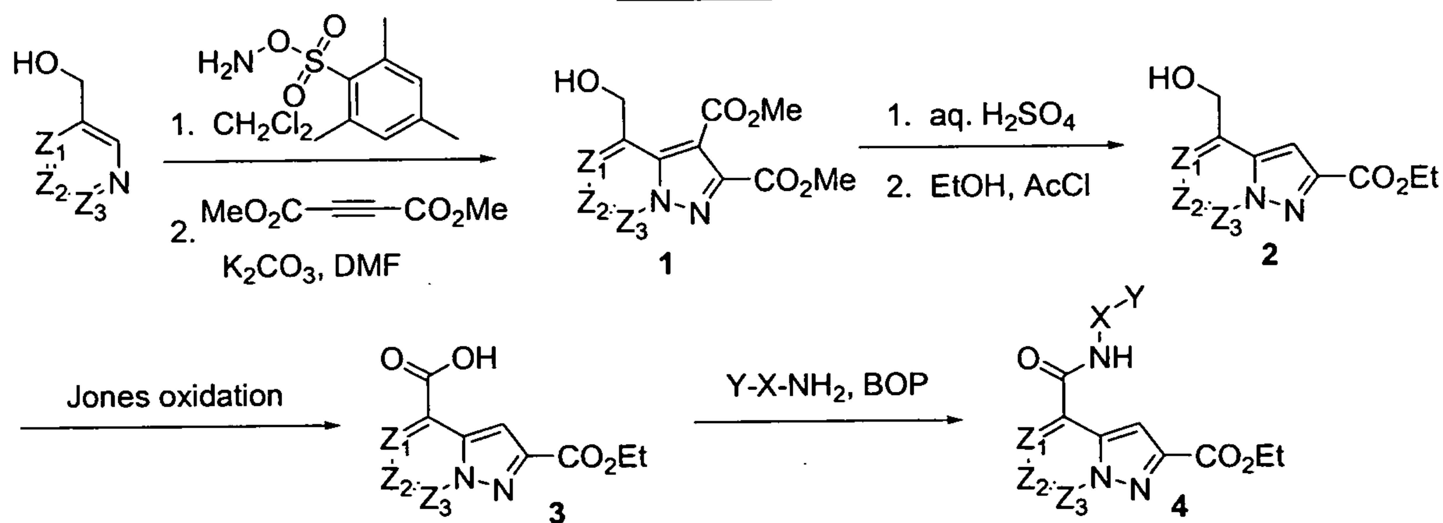
Scheme 1
