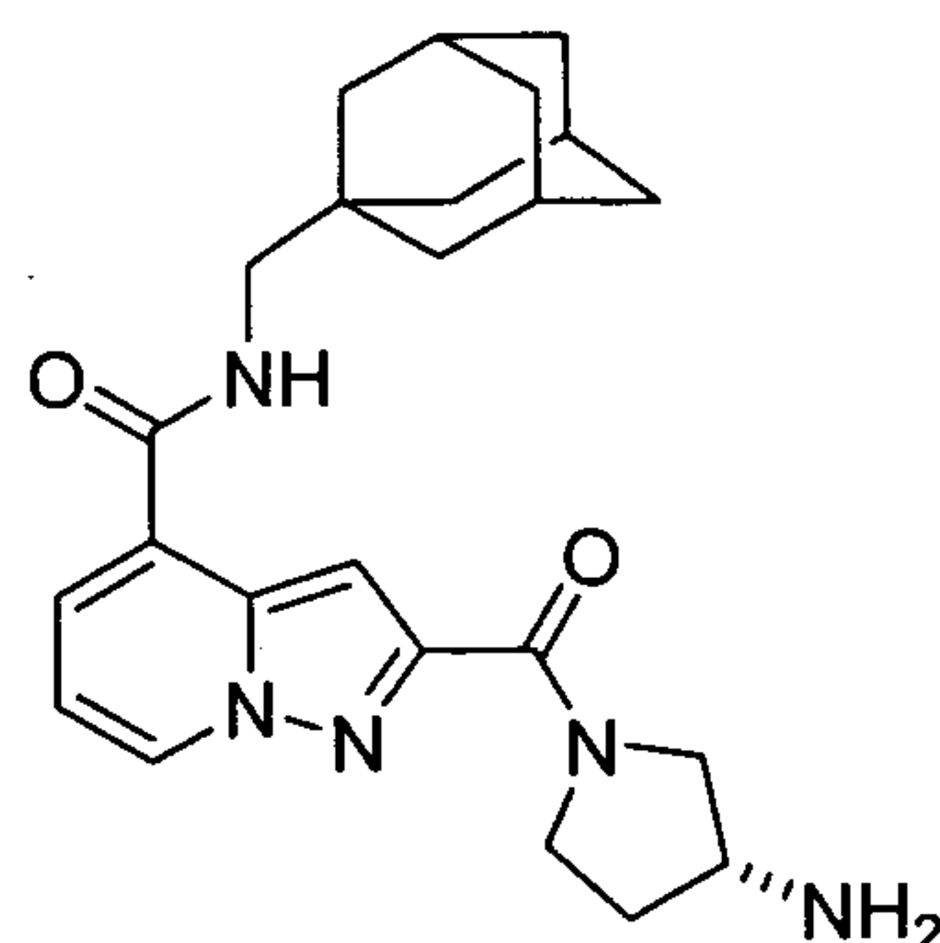
Compound 2
