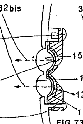
FIG.73-B SECTION A-A
