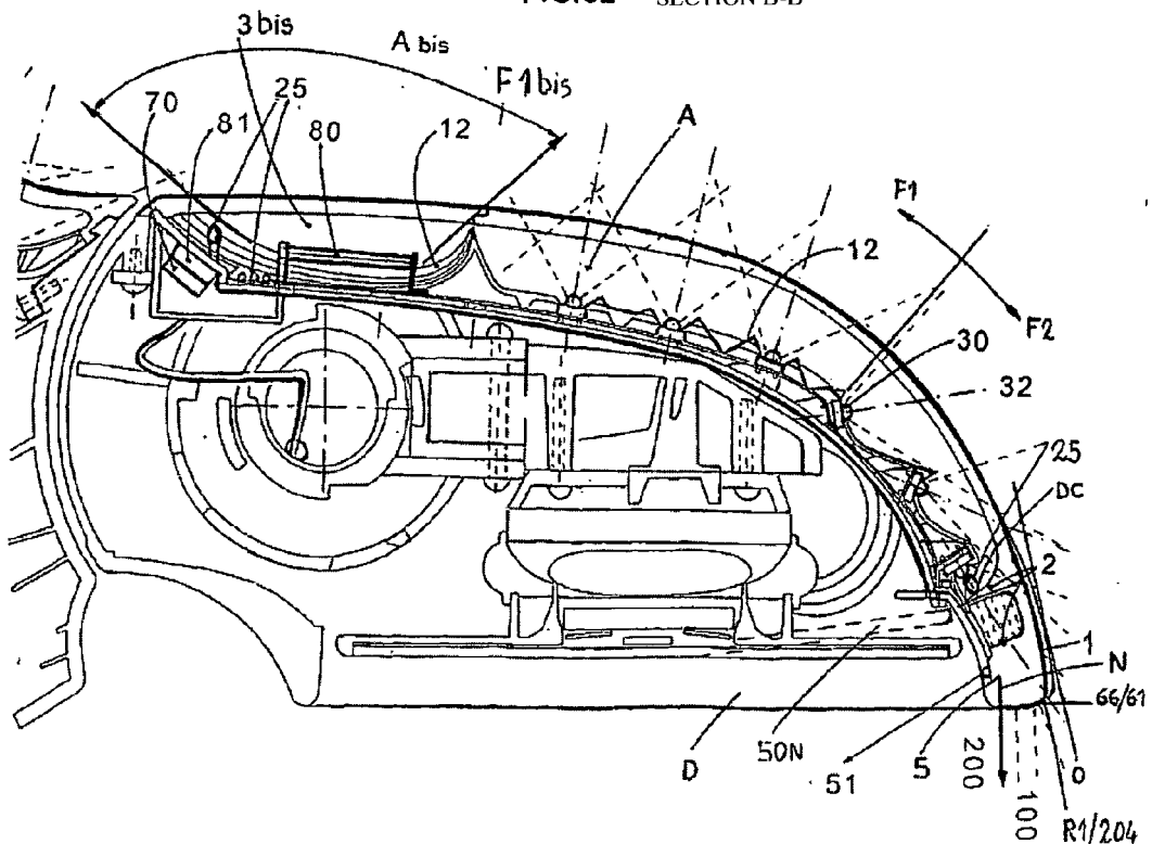
FIG.52 SECTION B-B
