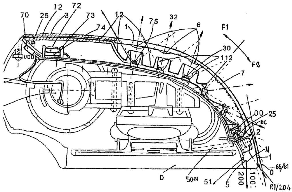
FIG.52 SECTION B-B
