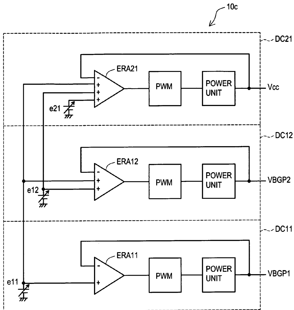
FIG. 13 CIRCUIT DIAGRAM OF POWER SUPPLY 10c
