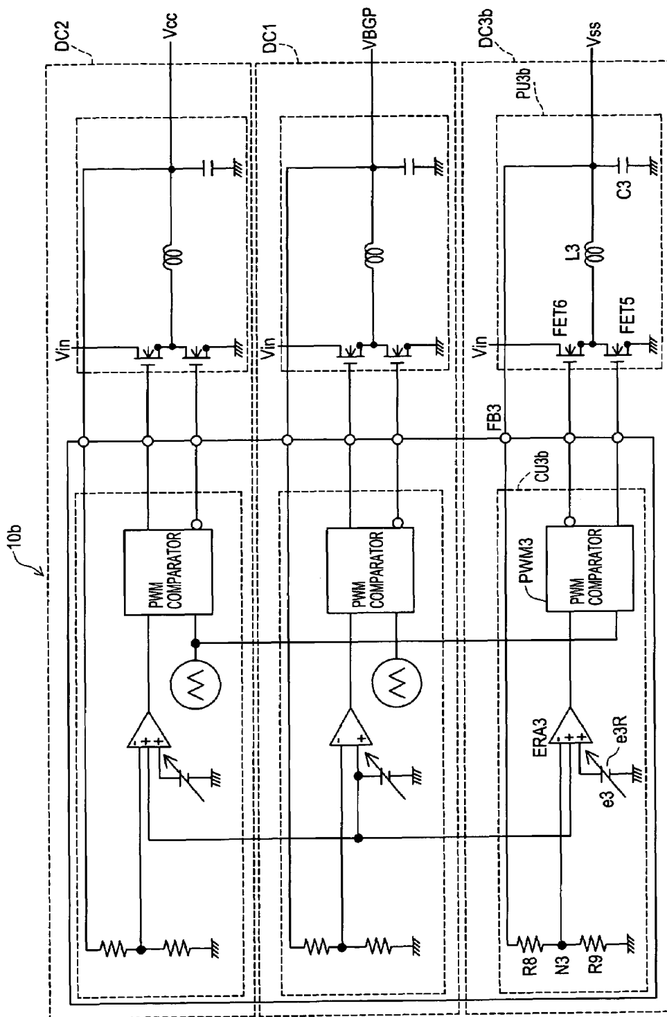
FIG. 11 CIRCUIT DIAGRAM OF POWER SUPPLY 10b
