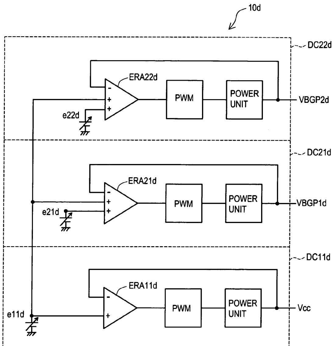
FIG. 14 CIRCUIT DIAGRAM OF POWER SUPPLY 10d
